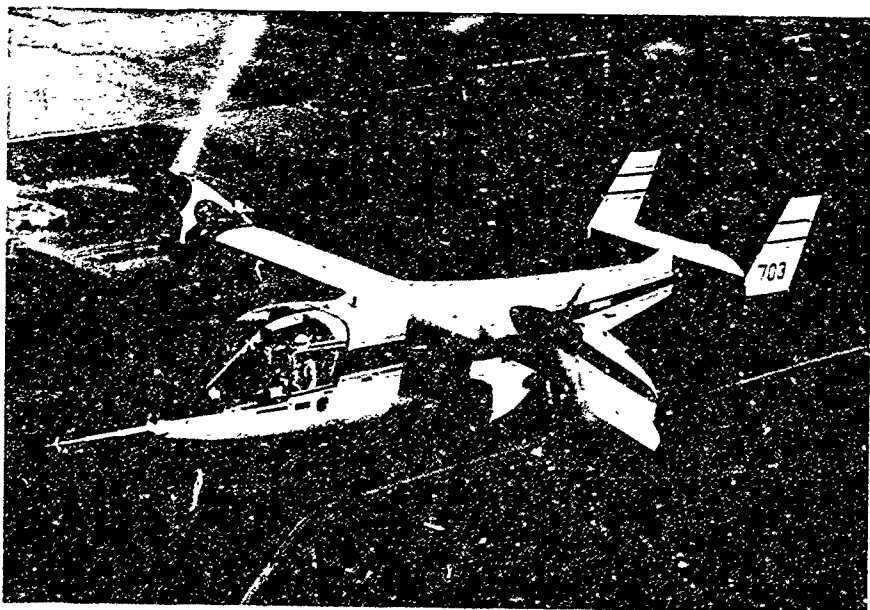
The XV-15 tilt rotor research aircraft For takeoff (above), the craft's rotors are horizontal to provide lift, then they pivot forward (bottom) to a full vertical position to give cruising speeds twice those of conventional helicopters.
