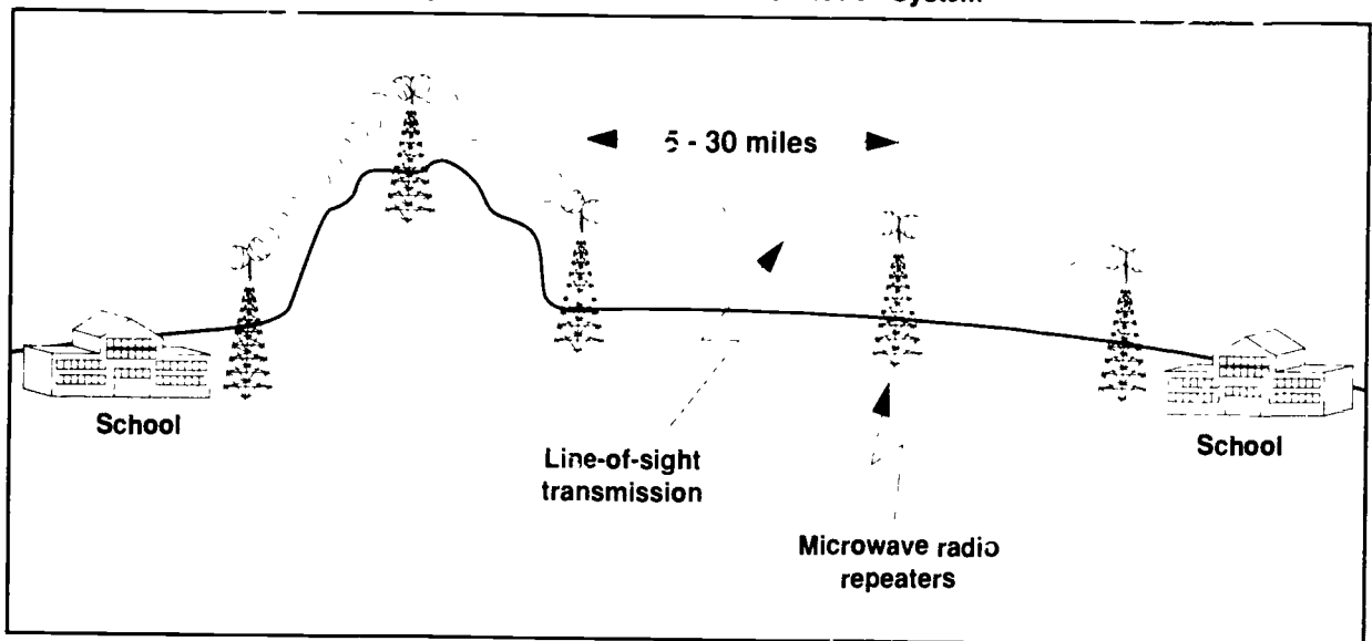
Figure 3-8—Microwave Communication System
