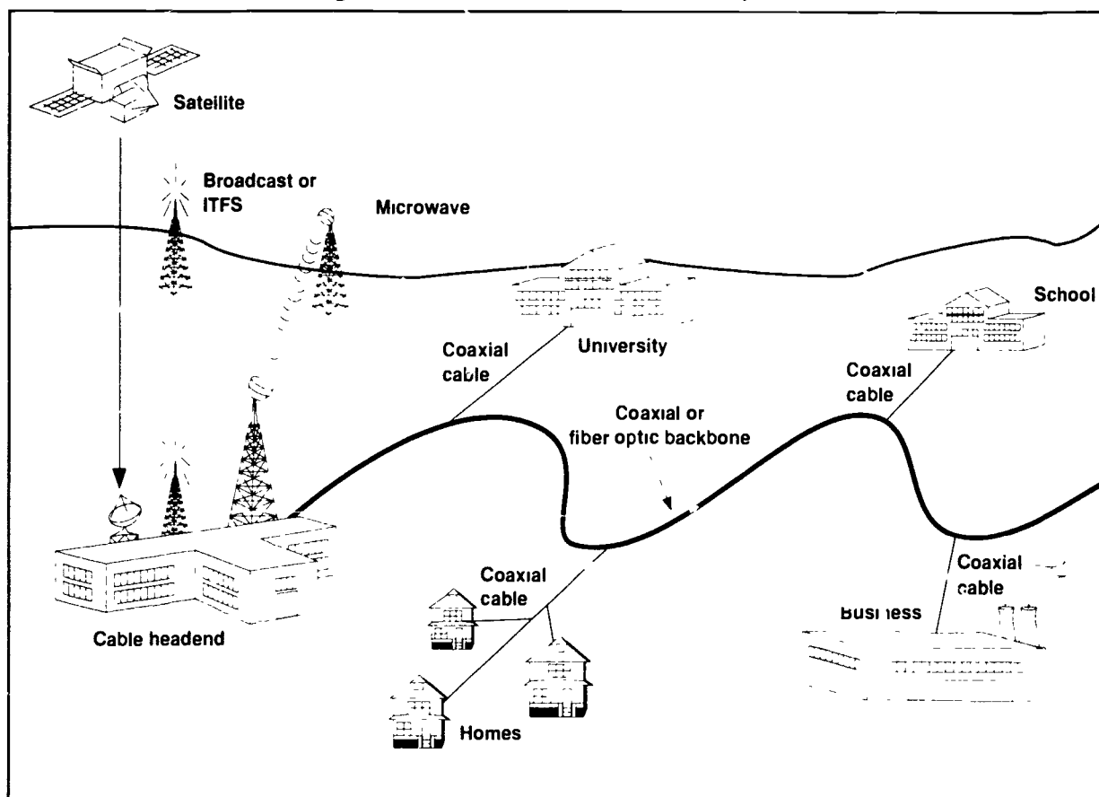
Figure 3-6—Cable Television Distribution System
