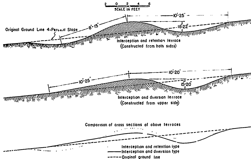
Figure 79.—Terrace cross sections after settlement and cultivation.
