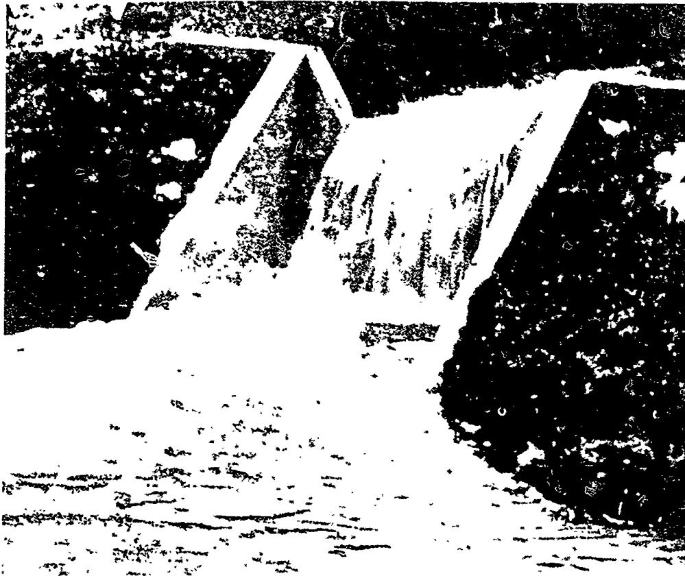
Figure 153. —Reinforced concrete headwall, or drop spillway, where flow from a field ditch drops into an outlet ditch. The apron between the wing walls is below low water in the outlet.
