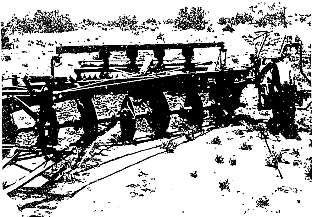
Figure 129. —A range-pitting machine. The alternate disks are mounted 2 inches off center and, in operation, scoop out shallow pits that catch the rainfall and stimulate grass production. This machine has been equipped with cultipacker and seedboxes to permit pitting and seeding in one operation.
