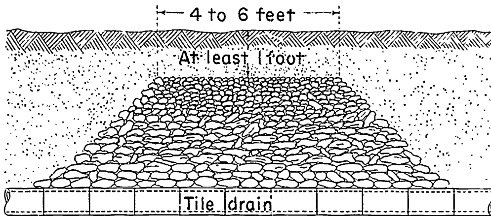
Figure 168.—A blind inlet made by digging out a wet spot over tile and filling it with cobbles, broken tile, and gravel graded upward from coarse to fine. In cropland the top 12 inches should be porous soil.
