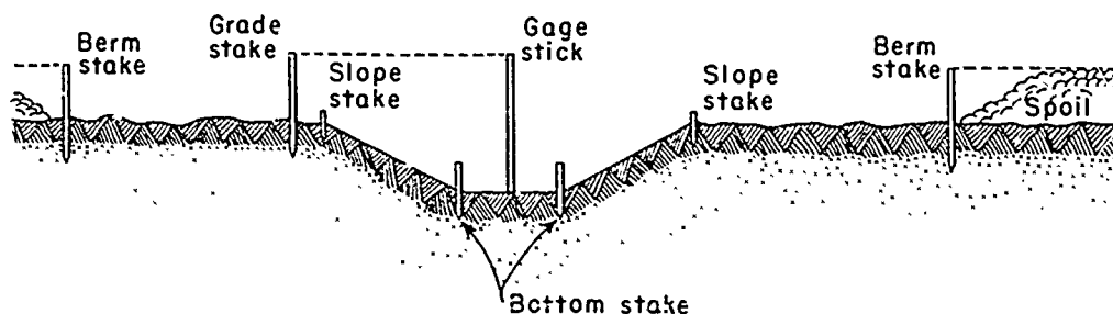
Figure 151.—Cross section of ditch showing the location of the different kinds of construction stakes.
