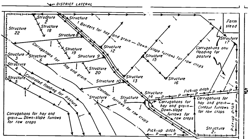
LAY-OUT OF IMPROVED FARM IRRIGATION SYSTEM AFTER LAND GRADING
