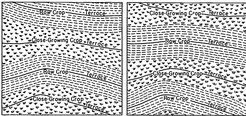
Erosion-Resistant Strip on Alternate Terraces
