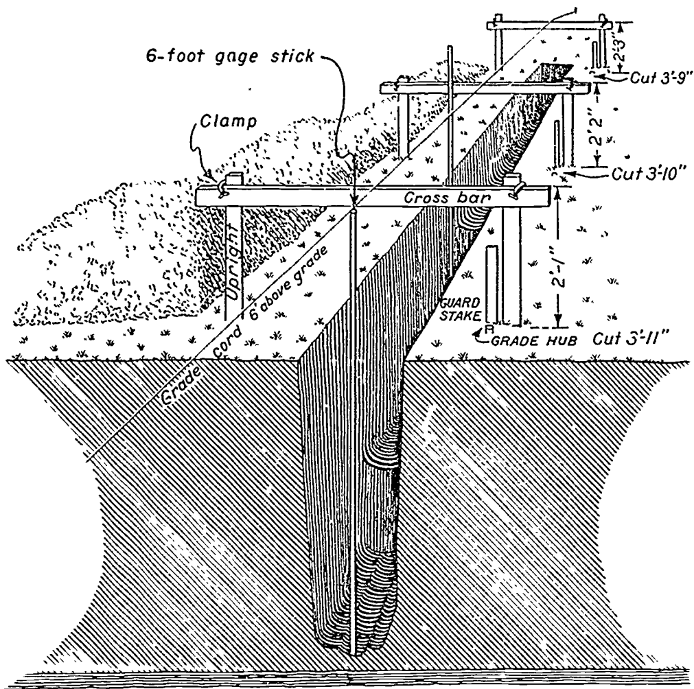
Figure 162. —Gage-and-line method of establishing grade for a tile drain. A cut of 3 feet 11 inches is indicated at the hub in the first station. Subtracting this cut from the length of the gage stick (6 feet), the difference of 2 feet 1 inch is the height for setting the top of the crossbar above the hub. The gage stick at the first station shows that the trench has been dug to the correct grade elevation at that point. The gage stick at the second station shows that more digging is required for the needed cut of 3 feet 10 inches.
