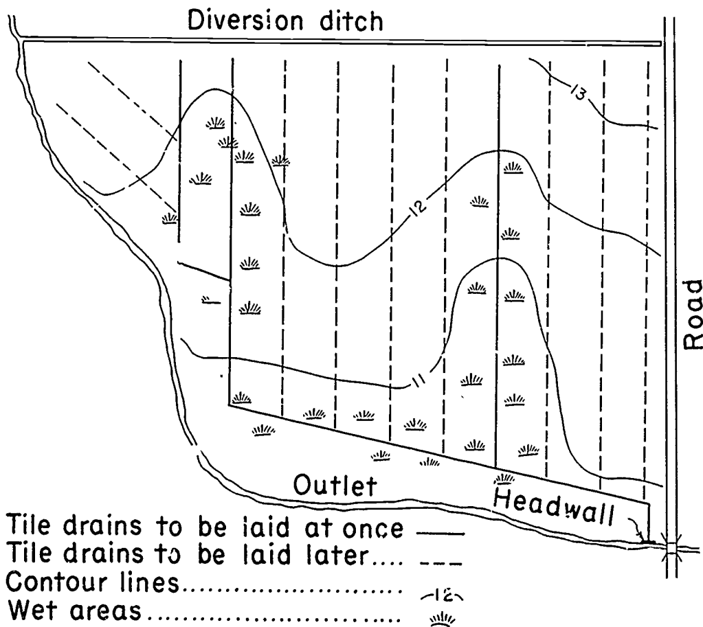
Figure 157.—Plan for a complete system of tile drainage. Random drains are to be installed at once in wettest parts of field and parallel lateral drains to be installed later.
