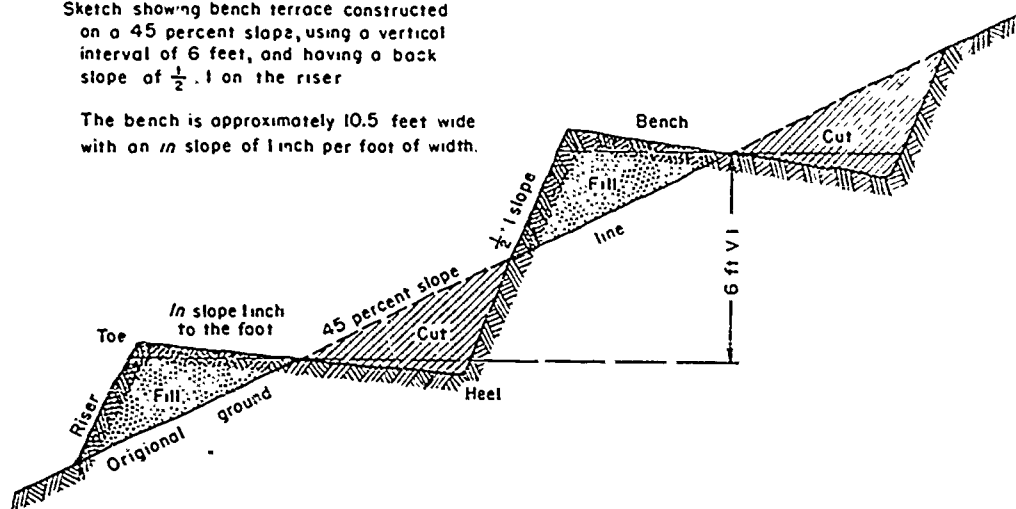
Figure 84.—Cross section of an excavated bench terrace.
