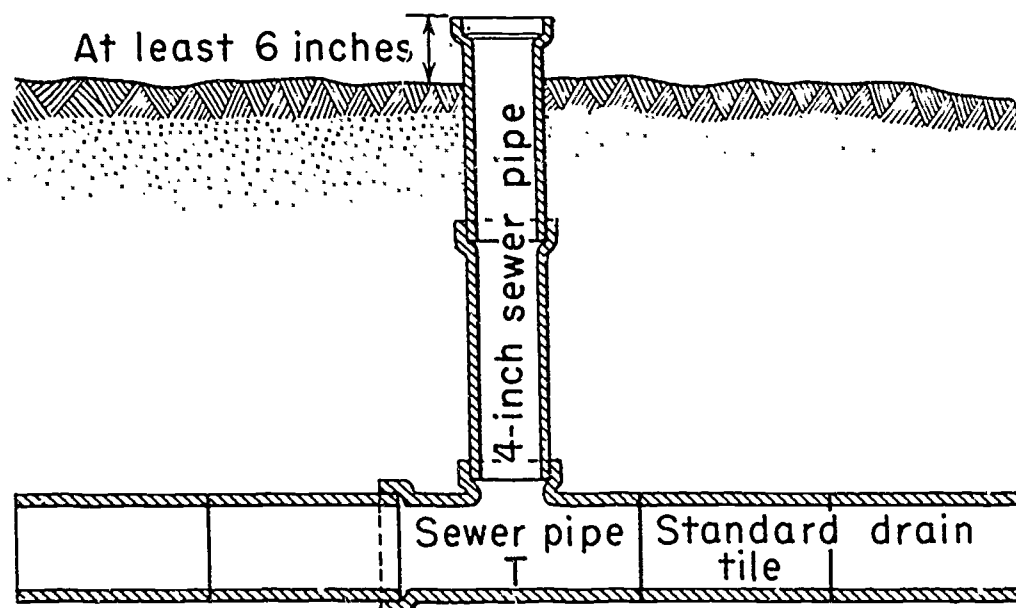
Figure 169.—A pressure relief well made of sewer pipe.
