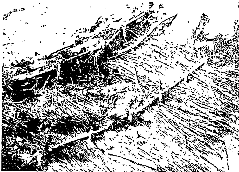
Figure 65.—A dam built of branches in a small gully. Note the sediment deposited above the dam.
