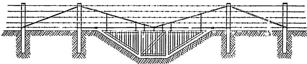
Figure 155. —A three-section watergate, swinging from a cable that can be tightened if it sags. The gate is designed to confine livestock but pass floating debris.
