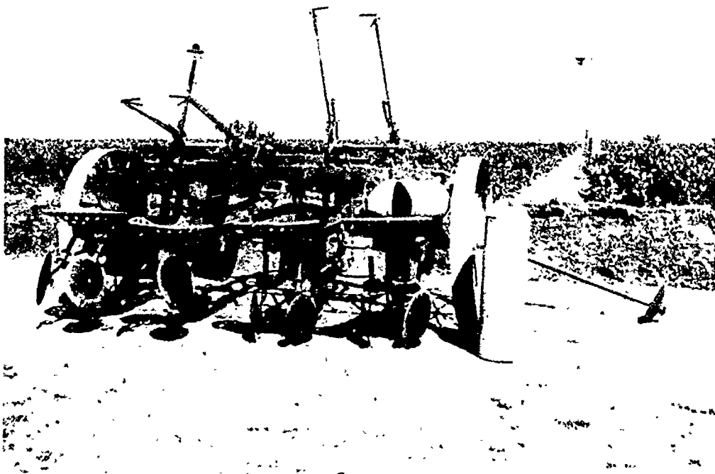
Figure 173. —Rear view of four-row mechanical seeder.
