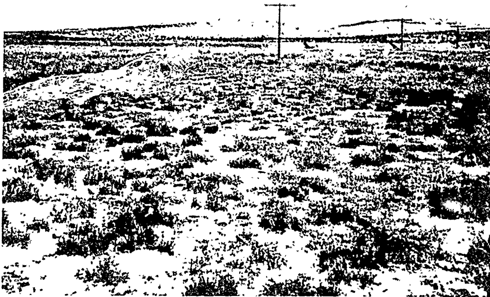
Figure 130. —A water-spreading system consisting of a dike and diversion structures designed to catch the storm waters from the distant slopes and spread them over the depleted but potentially productive flat in the foreground.
