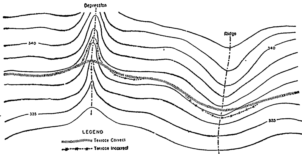
Figure 92.—Realining the terrace line by straightening sharp curves facilitates both terrace construction and tillage operations.
