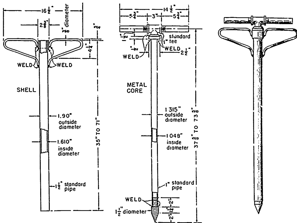
Figure 152.—The Ashley core punch, a useful tool for getting dynamite into wet soils that tend to cave or for getting it under stumps and boulders.
