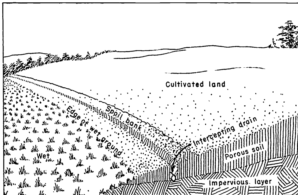
Figure 158.—Proper location for an intercepting drain.
