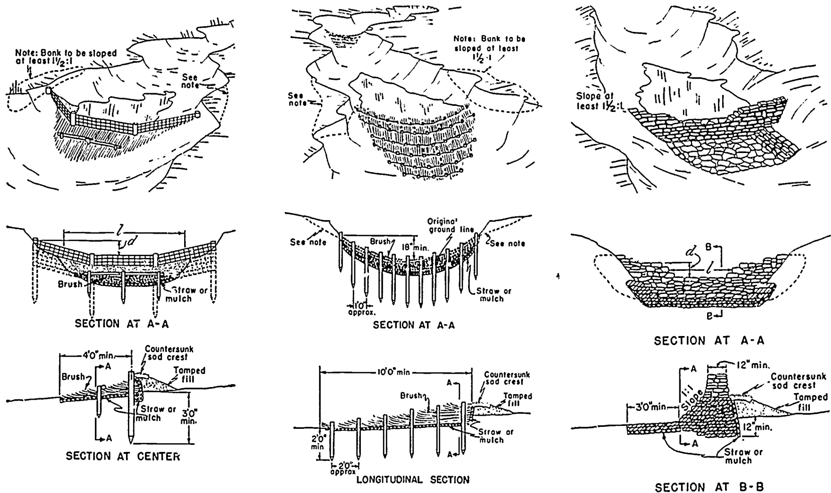
Figure 64.—(Left), a woven-wire dam; (center), a brush dam in common use; (right), a loose-rock dam.
