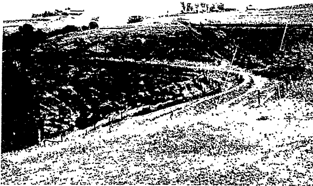
Figure 60. —Water is intercepted by a diversion ditch above the gully and carried to a disposal point so slowly that little erosion occurs. The fence keeps out livestock.
