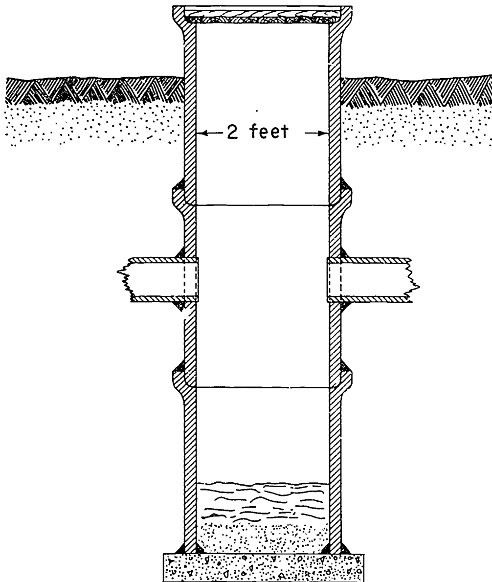
Figure 166. —A silt well made with sewer pipe. Since it has an open top, it also serves as a “relief well.” Like the concrete silt well in figure 167, it can serve also as a junction box where two or more tile lines come together.
