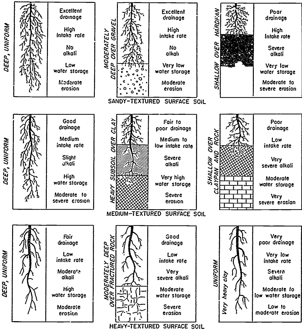
Figure 135. —Some typical irrigated soil profiles indicating effective depth and relative dangers of poor drainage, low intake, alkali, and erosion.
