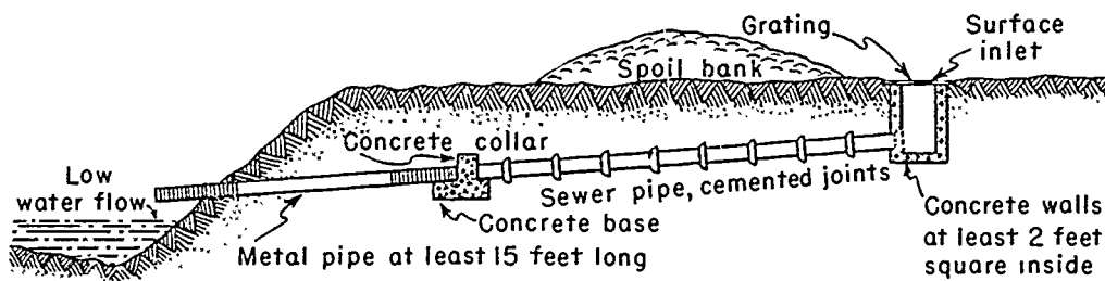
Figure 154. —Pipe outlet under spoil bank to carry surface flow from low ground to drainage ditch. The water enters through a concrete inlet back of the spoil bank.
