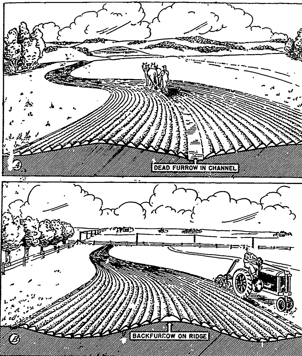
Figure 96.—Maintaining terraces by plowing: A, The channel of the channel terrace can be enlarged by plowing it out. Between channels turn as many of the furrows uphill as possible to offset the natural soil movement down the slope. B, The ridge of the ridge terrace can be enlarged by backfurfrowing to it. The location of the dead furrow should be changed from year to year to avoid excessive depression at any one point.
