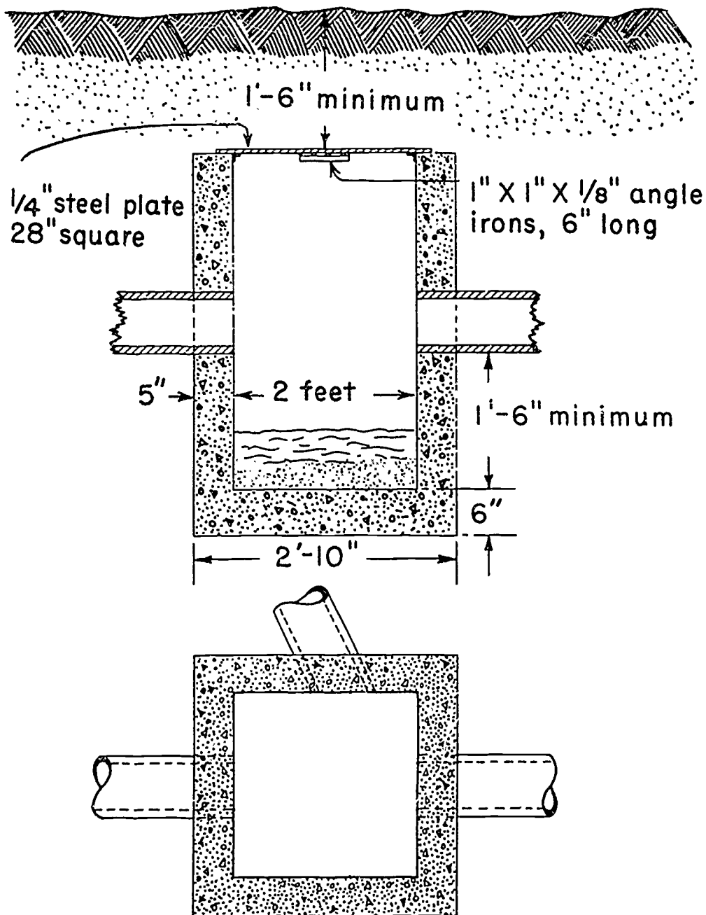
Figure 167.—A silt well made of concrete and sunk below plow depth so as not to interfere with cultivation. Silt wells can also serve as junction boxes, as shown in the cross section that is the lower part of the drawing.
