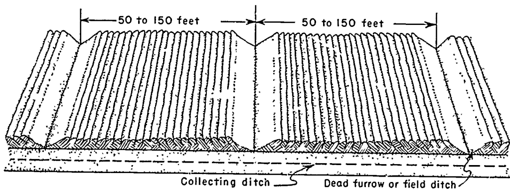
Figure 150.—How to plow a field divided by field ditches.
