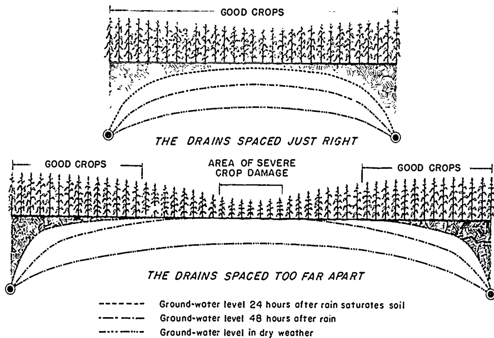
Figure 159.—How spacing of tile drains affects ground-water level and crop damage.
