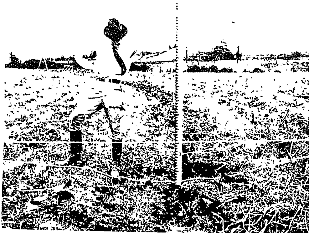
Figure 80. —A broad-channel terrace in the Piedmont area. To be effective, the channel must have ample capacity.
