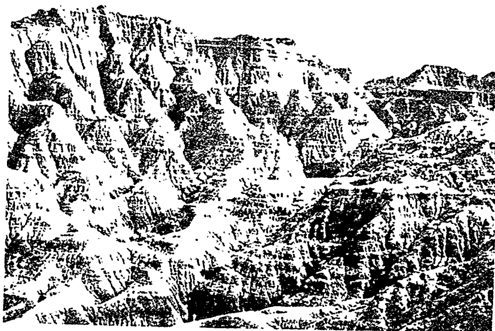
Figure 7. —The Badlands are typical of land forms produced under certain conditions of geology.
