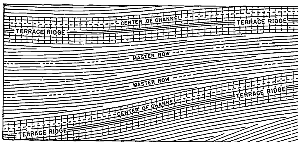
Figure 100.—Arranging point rows between master rows on terraced land places all the rows more nearly on the contour than does any of the methods shown in figure 99. This is the most intricate of the four suggested arrangements.
