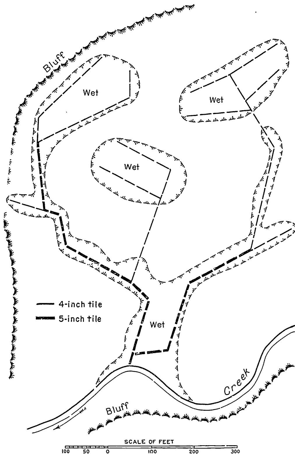
Figure 156.—Plan for a random system of tile drainage. Main drains are to be laid in the natural waterways and smaller branch lines in large wet areas.
