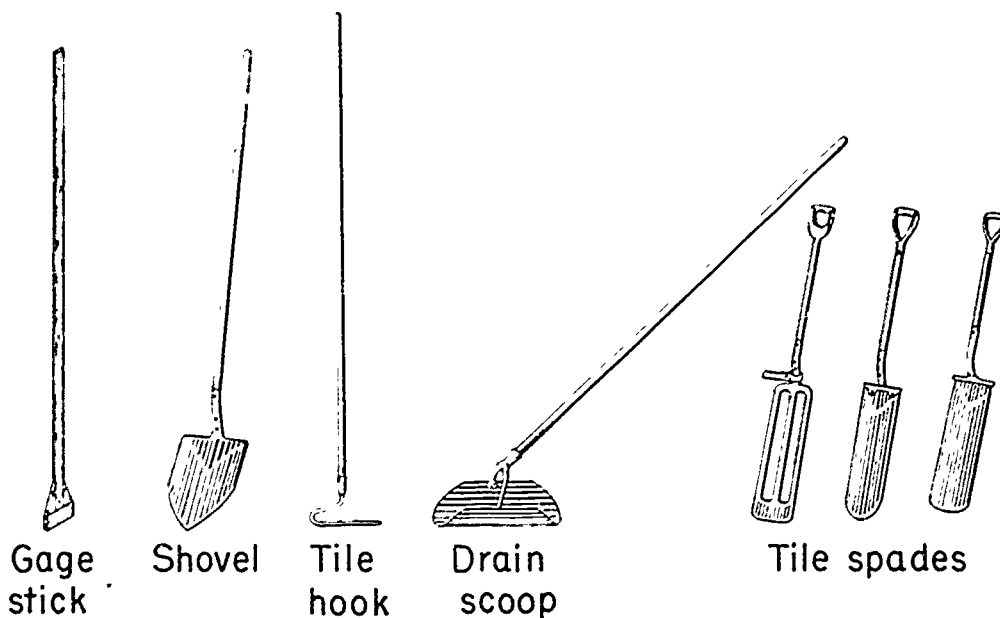
Figure 161.—Handtools for tile-drain construction.
