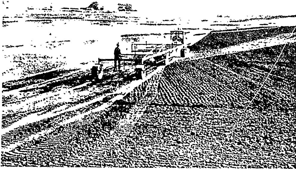
Figure 143. —Smoothing out the land surface with a landplane.
