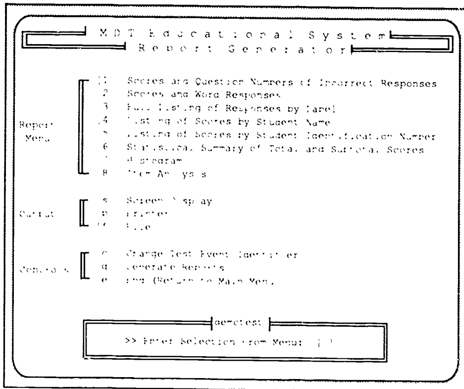
Figure 4-9: Monitor Screen for Standard Reports
