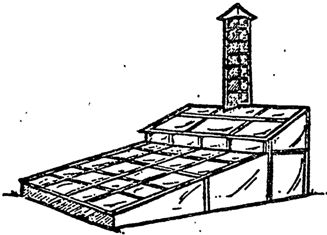
Fig. 13 International Rice Research Institute solar rice dryer, Thailand
