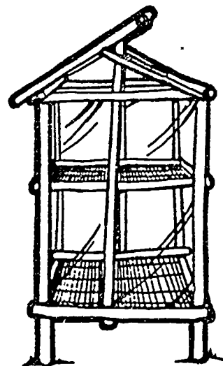
Fig. 24 Solar cabinet dryer, Indonesia
