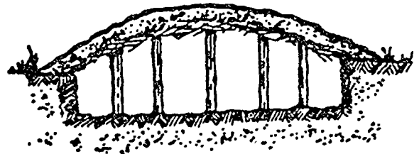
Fig. 40 Semi-subterranean potato storage house
