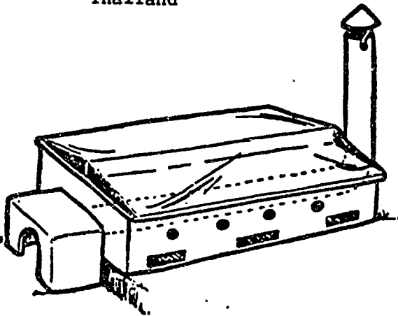
Fig. 15 VITA solar dryer with fuel-fired rainy season dryer attached
