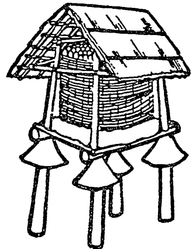
Fig. 48 Traditional store improved with rat guards
