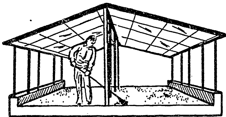
Fig. 21 Plastic-covered concrete drying floor for coffee, Columbia
