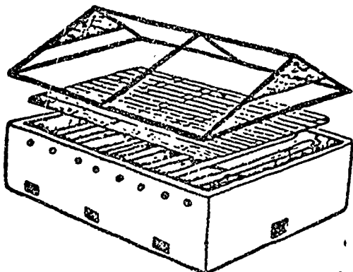
Fig. 11 Improved VITA solar dryer
