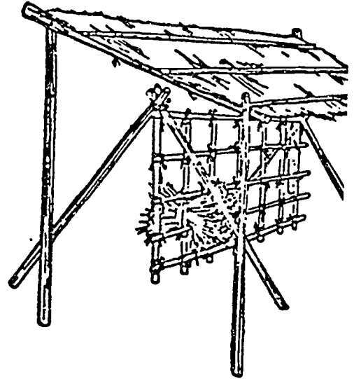
Fig. 8 Improved post-harvest dryer for rice, Sierra
