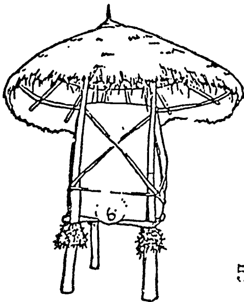
Fig. 35 Improved muddied basket with rat guards, Kenya
