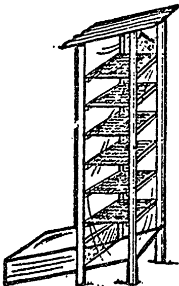
Fig. 17 Solar "chimney" dryer with pre-heater
