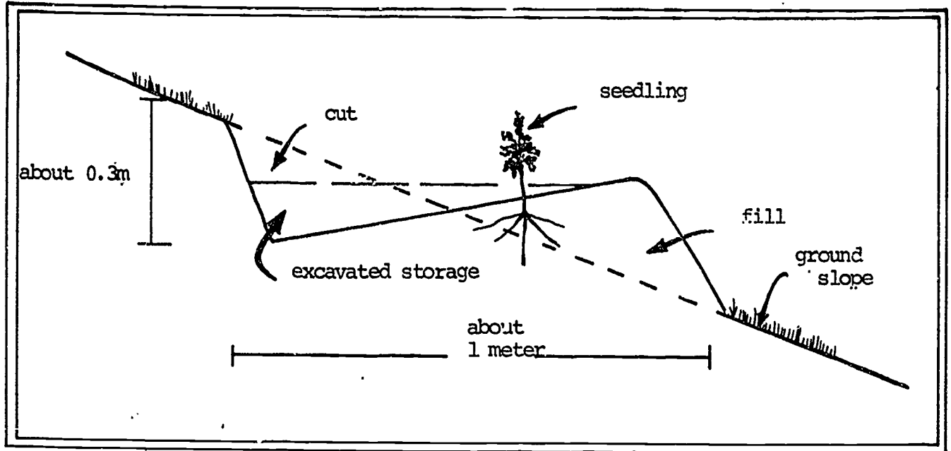
Figure 28. Cross-sectional View of Gradonis
