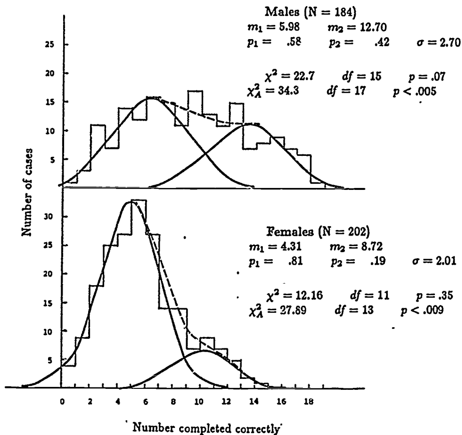
Figure 4: Score distributions by sex for the Vandenberg-Shepard test. Both distributions can be represented as the sum of two normal components. A single component does not fit the data. Adapted from Zimowski (1985).
