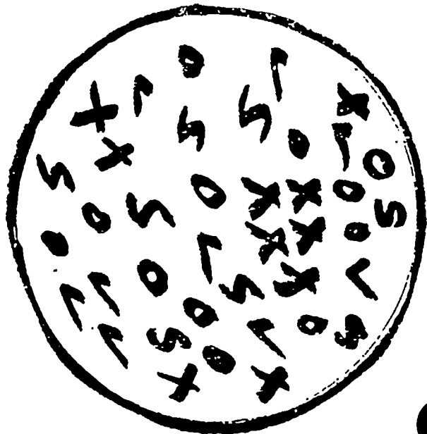
Water Sample #2
