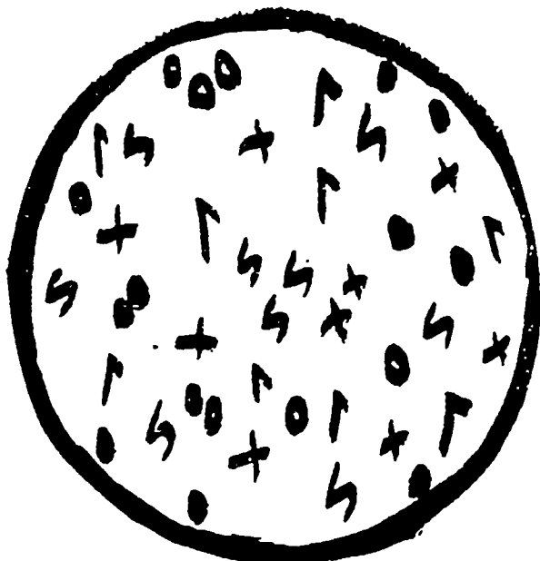
Water Sample #3
