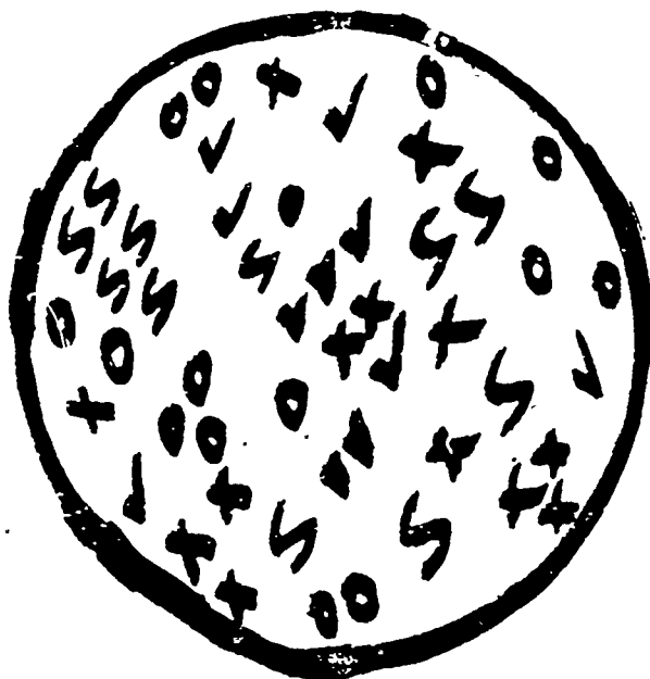
Water Sample #1
