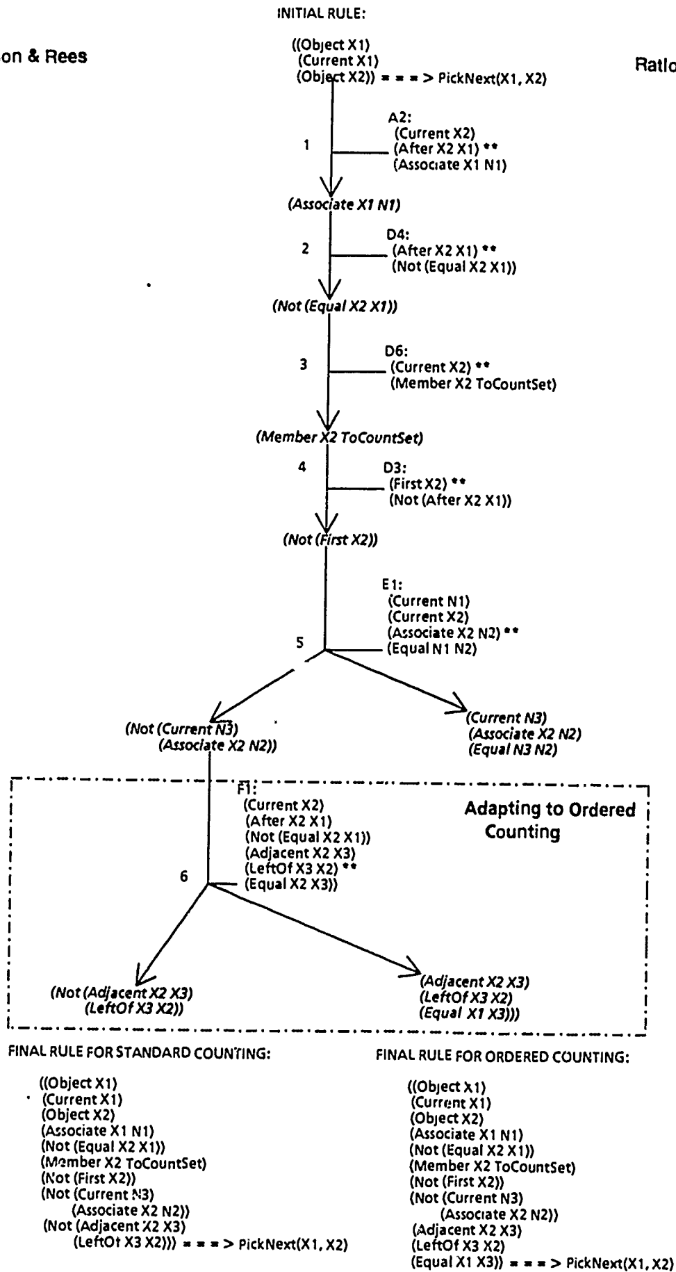
Figure 9: Revisions of rule 2 (see Figure 7) in adaption to ordered counting.
