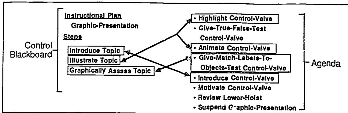
Figure 5-1: Representation and Interpretation of an Instructional Plan
