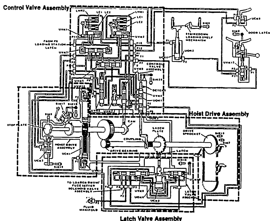
Figure 3-1: Schematic of the Lower Hoist Assembly
