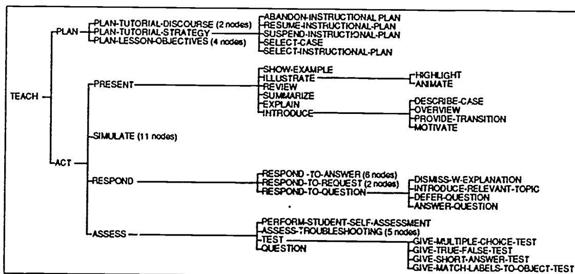
Figure 6-1: A Taxonomy of Verbs Representing Instructional Actions
