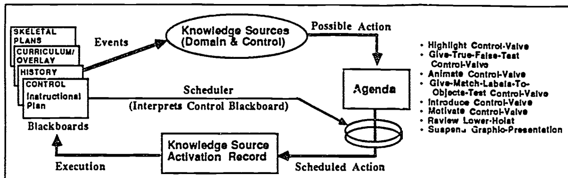
Figure 4-1: The BB1 Blackboard Execution Cycle
