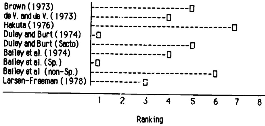
Figure 1. Article Ranking in Several Studies
