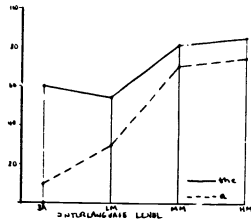
D Lamotte et al (1982) Spanish the and a TLU
