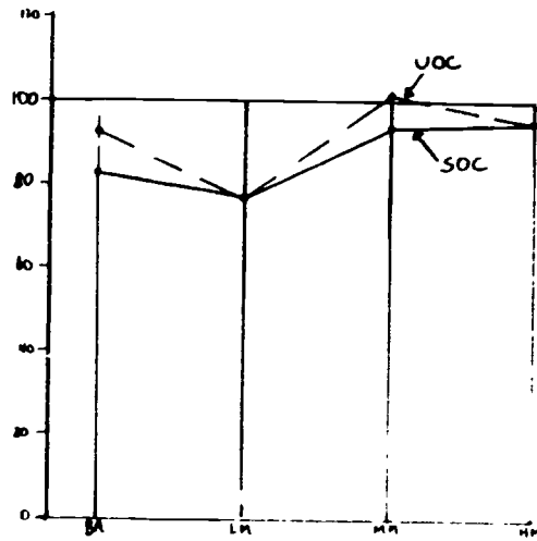
B \alpha SOC and UOC German
