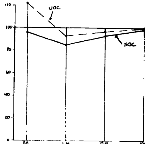
C \theta SOC and UOC German
