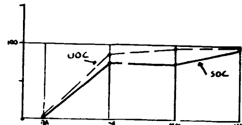
C \leq SOC and UOC - Chinese
