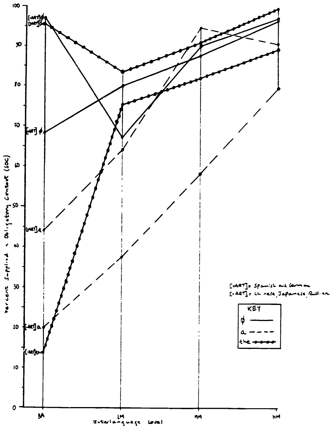
Figure 5. Overall Article Accuracy
