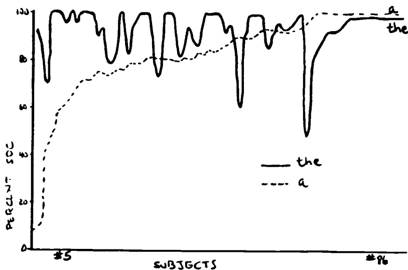
B. Andersen's Spanish Subjects' the and a SOC
