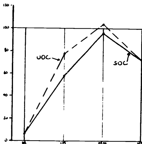
B. a SOC and UOC: Spanish
