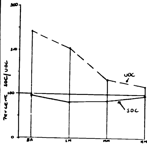
A \phi SOC and UOC - Chinese
