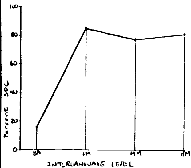
A. Japanese Subjects the SOC
