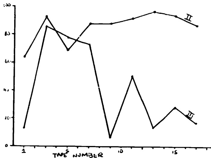
B. Ge's the Usage in Categories II (correct) and III (incorrect)
