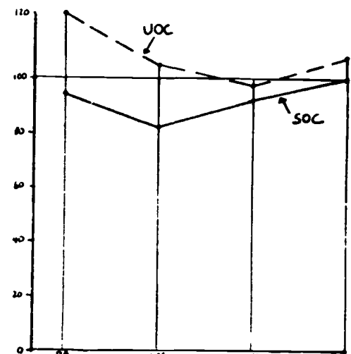
C. the SOC and UOC. Spanish
