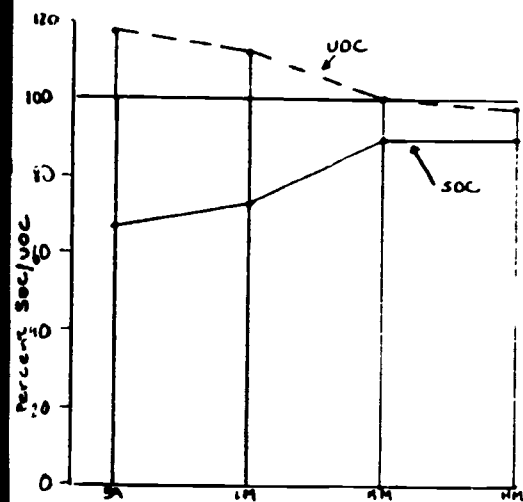
A. \phi SOC and UOC. Spanish
