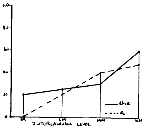
B. Lamotte et al. (1982) Japanese the and a TLU
