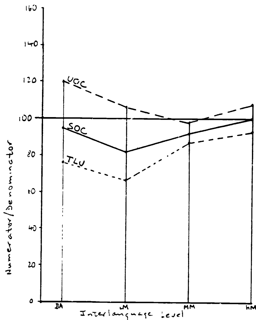
Fig. 13. Comparison of UDC, SOC, and TLU in the Spanish Subjects' Usage of the
