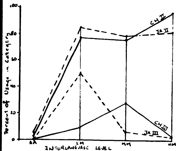
A. Chinese and Japanese the Usage in Categories II (correct) and III (incorrect)
