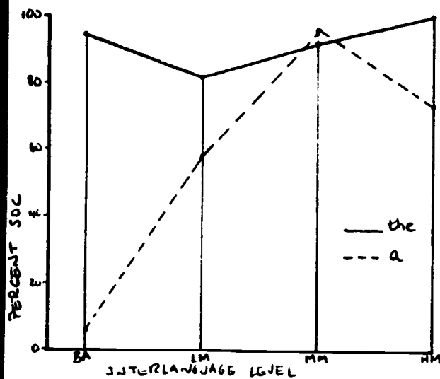
A. Spanish Subjects' the and a SOC
