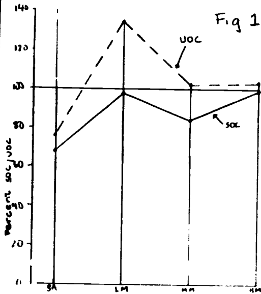
A \phi SOC and UOC German
