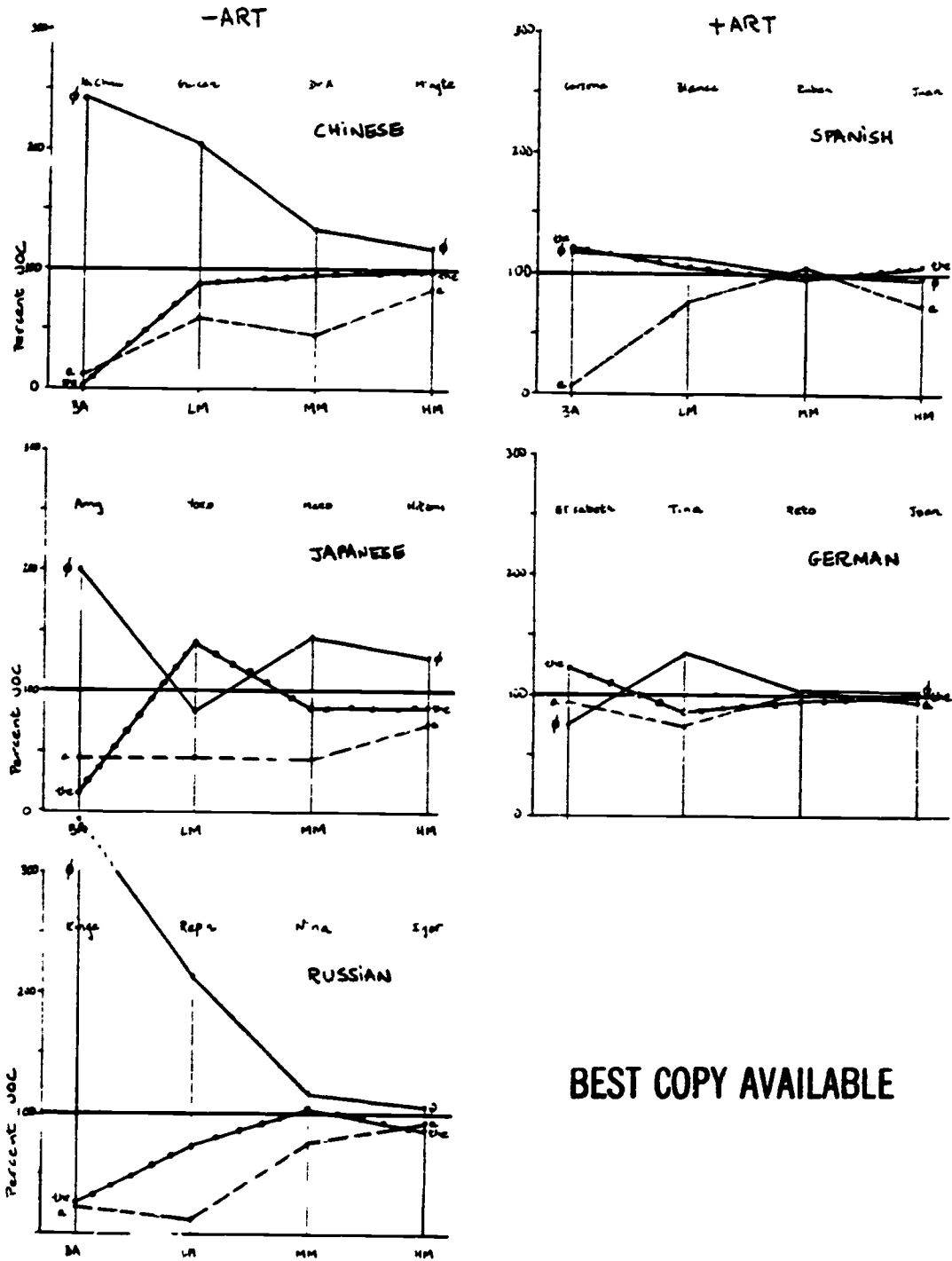
Fig. 7. Articles Used/Articles Required (UOC)
