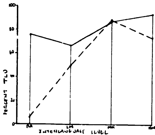
C Spanish Subjects' the and a TLU
