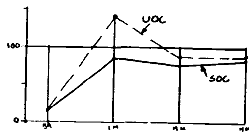
C. \beta SOC and UOC Japanese
