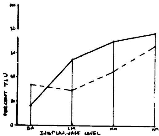
A Japanese Subjects' the and a TLU
