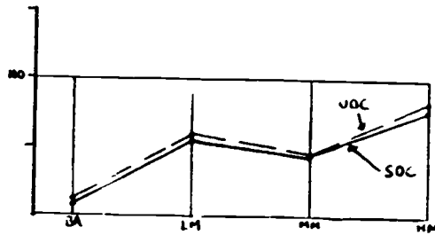
B. \leq SOC and UOC - Chinese
