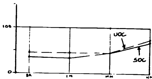
B. \alpha SOC and UOC Japanese
