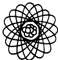
Gold — 79 protons
