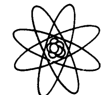
Carbon — 6 protons
