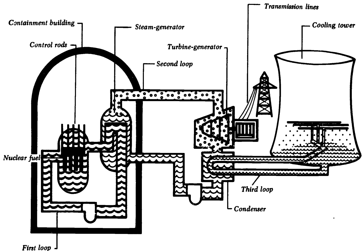
Pressurized Water Reactor
