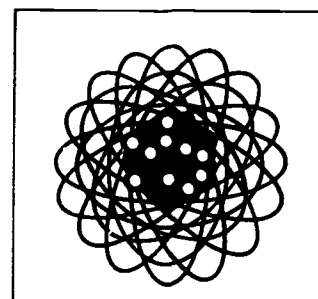
Uranium-238
