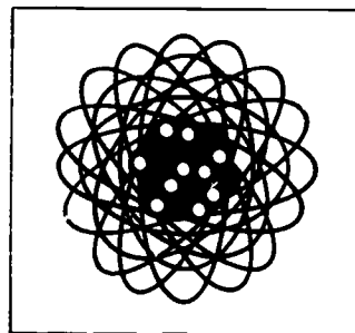
Uranium-235
