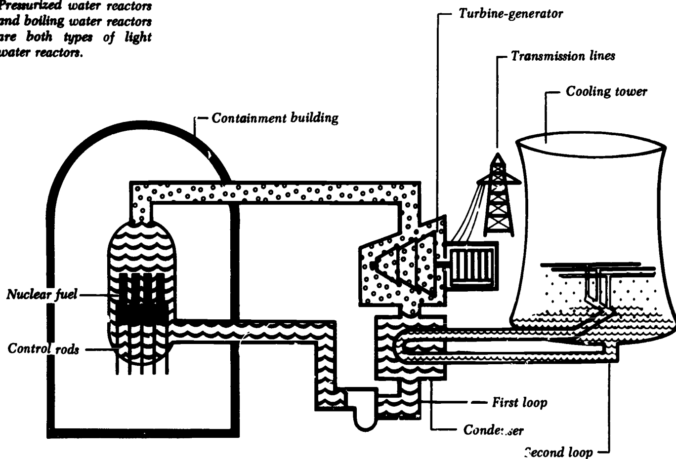
Boiling Water Reactor
