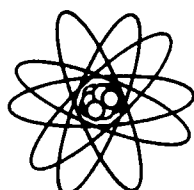
Iron — 26 protons
