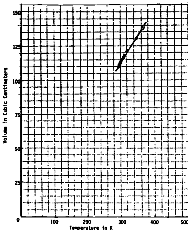
Figure 5. The data of Fig. 2 graphed with the zeros of both scales located at the intersection of axes.
