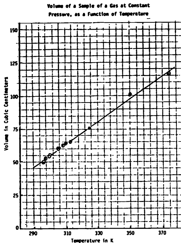
Figure 6. The data of Fig. 2 graphed employing expanded scale.
