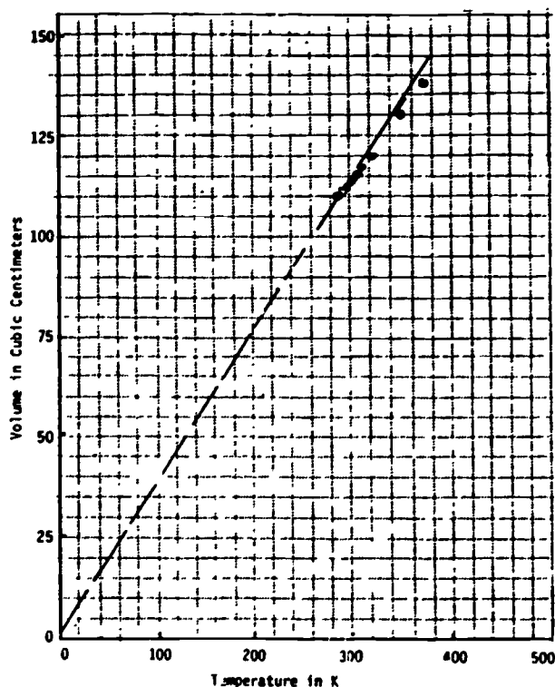
Figure 7. Figure 5 re-drawn using knowledge gained from Figure 6.
