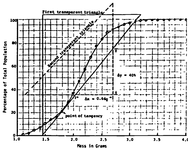
Figure 13. Determination of slope ( \Delta y / \Delta x ) by Method of Tangents. At x = 1.8g .
