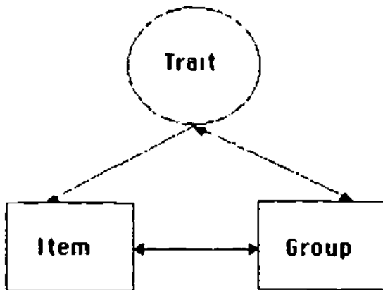
Figure 1 Graphical display of (a) association of group membership and item responses, (b) an unbiased item, (c) a biased item, and (d) a biased item where the bias disappears by introducing an additional trait.
