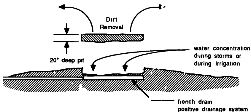
Figure 3.7 When using a pit positioned on top of a knoll to contain loose safety surface material, a french drain is a good example of a positive drainage system.
