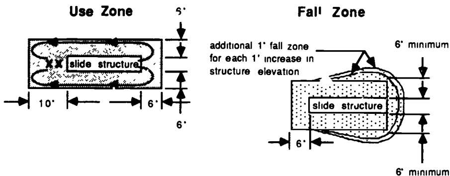
Figure 3.4 The use zone and the fall zone frequently overlap.
