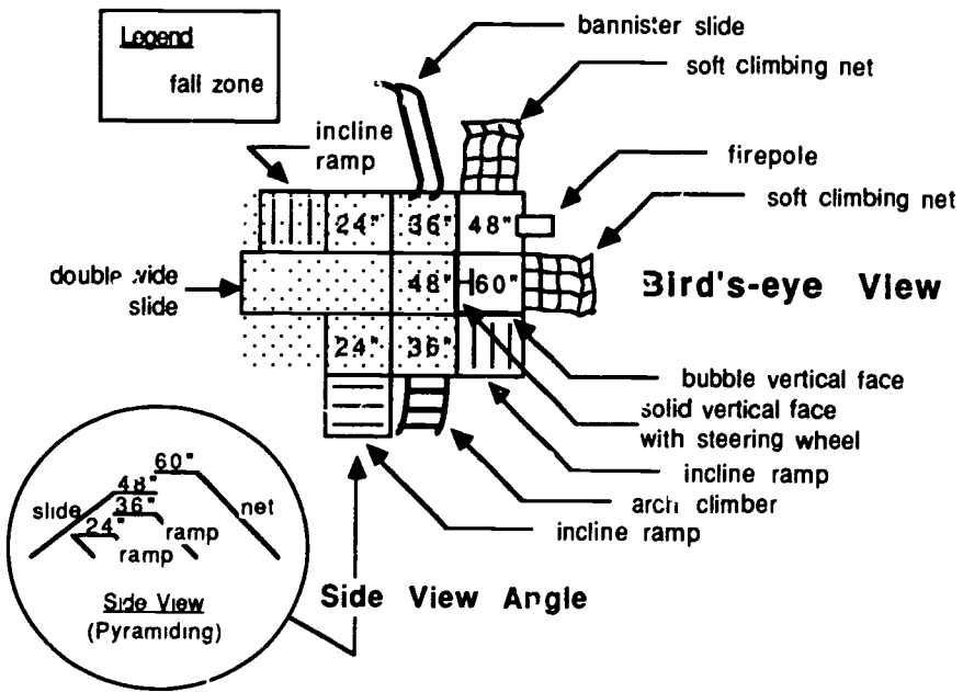
Figure 3.5 The concept of fall zone is slightly modified for application to linked structures which employ the pyramiding concept.
