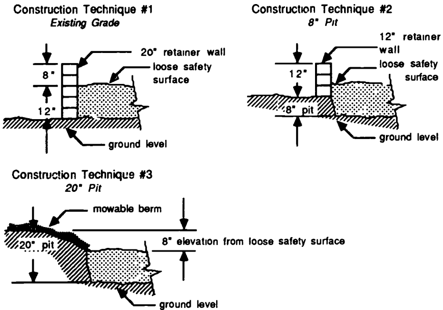
Figure 3.6 Three variations or techniques can be used for containing loose safety surface material. Two of these include the construction of a retainer wall.
