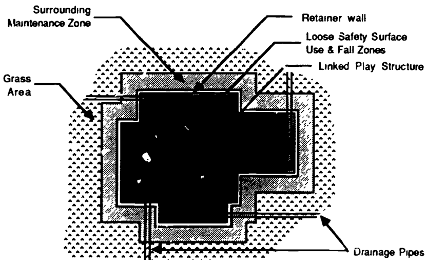
Figure 3.8 The surrounding maintenance zone is the area where the heaviest overflow of loose safety material will accumulate. Using decomposed, compacted granite helps keep the maintenance of this zone less labor intensive.
