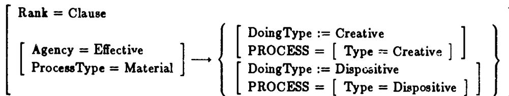
Figure 14: DoingType system in FUG, using disjunction and negation.
