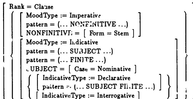
Figure 11: MoodType and IndicativeType Realizations
