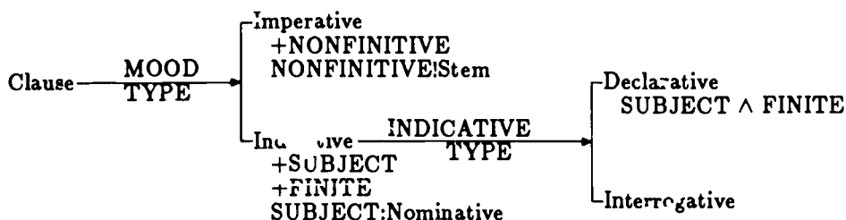
Figure 11: MoodType and IndicativeType Realizations
