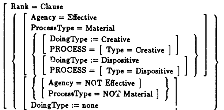
Figure 13: The DoingType System
