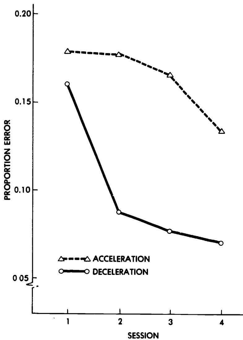
Figure III-6. Proportion error as a function of session for events representing accelerating and decelerating self motion
