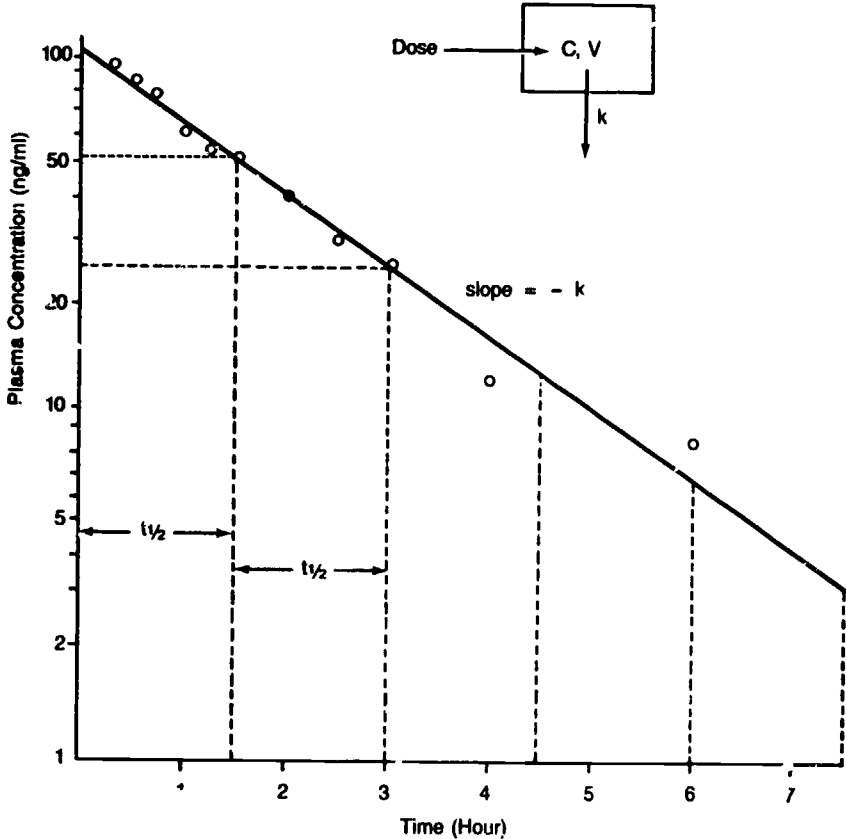
Figure 6. Plasma levels of cocaine (o) following an intravenous dose of 20 mg cocaine. Solid curve is a computer fit of the data to a one-compartment model (data from Cook et al. 1985). The inset is a schematic representation of a one-compartment model.
