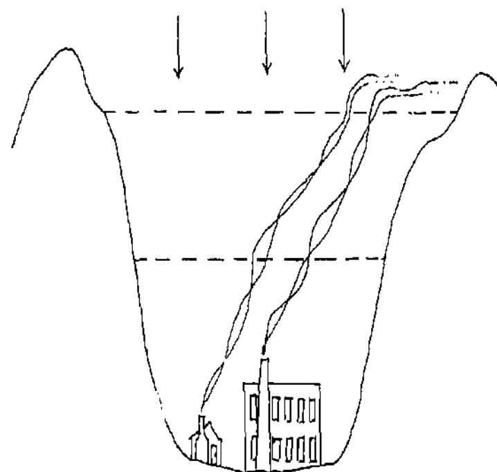
EFFECT OF TOPOGRAPHY ON AIR CIRCULATION
