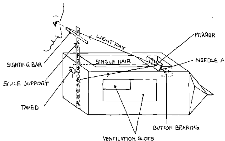
SIMPLE HAIR HYGROMETER.
