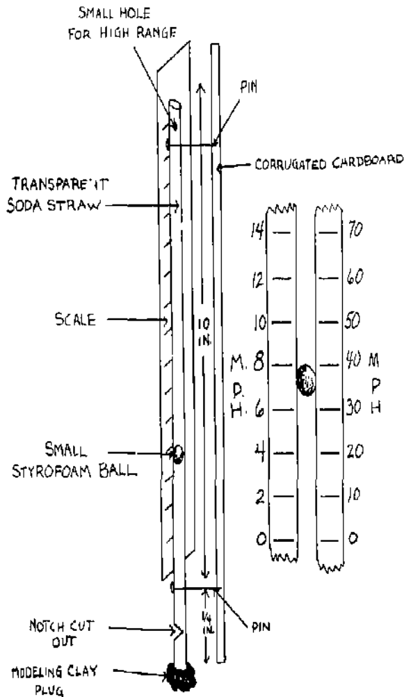
WIND-SPEED INDICATOR
