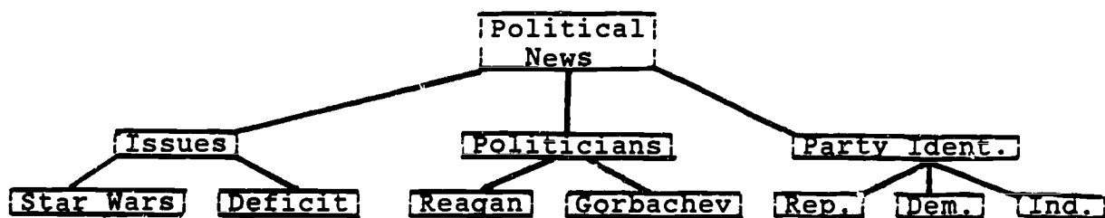
[Figure 3: Possible levels of abstraction in news processing]
