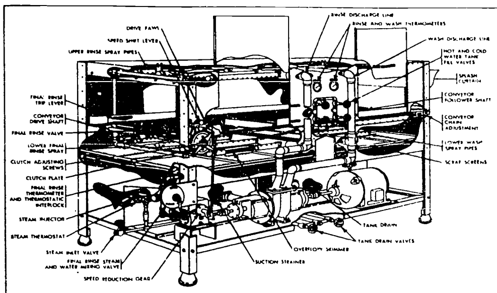
Figure 2-17. Typical Automatic Double-Tank Dishwashing Machine
