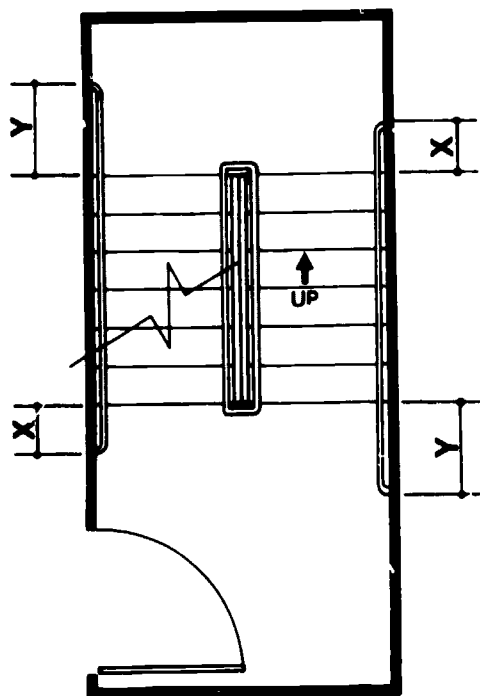
(a) Plan
