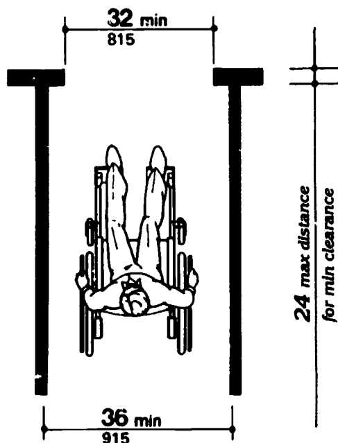
Fig. 1 Minimum Clear Width for Single Wheelchair
