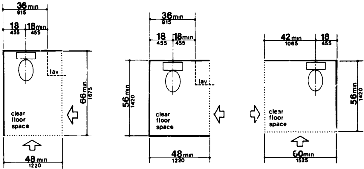
(a) Clear Floor Space for Adaptable Bathrooms
