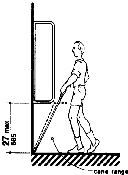
(b) Walking Perpendicular to a Wall
