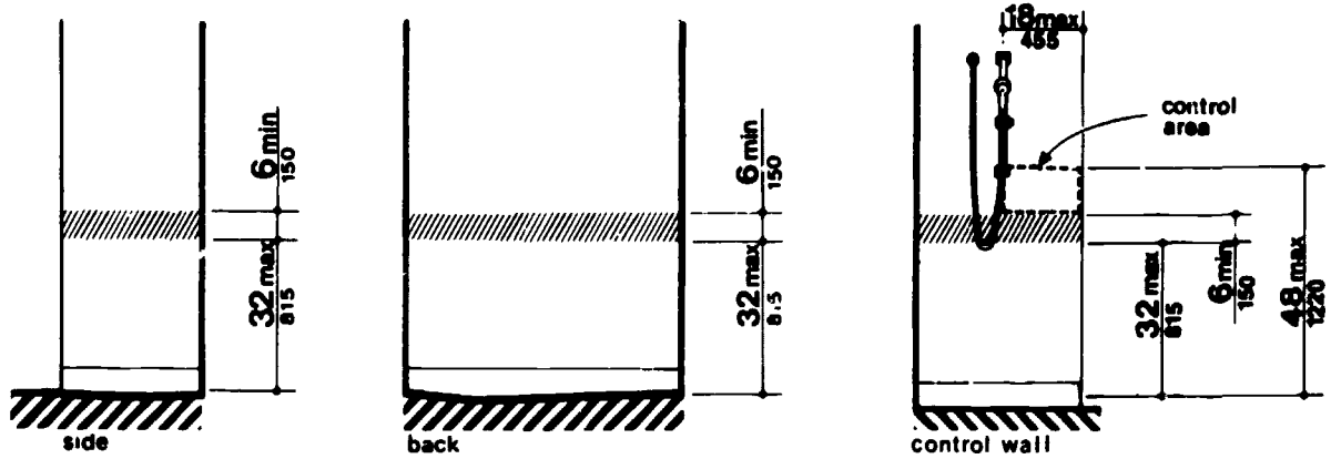
(b) 30-in by 60-in (750-mm by 1525-mm) Stall
