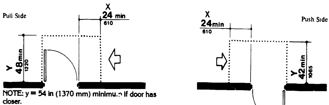
(b) Hinge Side Approaches — Swinging Doors
