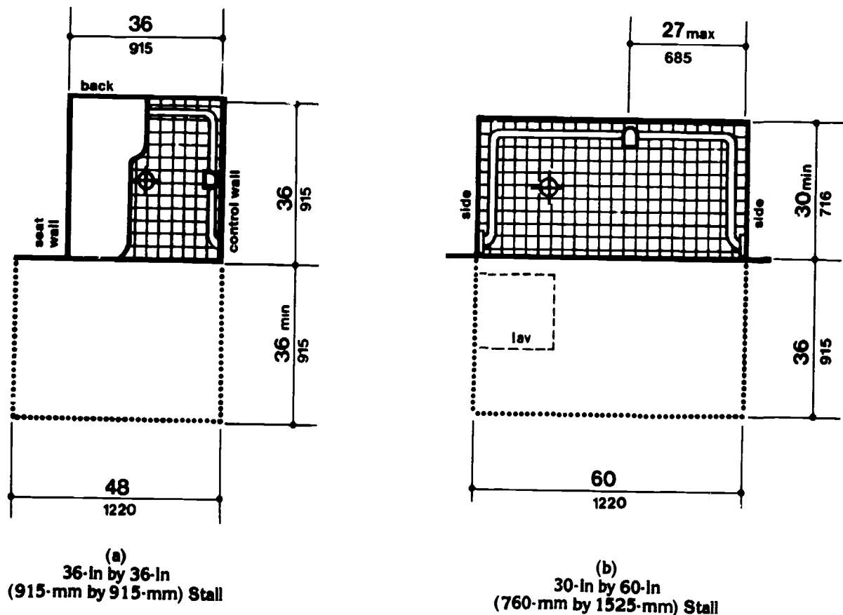
Fig. 35 Shower Size and Clearances
