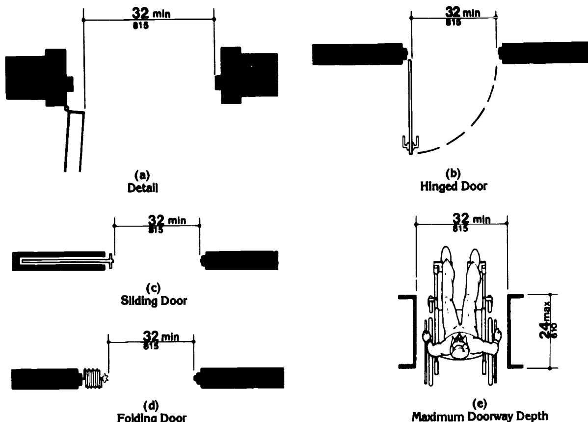
Fig. 24 Clear Doorway Width and Depth
