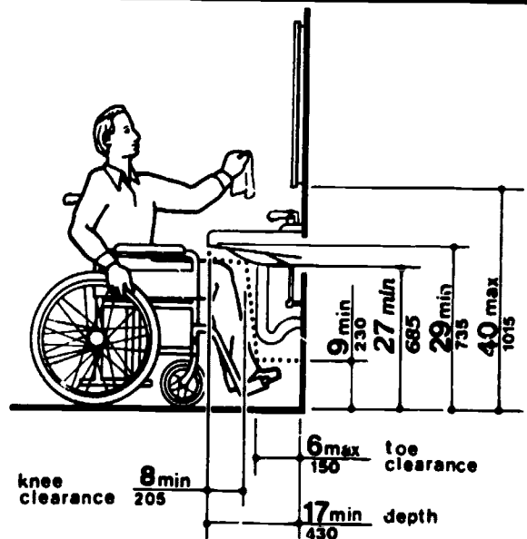
Fig. 31 Lavatory Clearances
