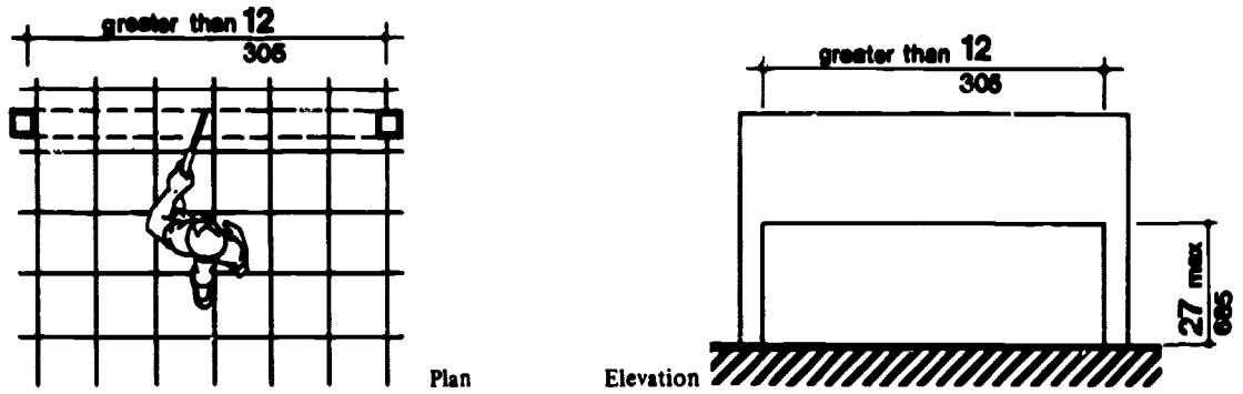
(c) Free-Standing Overhanging Objects
