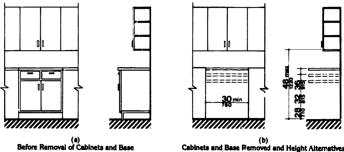
Fig. 50 Counter Work Surface
