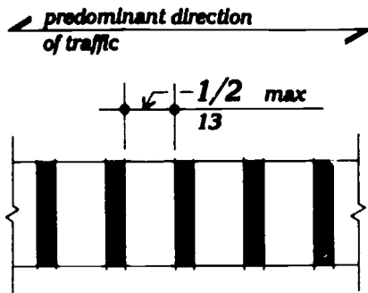
Fig. 8(g) Gratings
