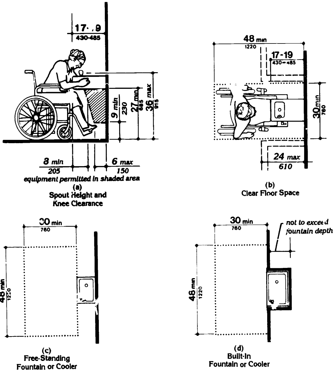
Fig. 27 Drinking Fountains and Water Coolers
