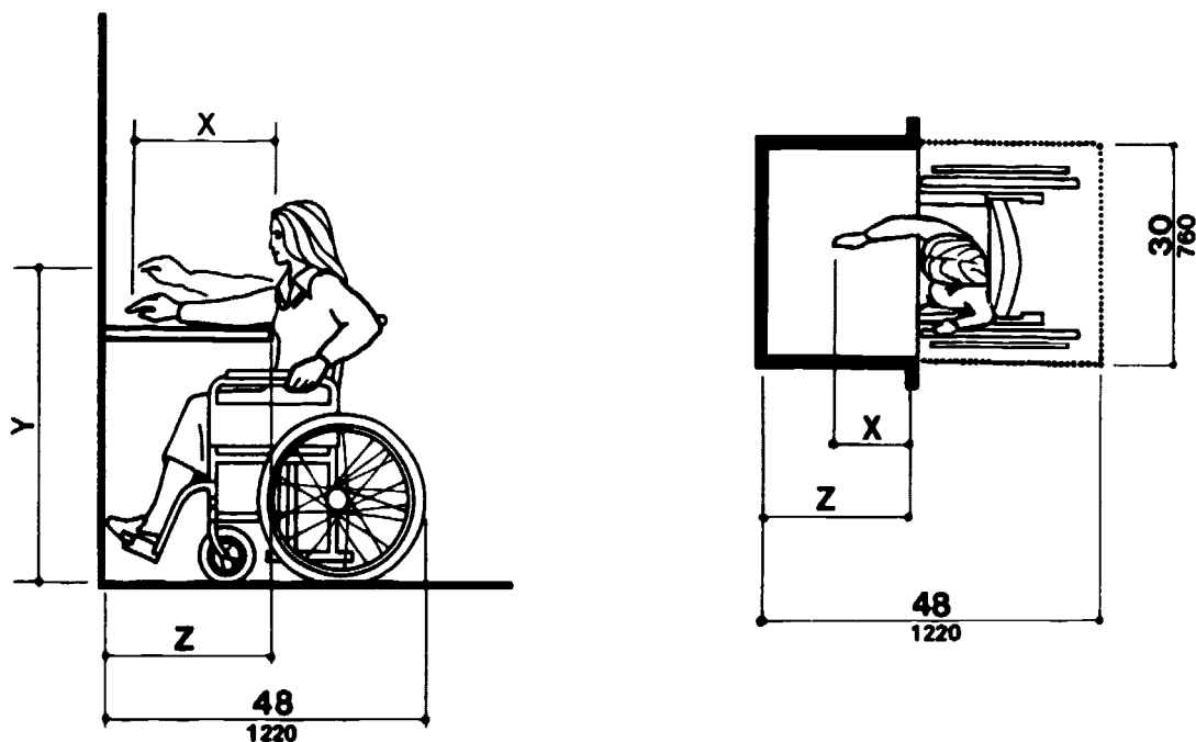
(a) High Forward Reach Limit
