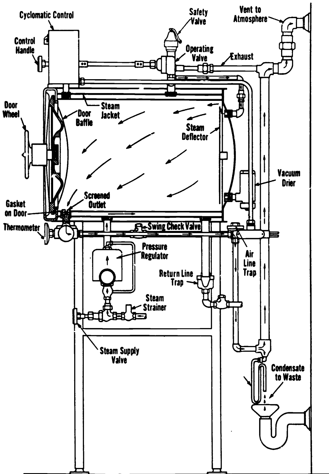
Figure 2-8. Autoclave (Courtesy of American Sterilizer Company, Erie, Pennsylvania)
