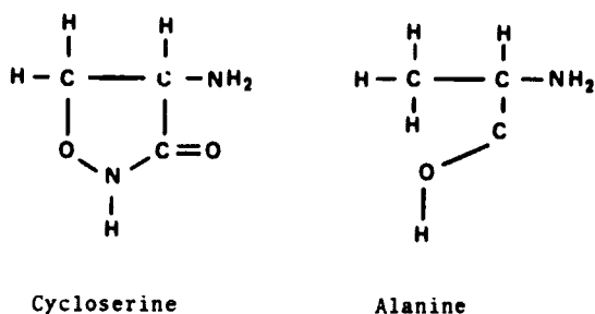
Figure 5-3. Structural formulas of cycloserine and alanine.
