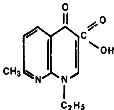
Figure 5-7. Structural formula for nalidixic acid.
