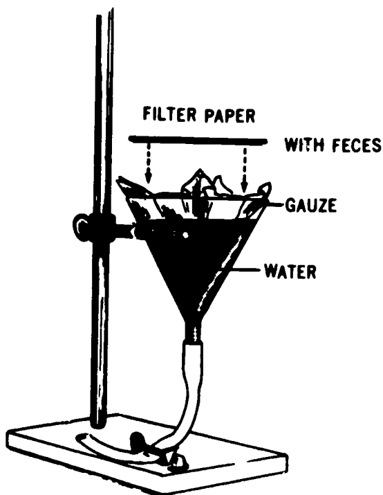
Figure 4-6 Baermann apparatus
