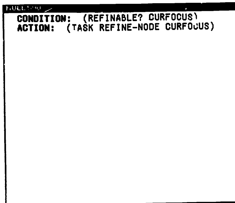
Figure 4-5: The Rule Window displaying a metarule of the task Pursue-Hypothesis.
