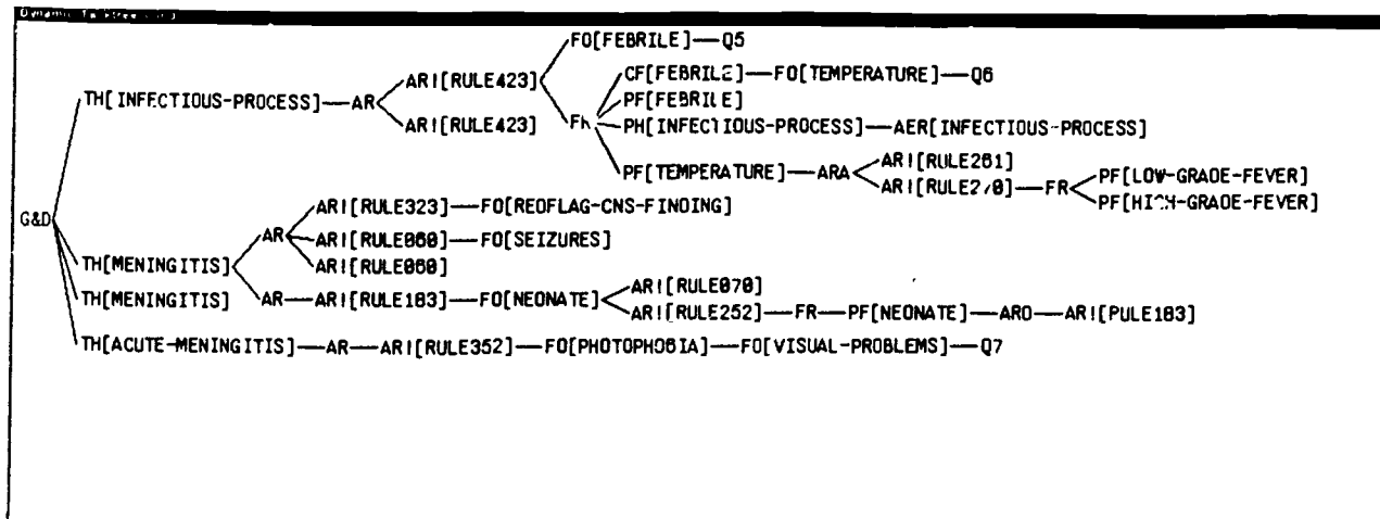
Figure 4-14: The Dynamic Task Tree Window.
