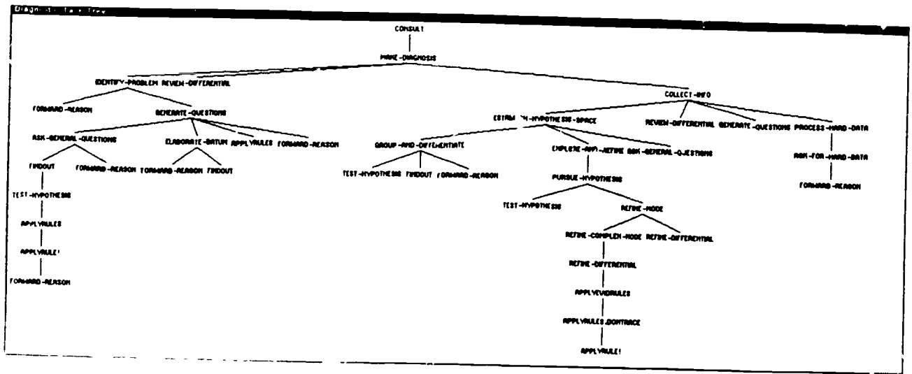
Figure 4-6: The Diagnostic Task Tree Window.
