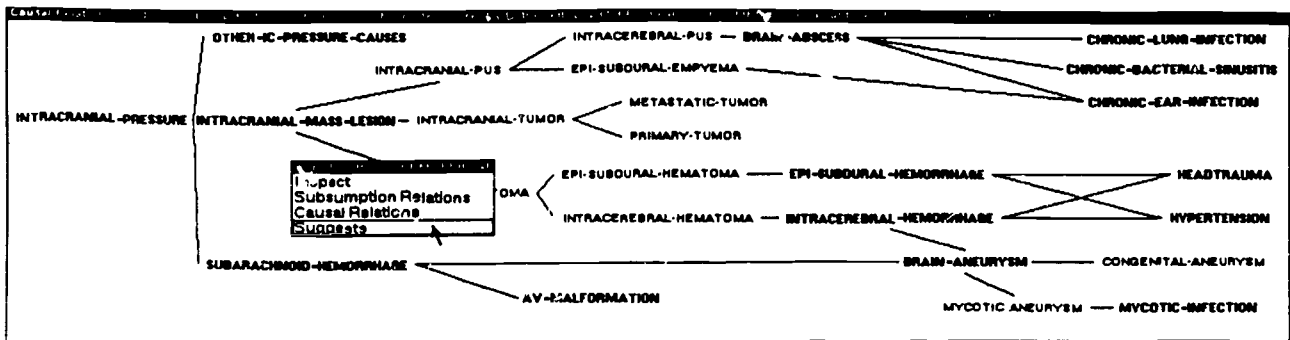
Figure 4-2: The Causal Relations Window.
