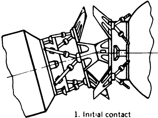
Figure 2-4.—Docking Mechanism Developed for Use in ASTP
