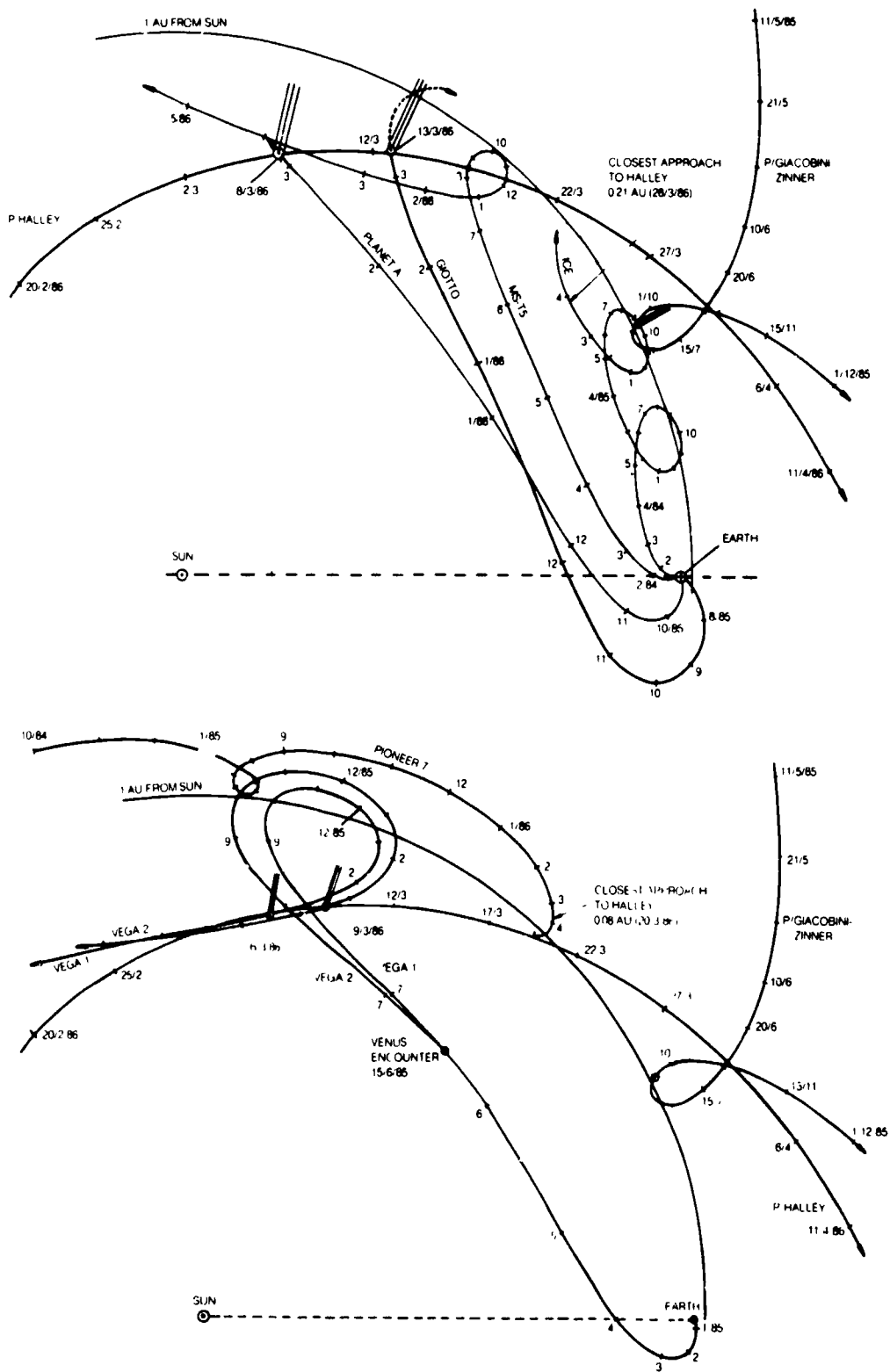
Figure 2-6.—Trajectories of the Various Halley Spacecraft Relative to a Fixed Sun-Earth Line
