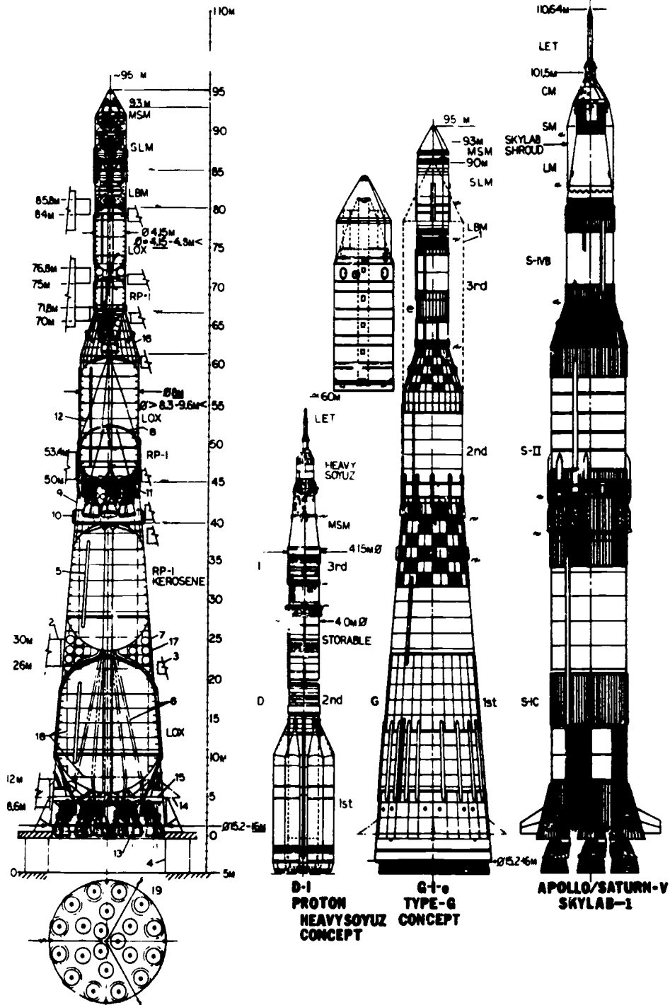
Figure 2-1.—Soviet Type G Booster, and U.S. Saturn V
