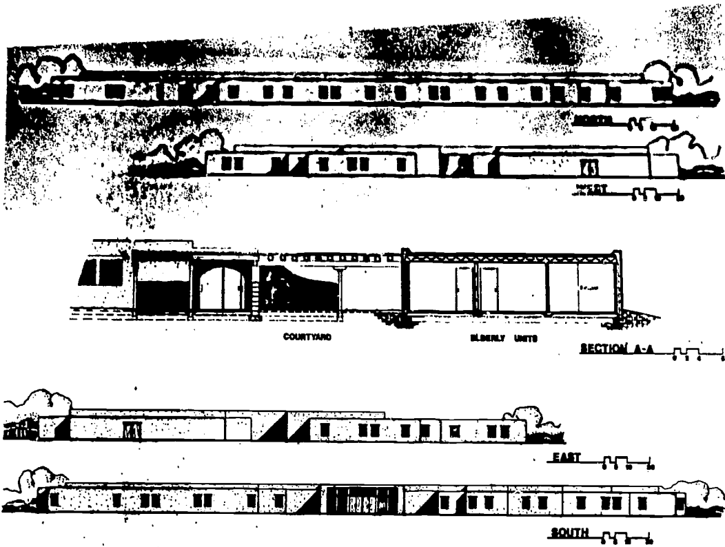
ELEVATIONS & SECTION
