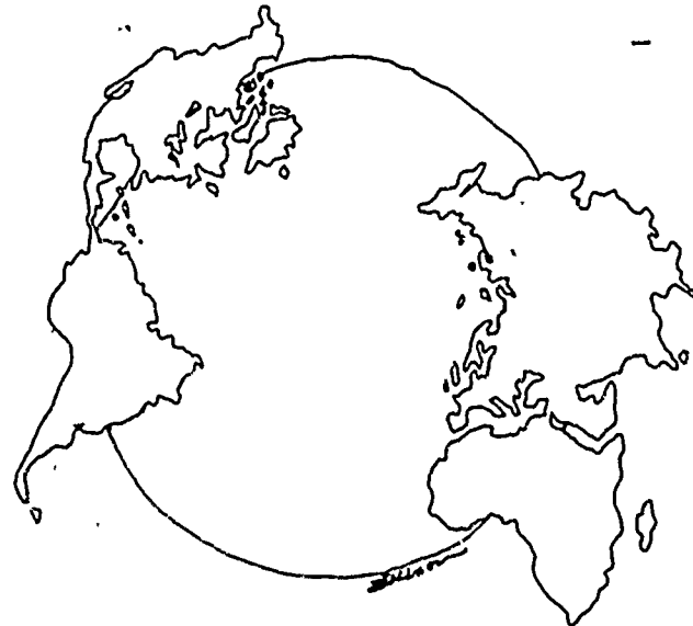
Continental drift.
