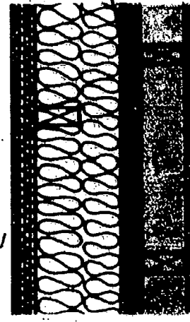
E.F.7. Frame wall, 7" curtain wall plus 1 foil-faced isocyanurate, unfilled cavity R-34 $.15/R/sq.ft.
