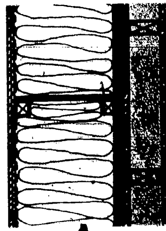
E.F.4. Frame wall, 11" Larsen Truss, unfilled cavity R-37 $.11/R/sq.ft.
