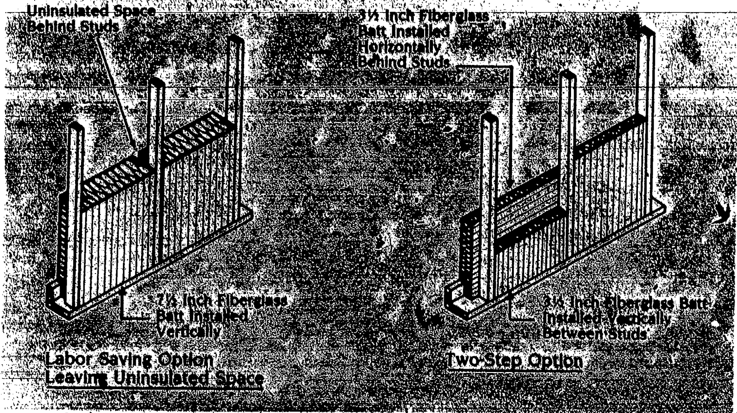
FIGURE 2.5c Insulation techniques for a 7 1/2-inch curtain wall retrofit.
