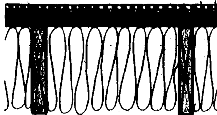
F.2. 9½" fiberglass batts between floor joists R-30 $.06/R/sq.ft.
