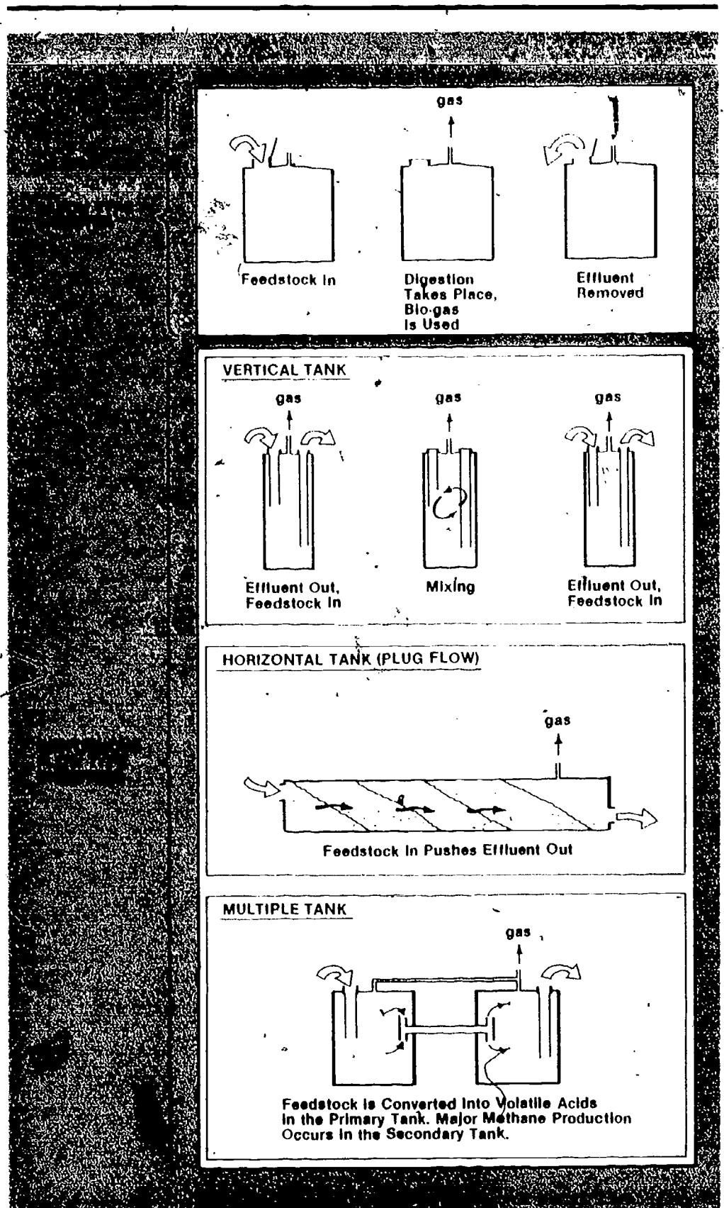
FIGURE 2: Two basic types of digesters can be used for farm-sized biogas production: batch and continuous.
