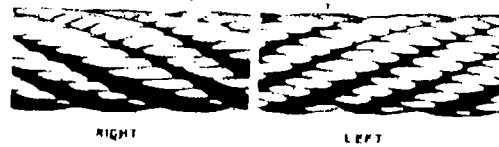
Fig 7-3. Right lay and left lay wire ropes.
