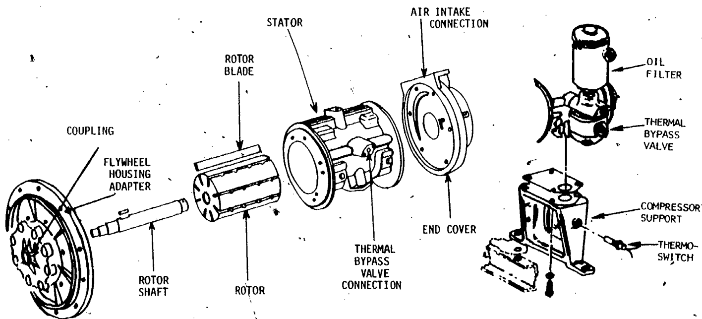
Fig 6-5. Exploded view of the the 250-cfm rotary compressor and thermal bypass valve.
