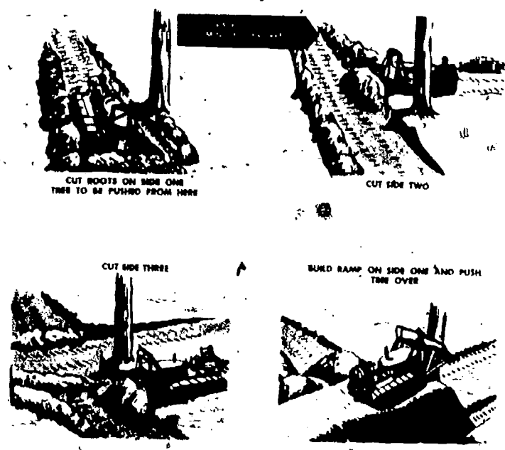
Fig 4-26. Four steps for removing large trees with bulldozer.
