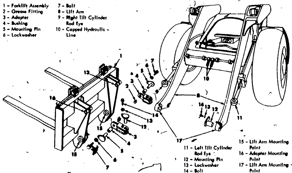
Fig 5-13. Forklift assembly.
