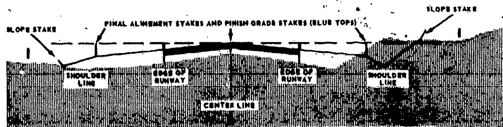
Fig 3-16. Cross section of runway showing stakes and markings.
