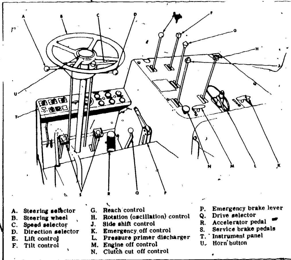
Fig 5-6. Driver's compartment arrangement.
