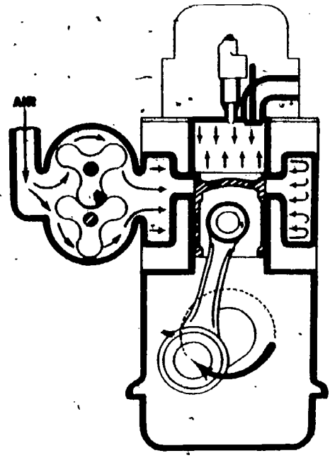
Fig 2-6b. Compression phase of upward stroke of engine piston.
