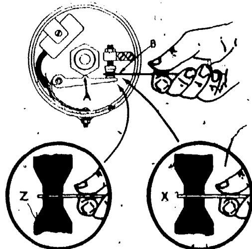
(A) RUBBING BLOCK ON CAM LOBE (B) GAGING THICKNESS BETWEEN CONTACTS (X) CONTACT POINTS IN CONDITION FOR GAGING (Z) CONTACT POINTS BURNED AND FITTED
