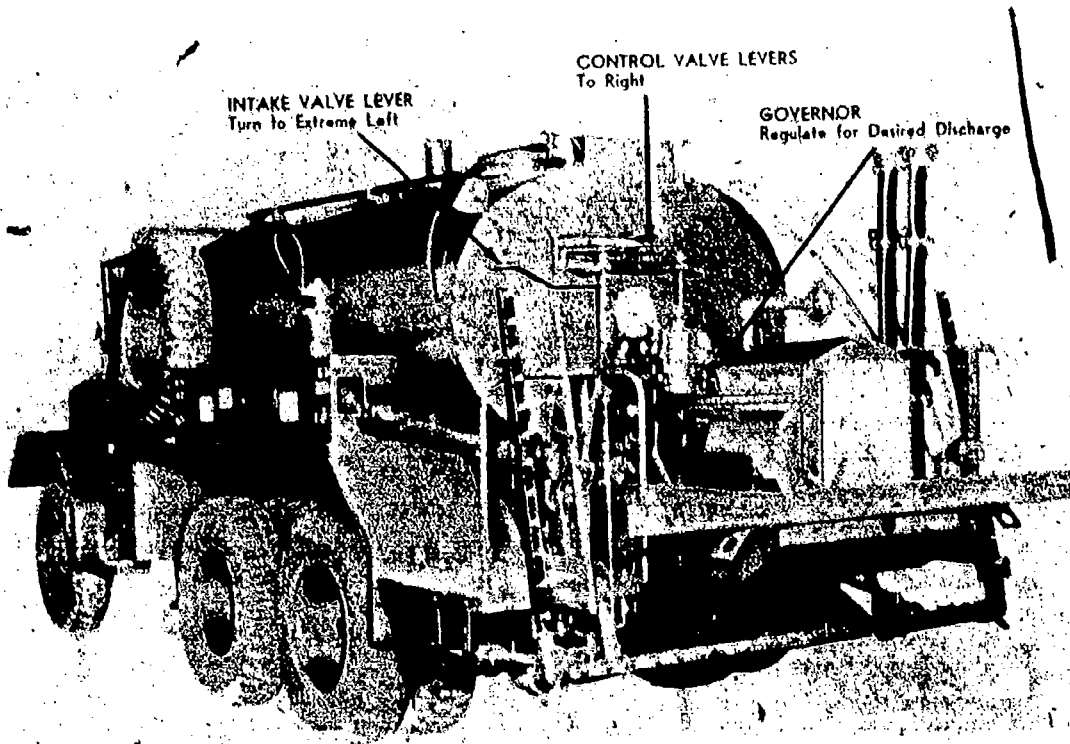
Fig 6-3. Asphalt distributor.
