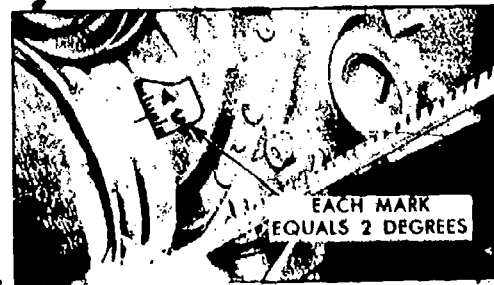
Fig 2-28. Ignition timing marks on flywheel and vibrator damper.
