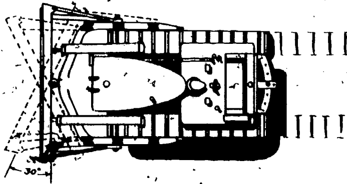
Fig 4-19. Tilting angledozer blade.
