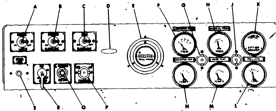
Fig 5-6. Driver's compartment arrangement.
