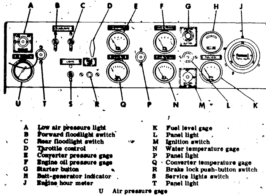
Fig 5-8. Instrument panel arrangement.
