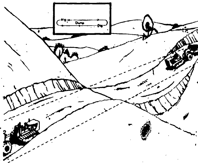
Fig 4-45. Scrapers working two cuts with a common fill between them eliminates a turn on the fill.
