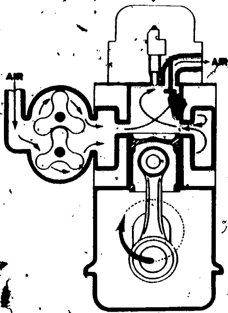
Fig 2-6a. Scavenging phase of upward stroke of engine piston.
