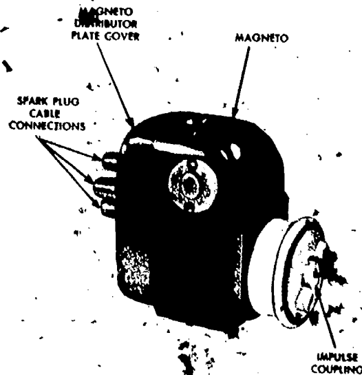
Fig 2-24. Automotive magneto.
