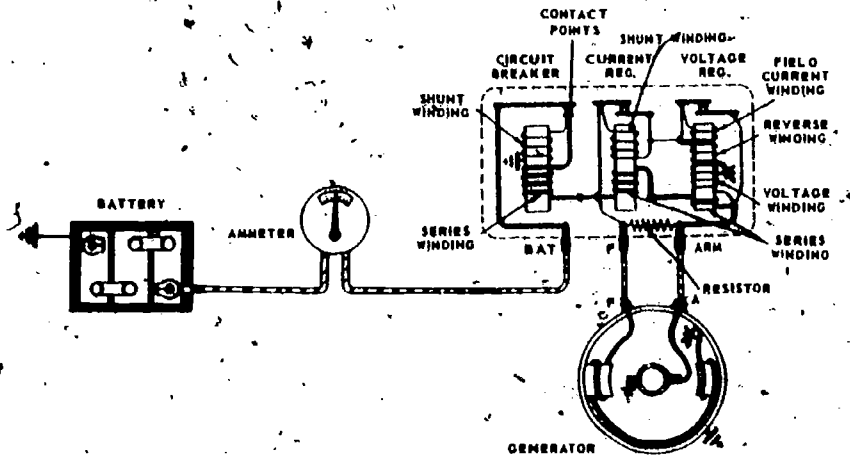
Fig 3-19. Charging circuit.
