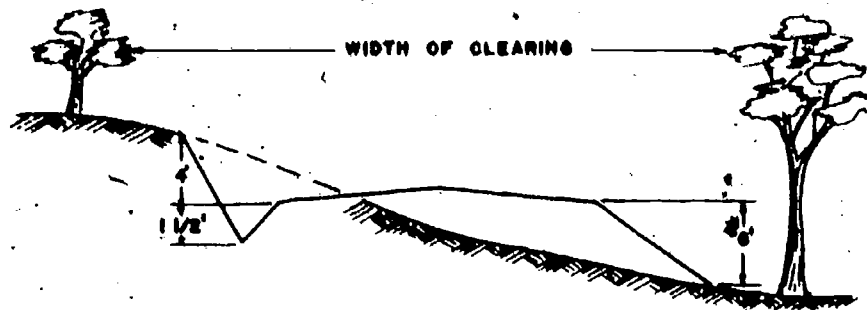
Fig 3-20. Determining width of clearing.
