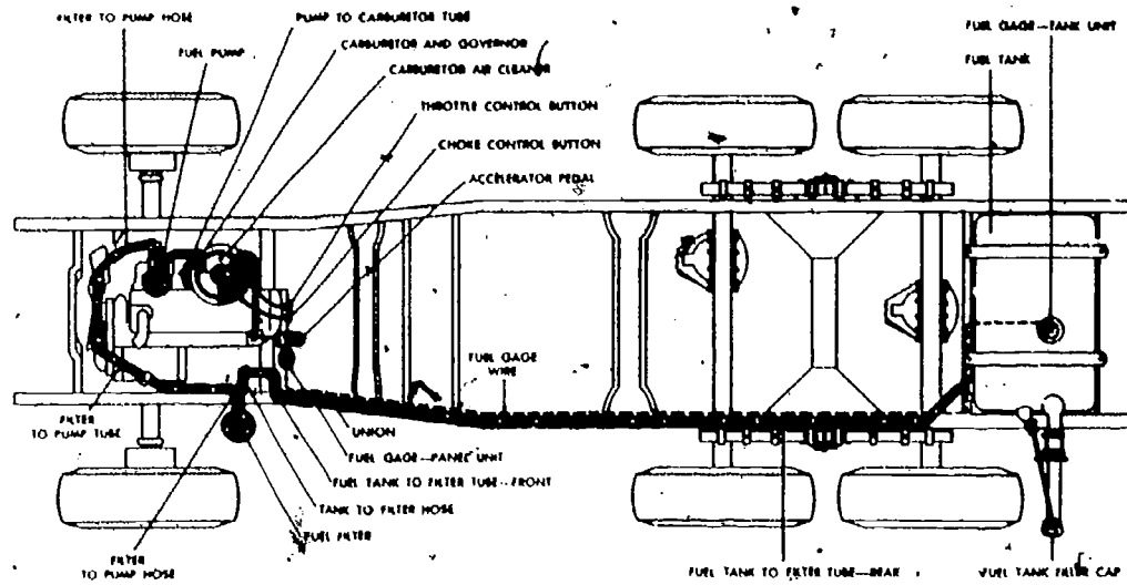
Fig 2-29. Fuel system of the gasoline engine.
