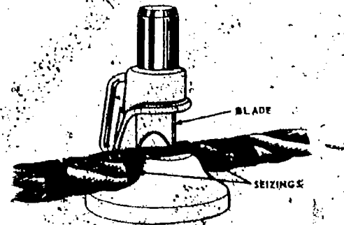
Fig 7-11. Hammer-type wire-rope cutter.
