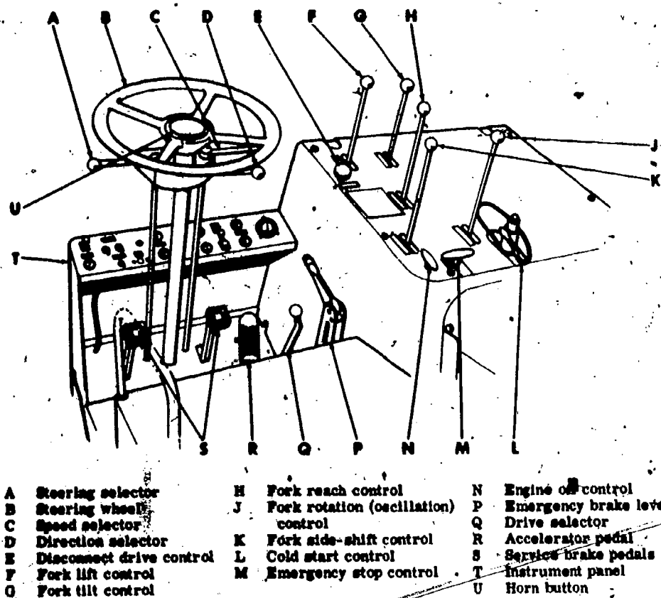
Fig 5-9. Driver's compartment arrangement.
