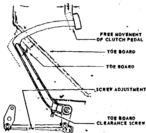
Fig 2-44. Clutch-pedal adjustment.
