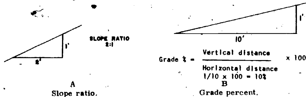
Fig 3-19. Slopes and grades.
