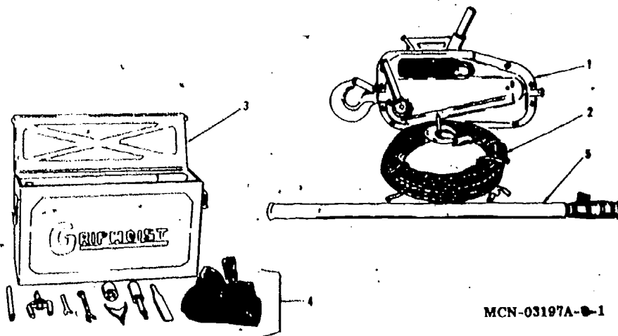
Fig 5-18. Skid assembly, sectionalization.
