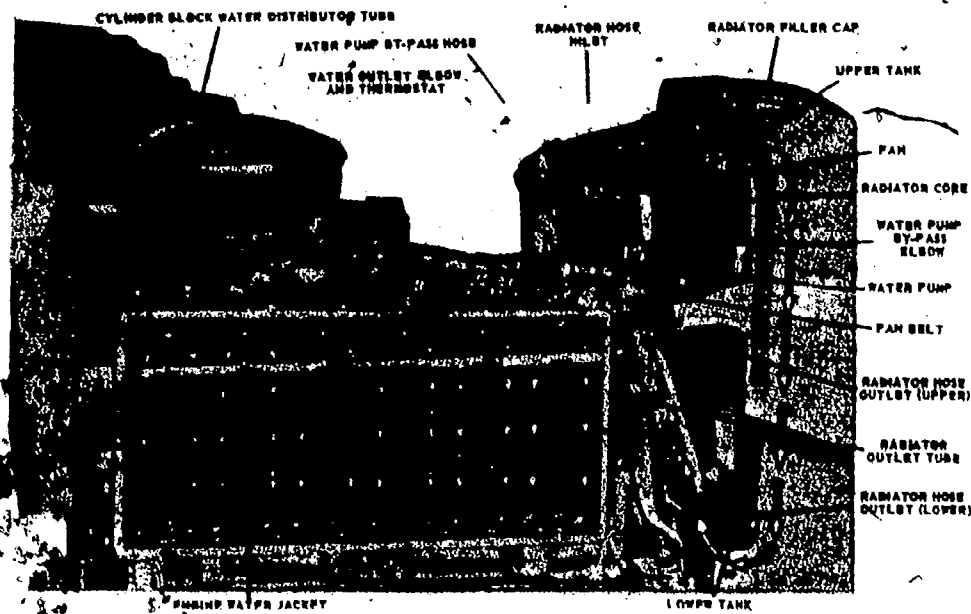
FIG 2-11. Liquid-cooled circulation system.
