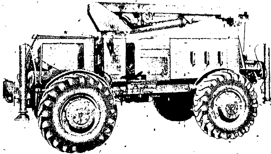
Fig 5-2. 3-ton hydraulic Anthony crane.
