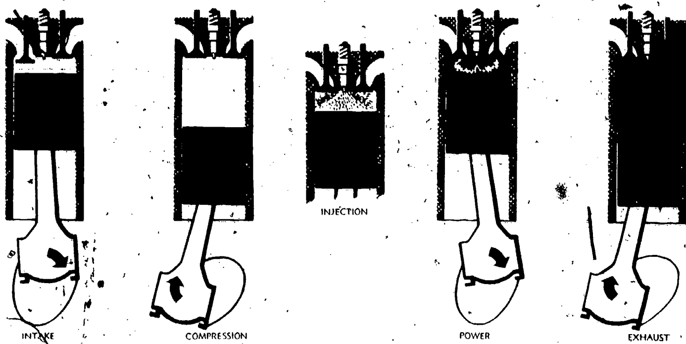
Fig 2-4. 4-stroke-cycle diesel engine.
