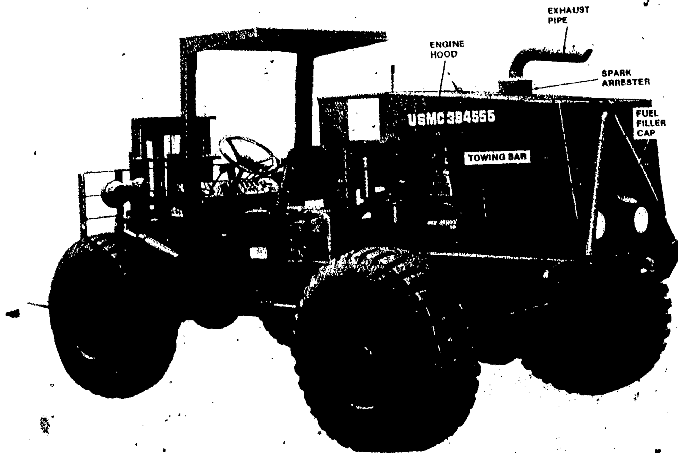
Fig 5-1. Case MC 4000 rough-terrain forklift.
