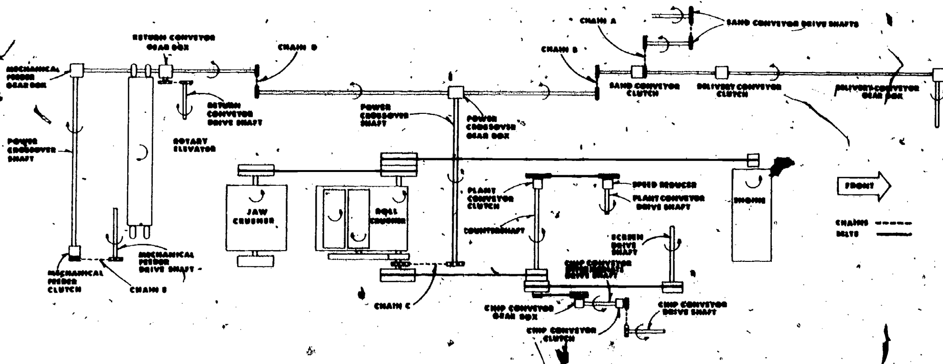
Fig 6-13. Model 101-S secondary plant--power flow diagram.
