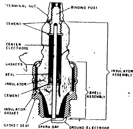
Fig 2-26. Sectional view of a typical spark plug.
