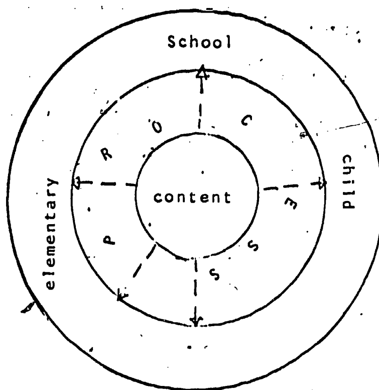
FIGURE 1 - PROCESS/CONTENT RELATIONSHIP
