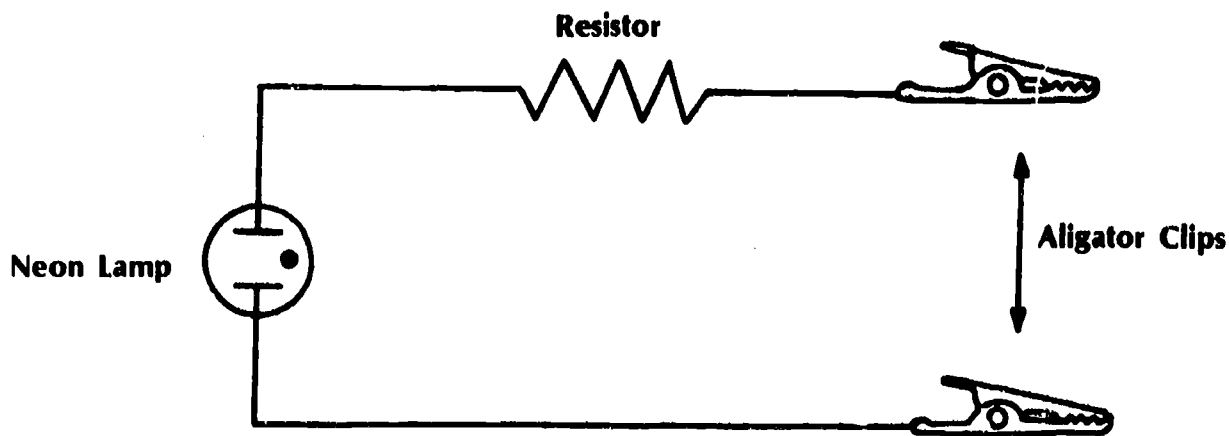
Schematic Diagram
