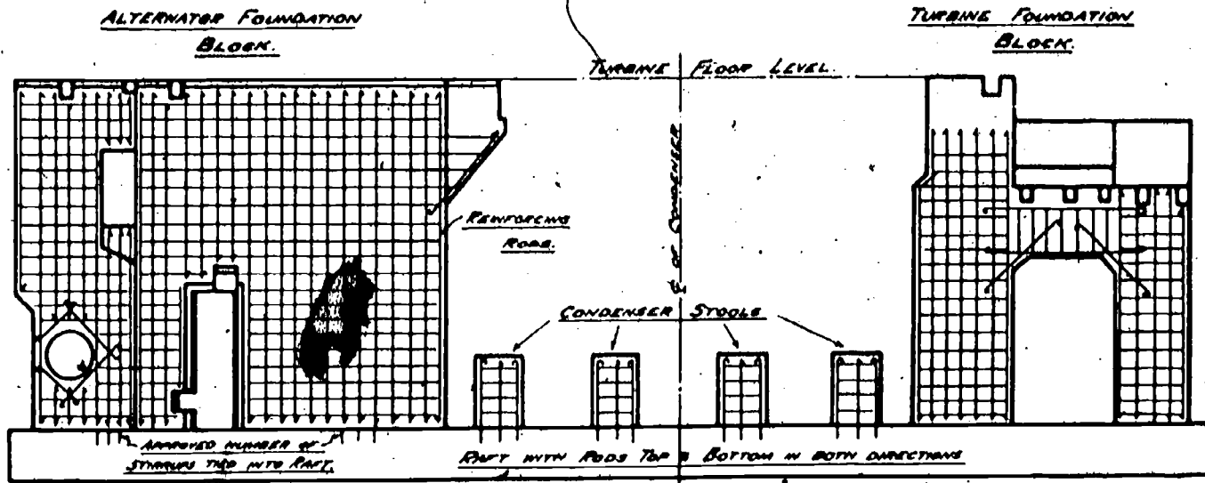
Elevation of TYPICAL TURBO-ALTERNATOR FOUNDATION BLOCK
