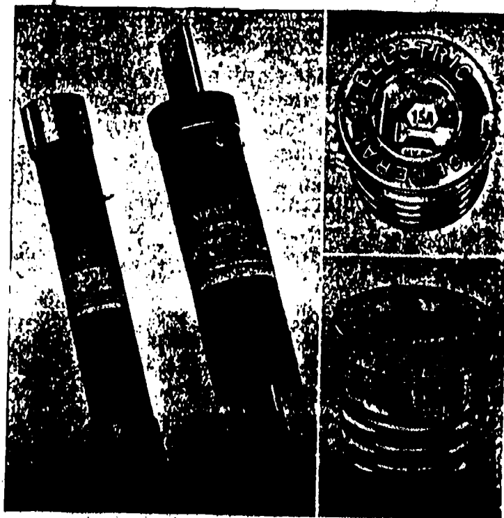
Some representative types of plug and cartridge fuses
