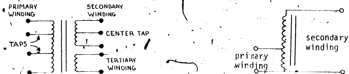
MULTI-TAP TRANSFORMER WITH TERTIARY WINDING
