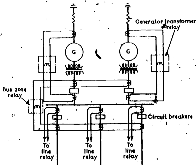
Locations of Current Transformers to provide overlapping zones of protection Fig. 18
