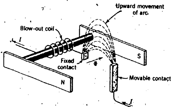
Operation of the Magnetic Blow-out Fig. 5
