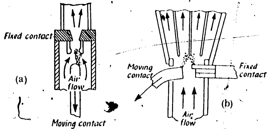
Types of Air-blast Circuit-breakers
