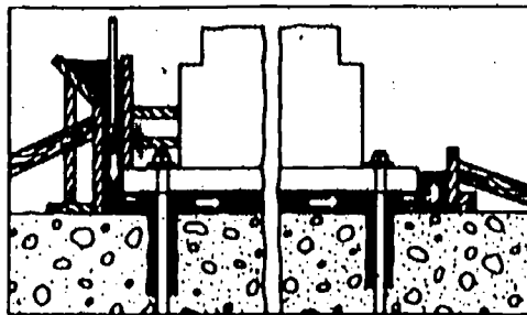
WELL and PLUNGER PRESSURE GROUTING for SOLID WIDE BEDPLATES
