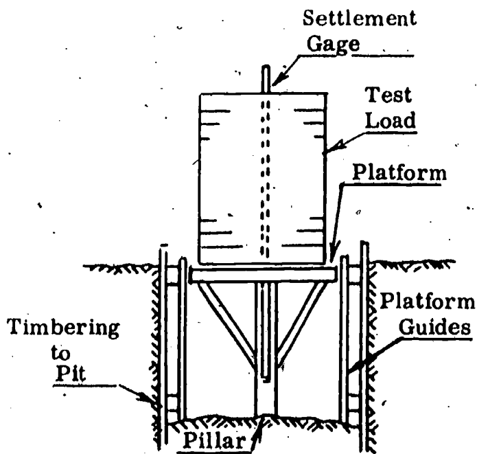
Test for Bearing Value of Ground Fig. 1
