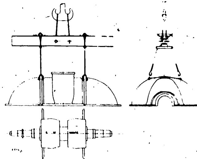
Arrangement for lifting L-p cylinder, centre and exhaust covers
