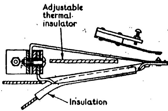
Single-phase Unimetallic Strip Thermal Relay Fig. 25
