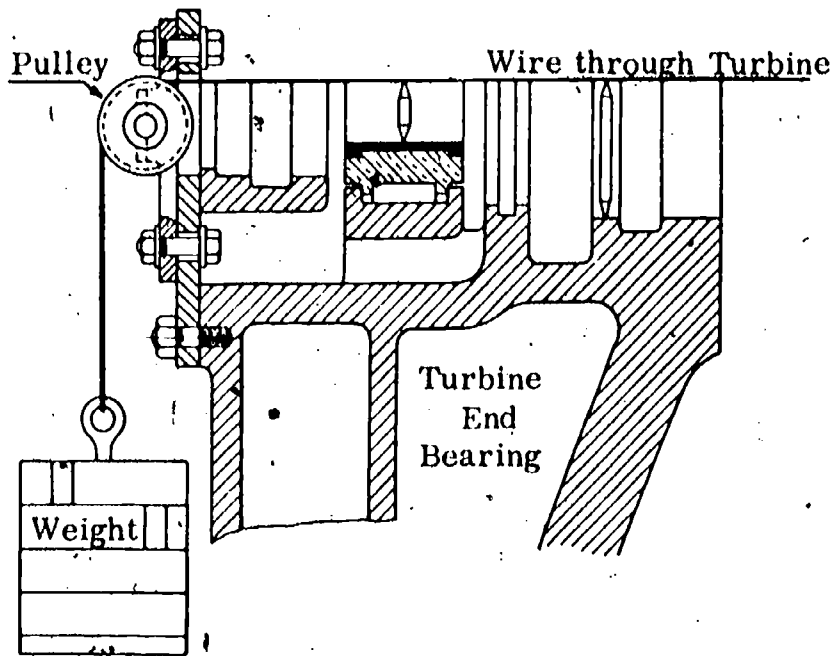
STRETCHED WIRE METHOD OF ALIGNING BEARINGS AND GLAND BORES
