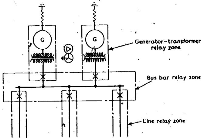
Zones of Protection overlapping to avoid blind spots Fig. 17
