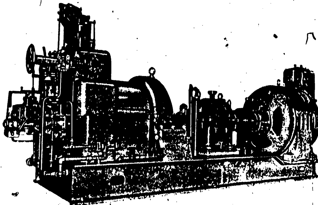
GEARED TURBO-GENERATOR UNIT with automatic steam control valve gear and generator having a belted exciter. This 300 kW unit operates with 1700 kPa steam, 263°C and exhausts to 10 kPa condenser pressure.
