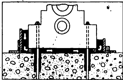
GRAVITY GROUTING plus RODDING and WORKING
