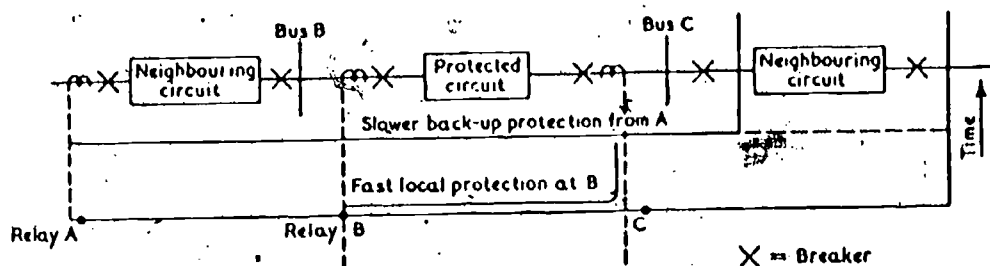
Back-up Relays Fig. 20
