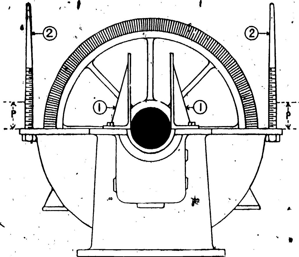
END VIEW OF TURBINE WITH COVER LIFTED
