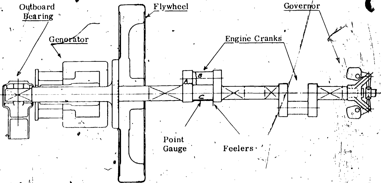
LINING OUT ENGINES AND SINGLE BEARING GENERATORS OR COMPRESSORS WITH SINGLE BEARING MOTORS
