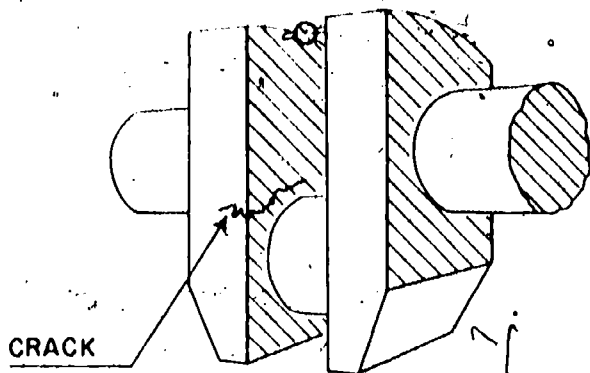
Fig. 14 showing TYPICAL FATIGUE CRACK
