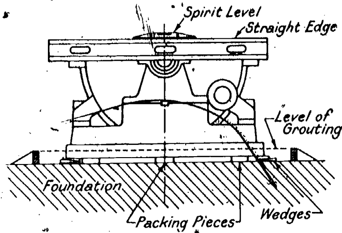
END VIEW OF TURBINE DURING ERECTION
