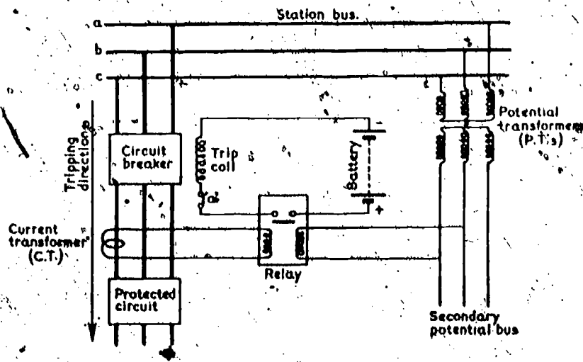
Basic Connections of a Protective Relay
