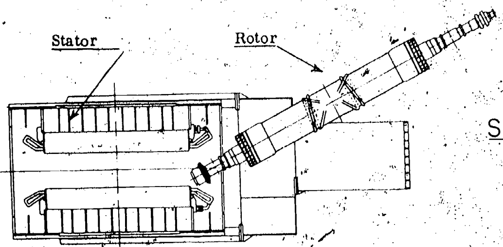
(1) - Plan View -
