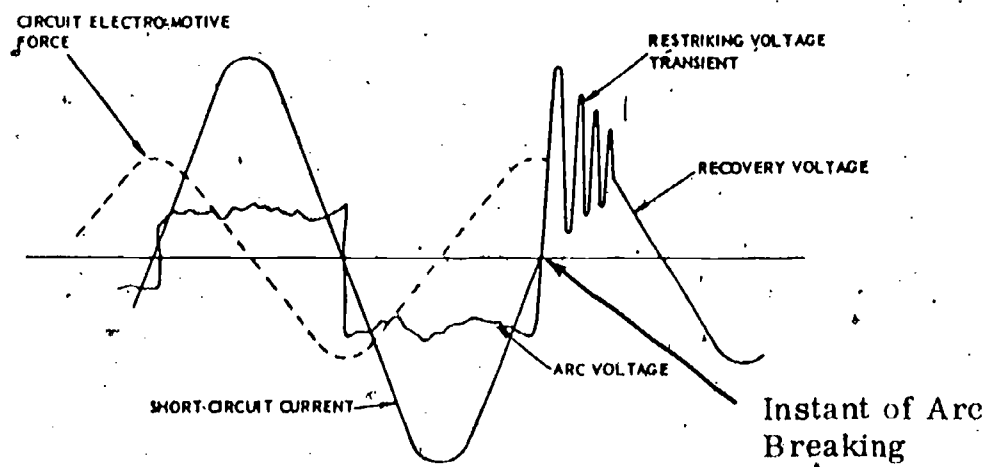
Restriking Voltage Transient Fig. 8
