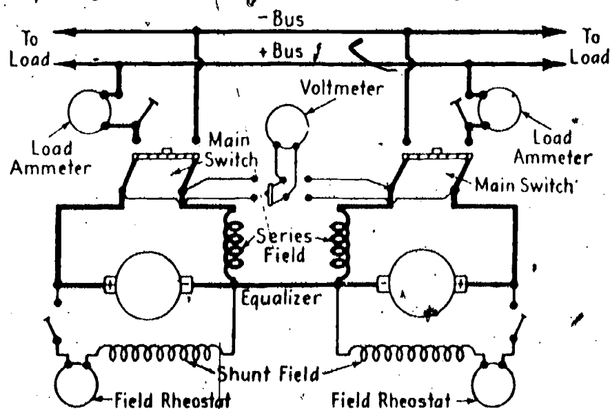
PARALLEL CONNECTION OF COMPOUND GENERATORS SHOWING USE OF EQUALIZER BAR
