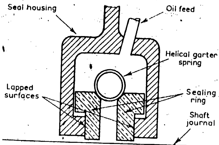
(a) Radial Clearance Type
