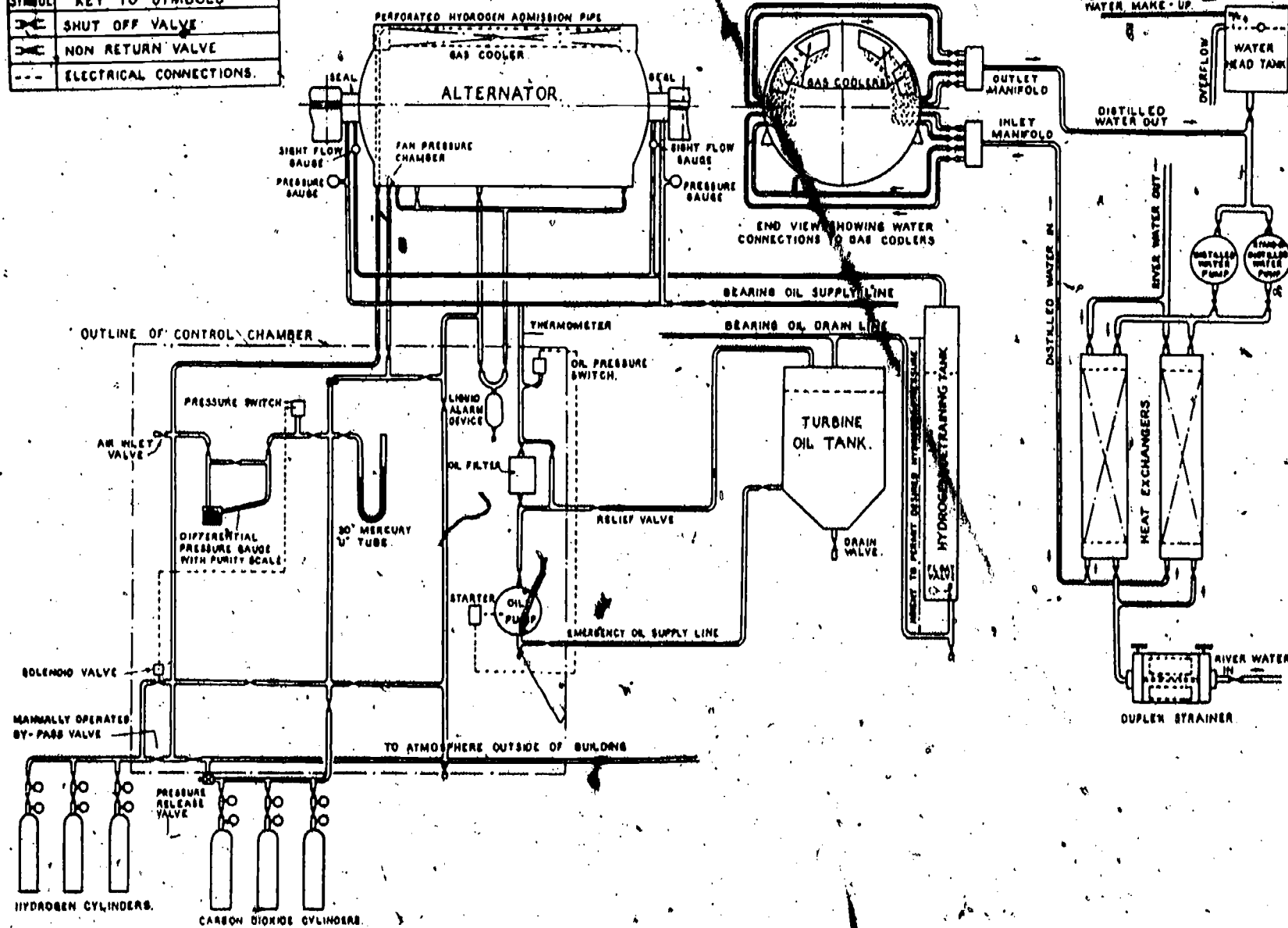
COMPLETE SYSTEM OF PIPEWORK AND AUXILIARIES FOR HYDROGEN-COOLED ALTERNATOR
