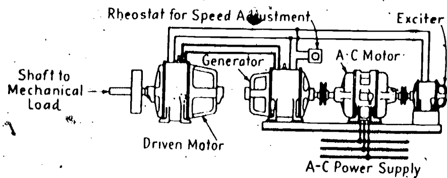
WARD LEONARD METHOD OF CONTROL
