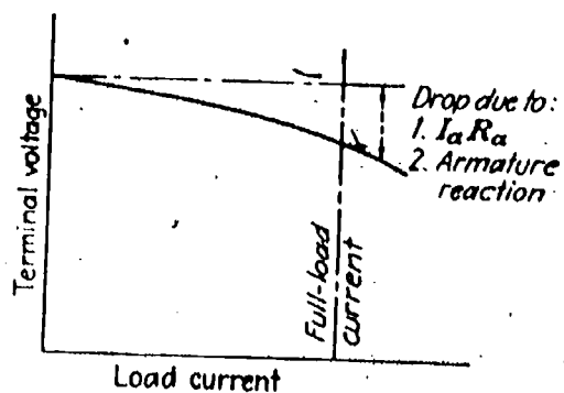
Voltage Regulation Curve
