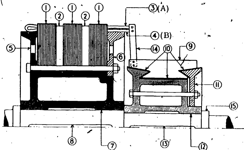
SECTION THROUGH ARMATURE AND COMMUTATOR FOR D-C GENERATOR
