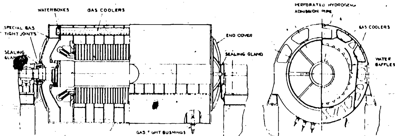
ARRANGEMENT OF HYDROGEN-COOLED ALTERNATOR Fig. 8
