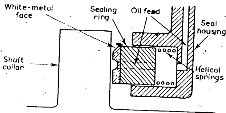
(b) Axial Clearance Type
