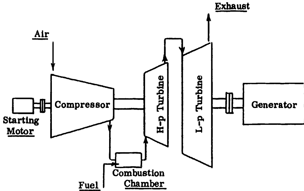
OPEN CYCLE GAS TURBINE with DUAL SHAFT
