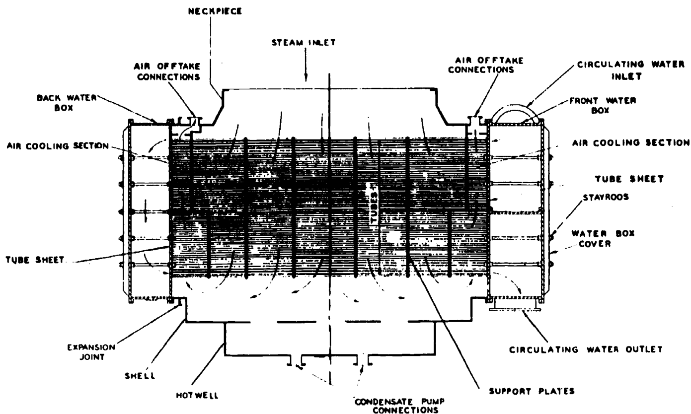
Surface Condenser
