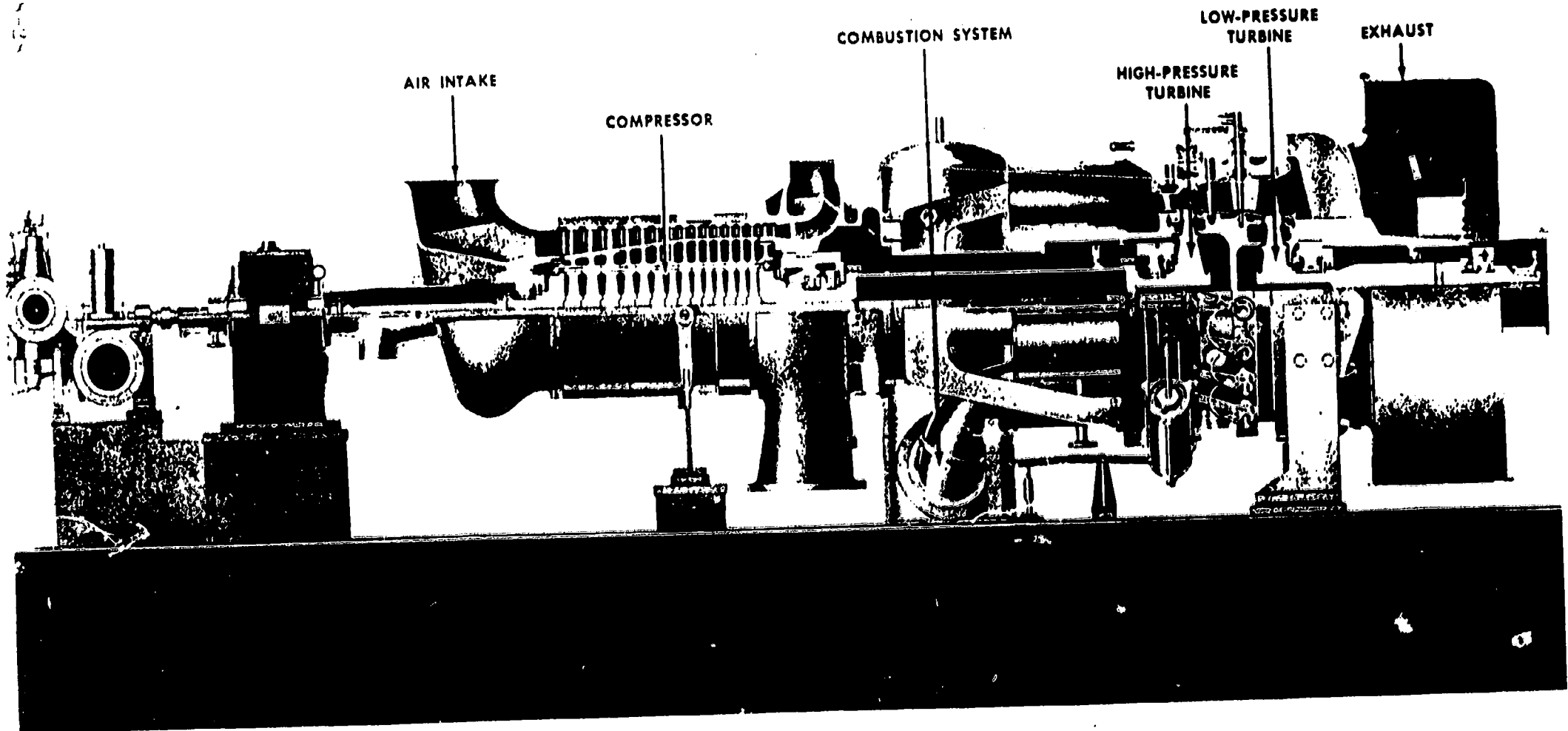
GENERAL ELECTRIC GAS TURBINE with REGENERATOR
