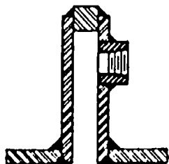
Detail of Condenser Shell Expansion Joint
