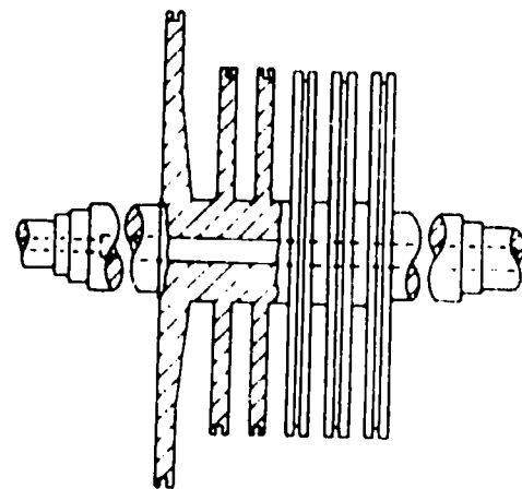
Solid Forged Disc Rotor
