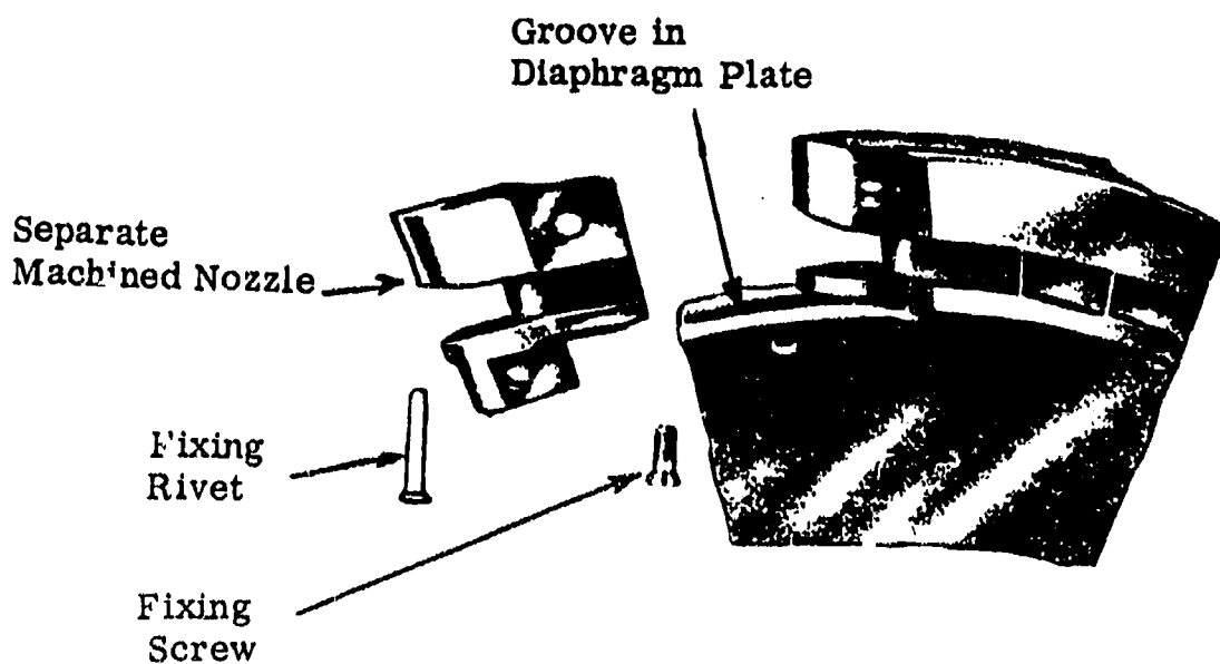
Built-up Diaphragm
