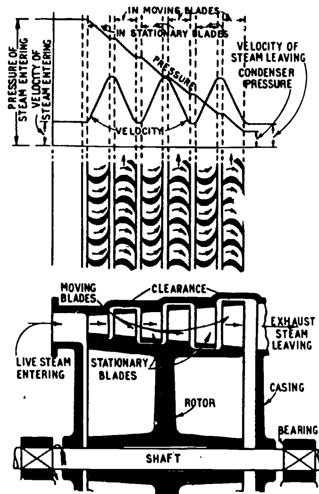
Simple Reaction Turbine
