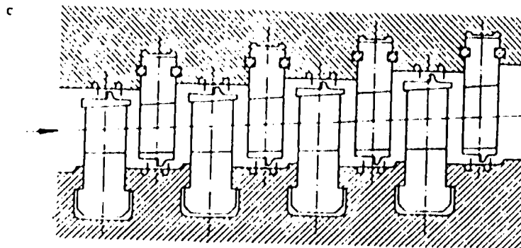
Drum-type rotor with tip-sealed blades Fig. 38
