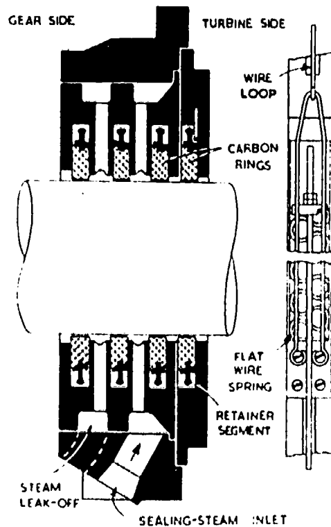
Carbon Ring Shaft Seal Fig. 24
