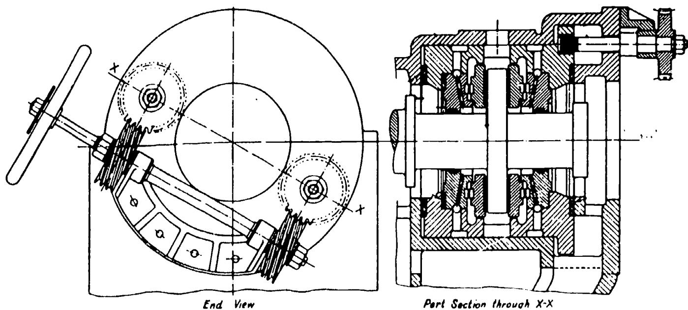
Thrust Adjusting Gear for Reaction Turbine
