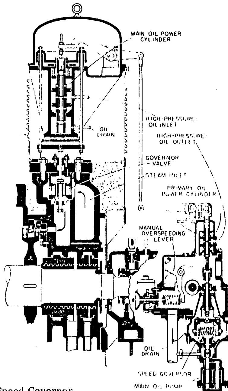
Speed Governor with Double Relay Hydraulic System
