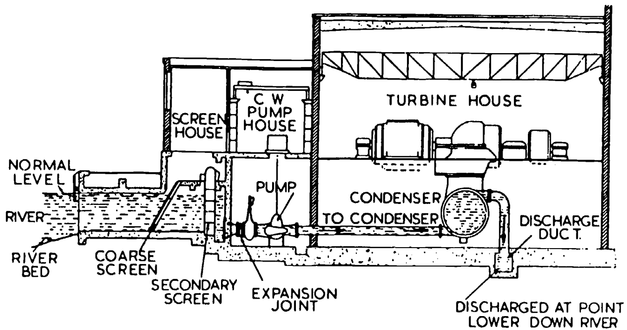
Condenser using Cooling Water from River
