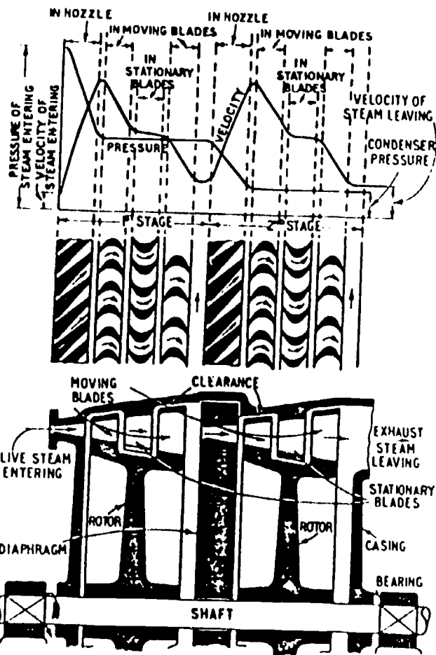
Pressure-Velocity Compounded Impulse Turbine
