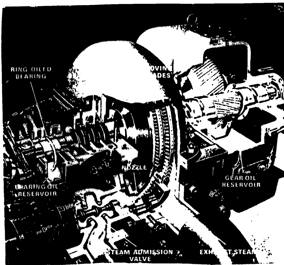
Cutaway Section of a small Turbine Fig. 42
