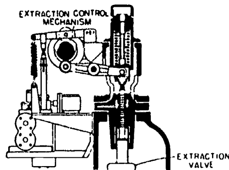
Grid-type Extraction Valve Fig. 34
