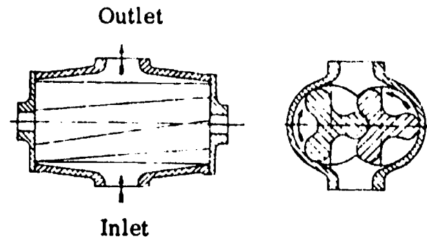
ROOTS COMPRESSOR
