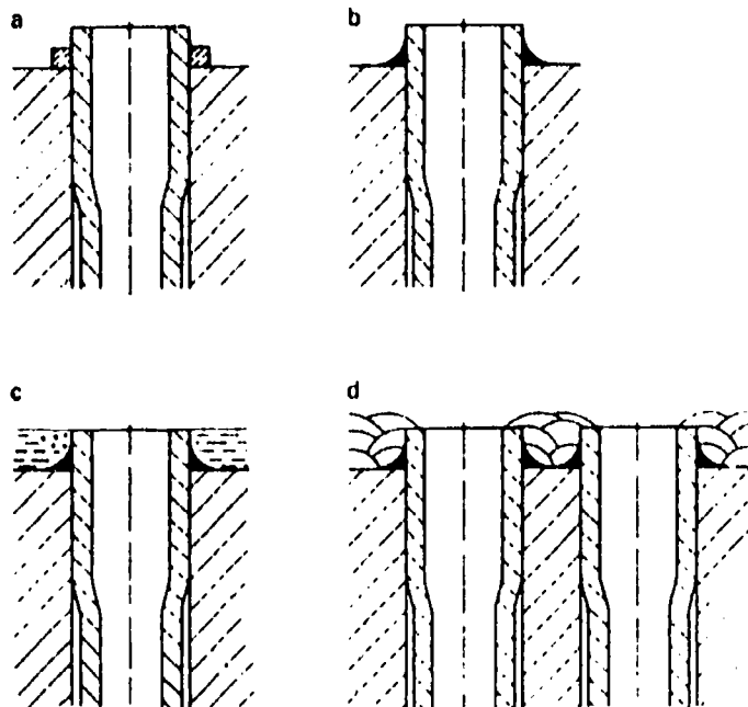
Stages of tube welding process
