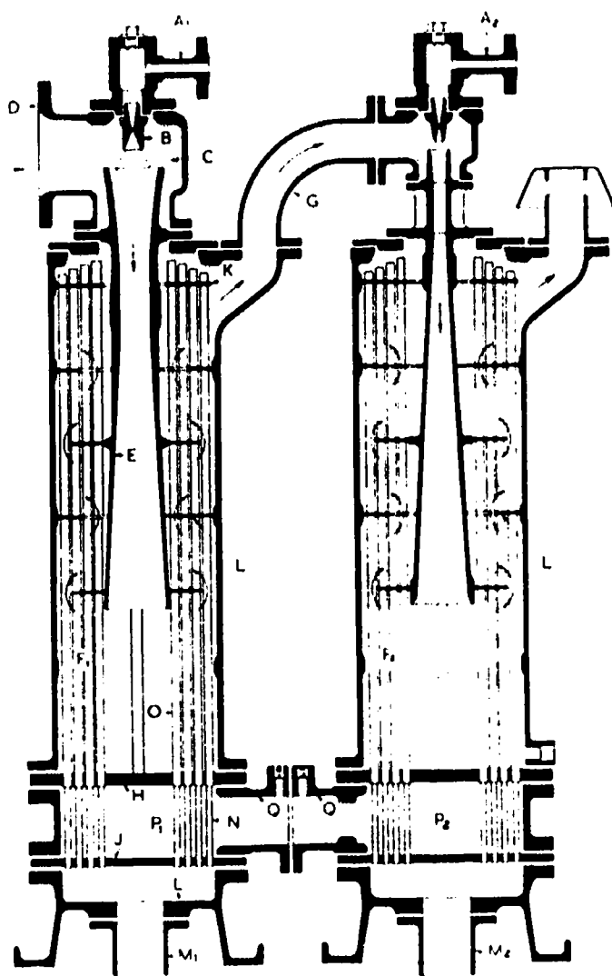
Section of a two-stage air ejector with inter and after surface coolers.
