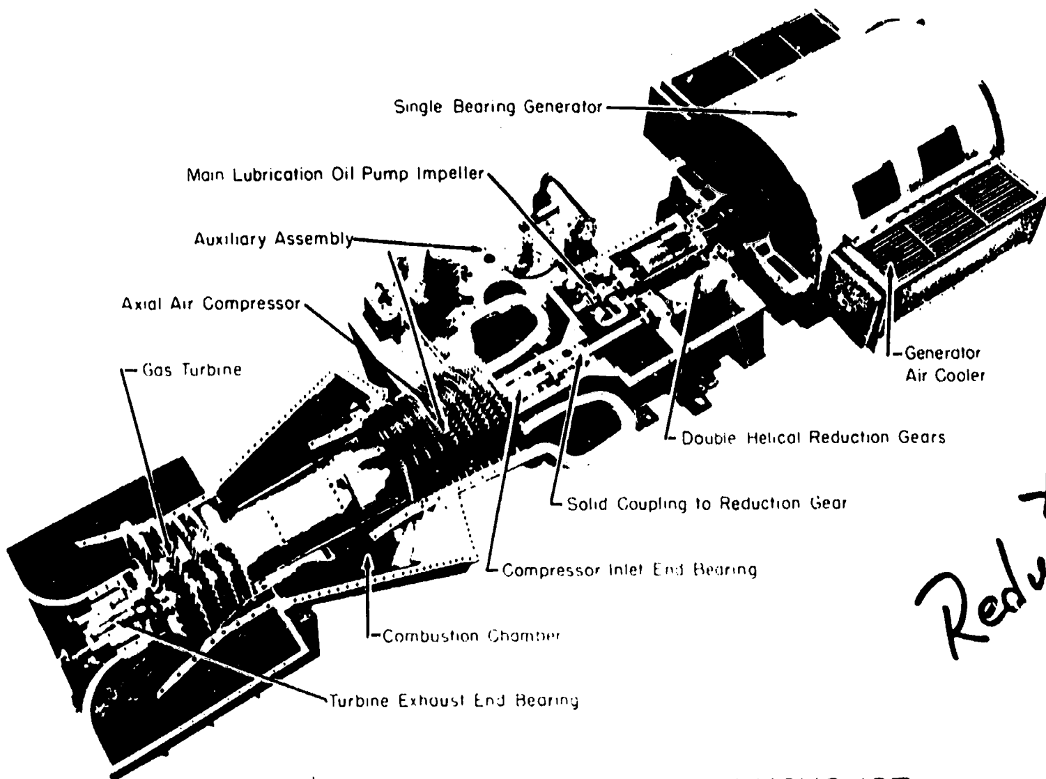
5000 kW CANADIAN WESTINGHOUSE GAS TURBINE Fig.27
