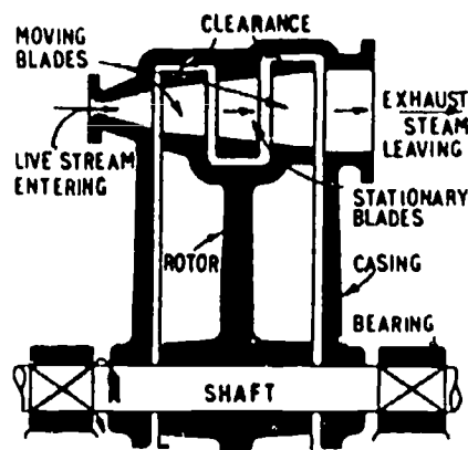
Velocity Compounded Impulse Turbine
