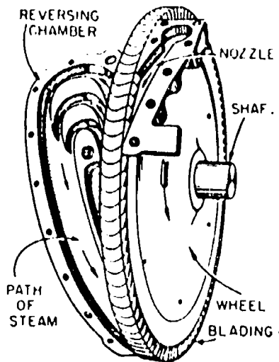
Re-entry Method of Velocity Compounding
