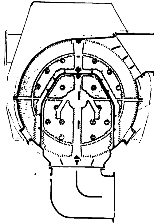
Central Flow Condenser
