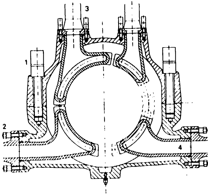
Cross-section through a valve casing with four valves and the wheel-chamber of an industrial turbine.
