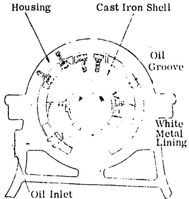
Main Bearing Fig. 44
