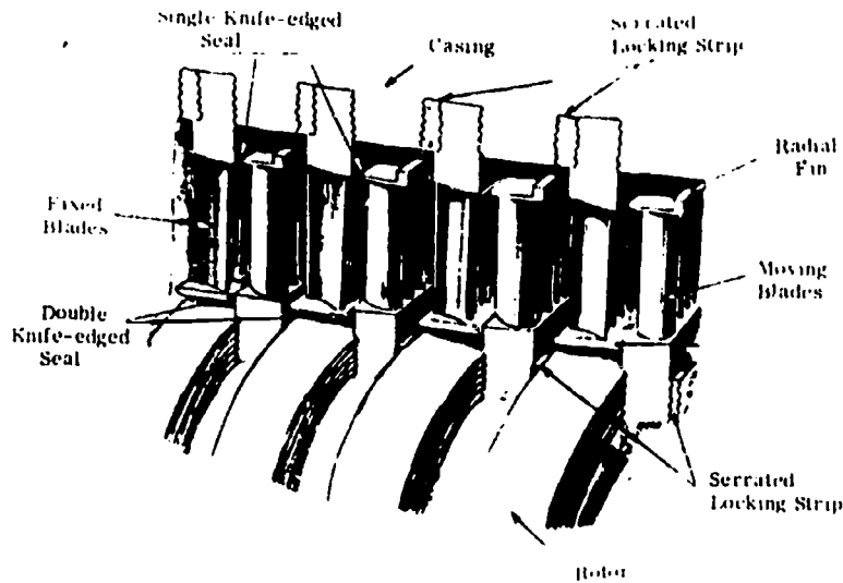
H-p Reaction Type Blading showing End Tightening Fig. 19
