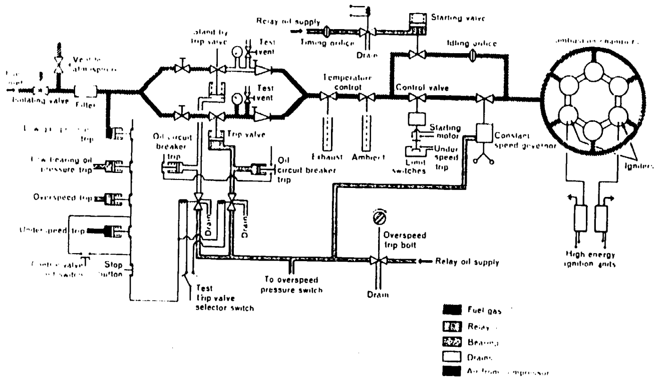
FUEL SYSTEM for A.E.I. GAS TURBINE -DIAGRAMMATIC ARRANGEMENT- Fig.31
