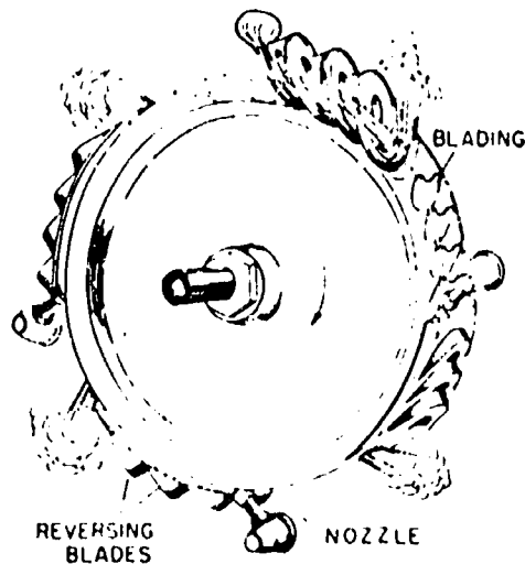
Another Method of Re-entry Velocity Compounding
