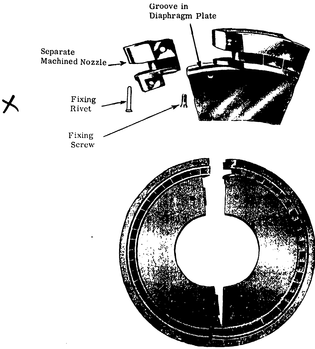
Built-up Diaphragm Fig. 22
