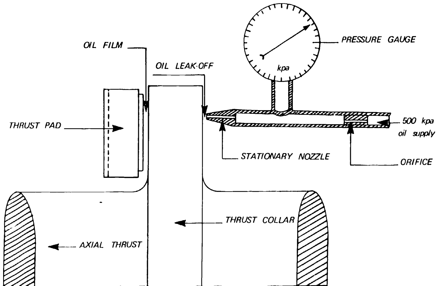
Thrust Collar Position Indicator
