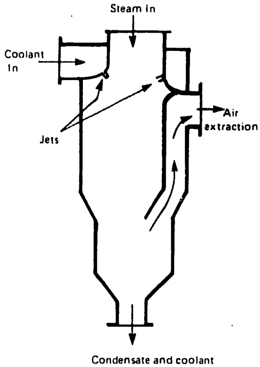
Jet Condenser
