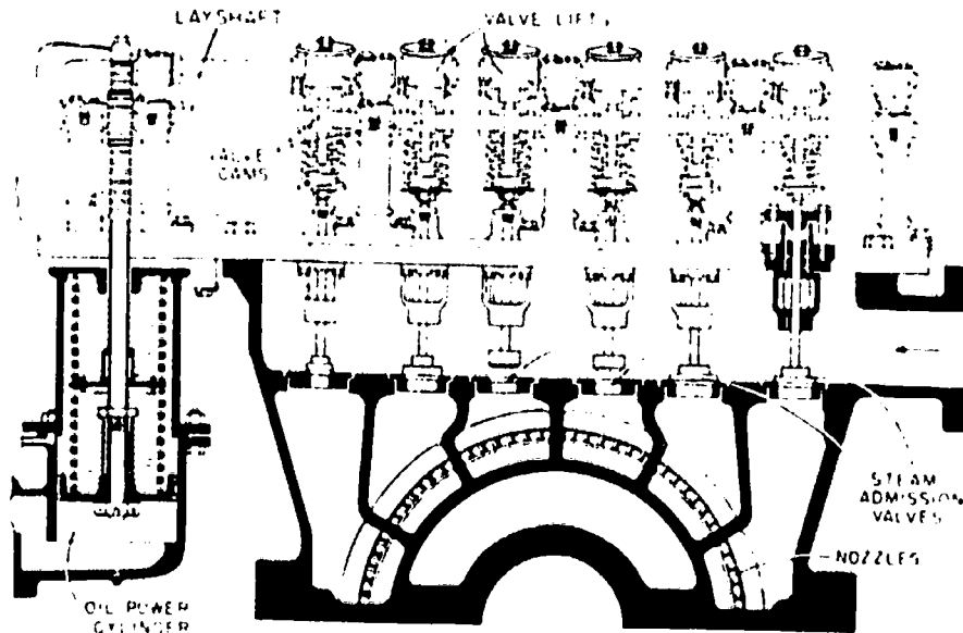
Cam-lift Steam Admission Valves Fig. 33
