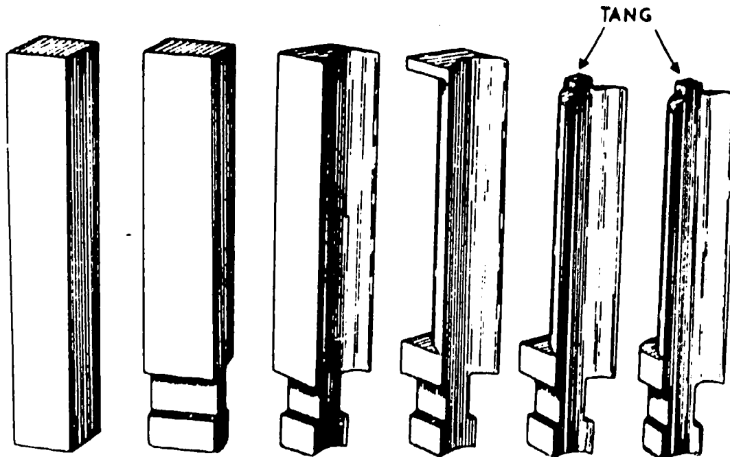
Stages in the manufacture of H-p Impulse Type Moving Blades Fig. 21
