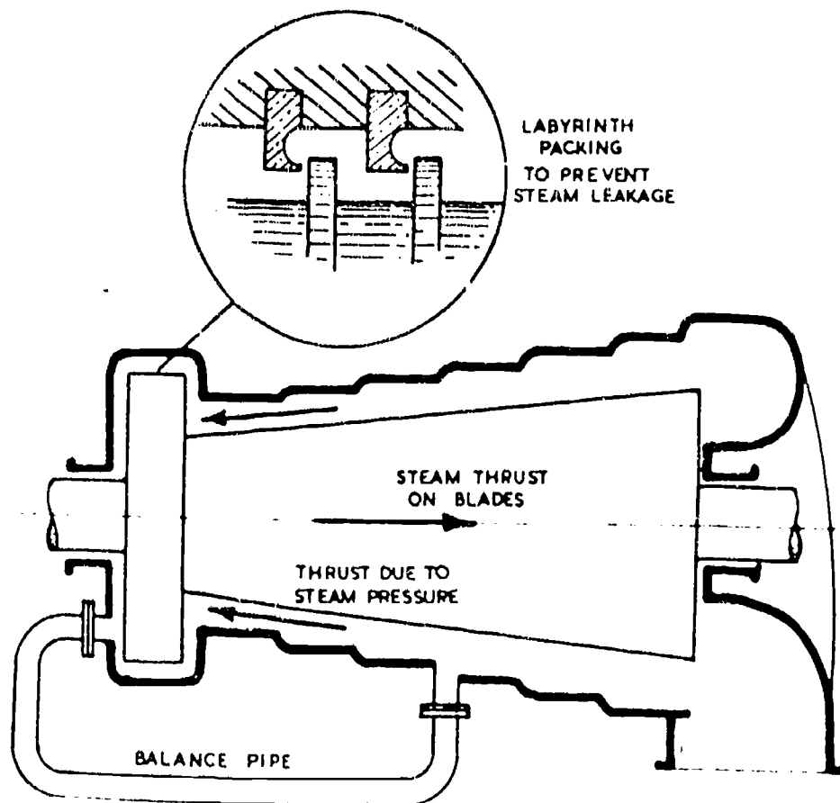
Dummy Piston and Balance Pipe
