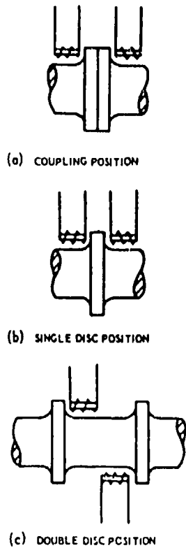
Arrangements of Axial Expansion Detector
