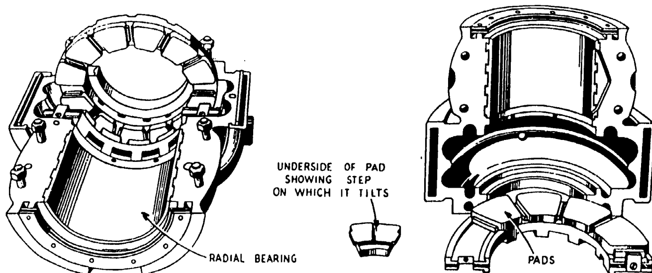
Combined Radial and Michell Thrust Bearing Fig. 41
