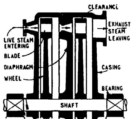
Pressure Compounded Impulse Turbine
