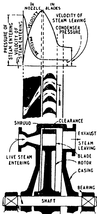
Simple Impulse Turbine
