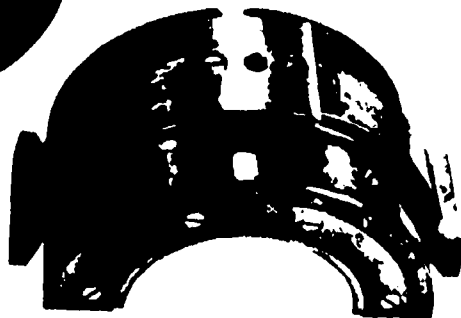
Babbitt-lined Journal Bearing
