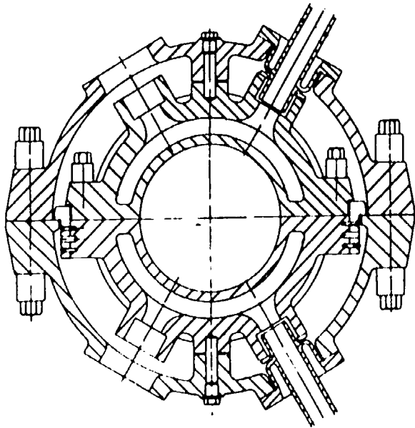
Cross-section through Double-shell Hp Turbine
