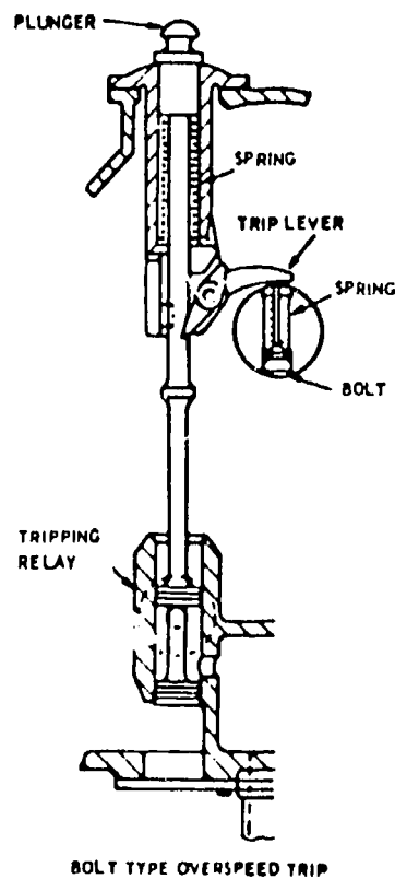
Emergency Trip Gear Fig. 1
