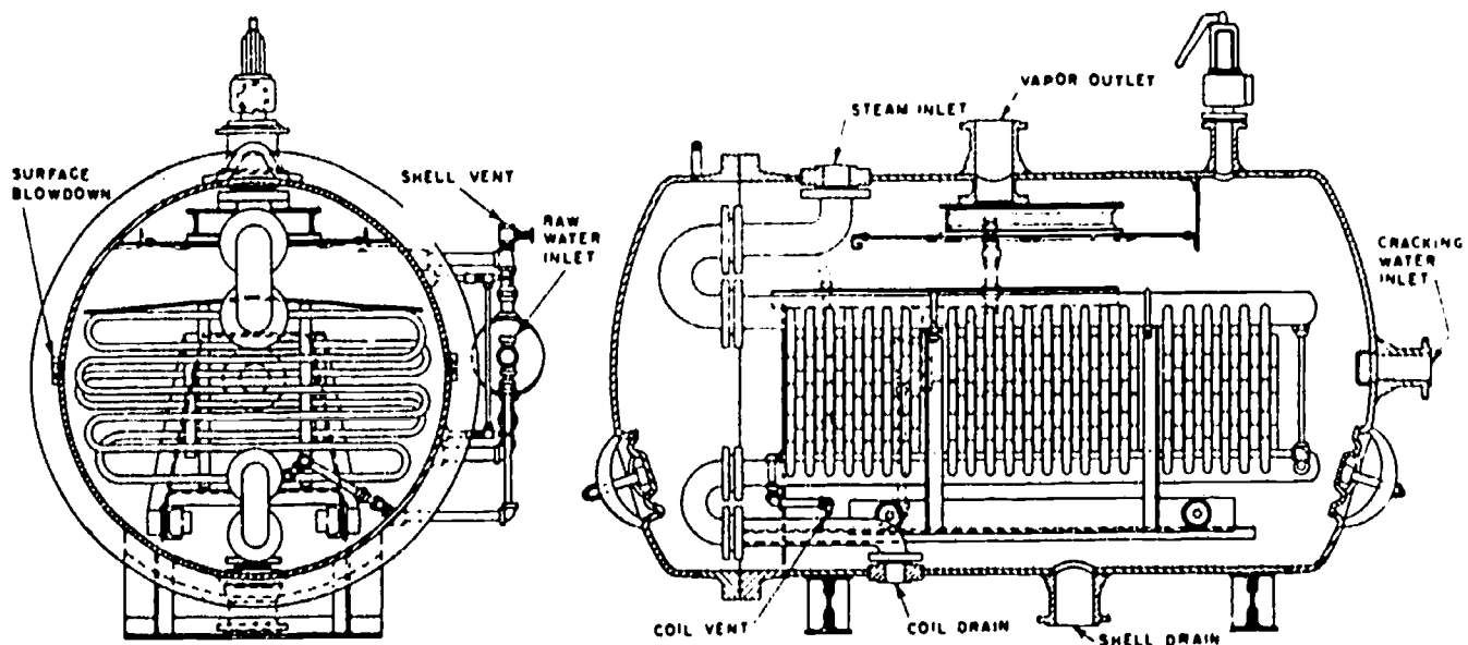
Submerged-coil Evaporator ( Foster Wheeler Corp.)
