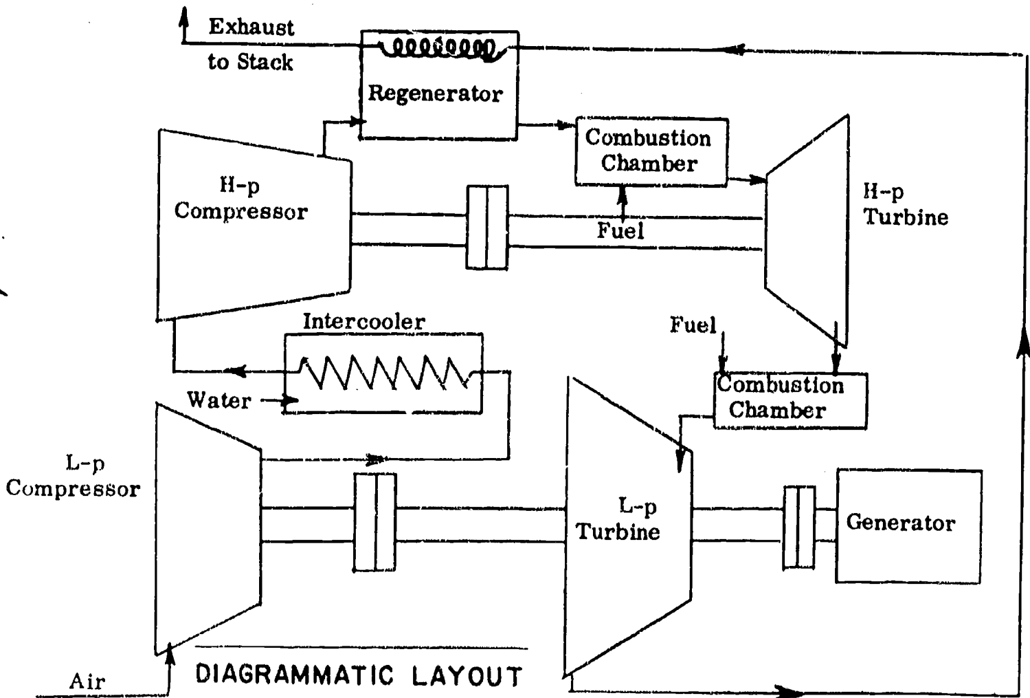
OPEN CYCLE GAS TURBINE with REGENERATOR, INTERCOOLER and REHEATER
