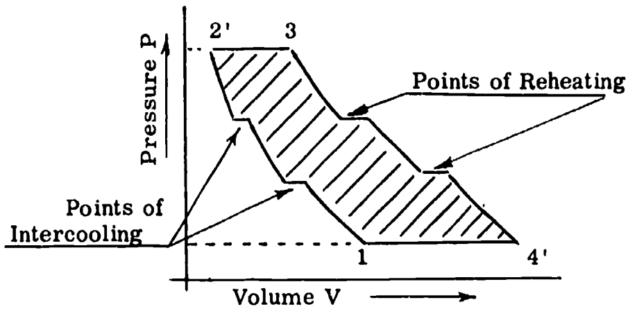
P-V DIAGRAM showing EFFECT OF INTERCOOLING and REHEATING
