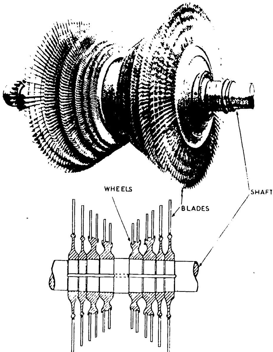
SECTION THROUGH DISC TYPE ROTOR
