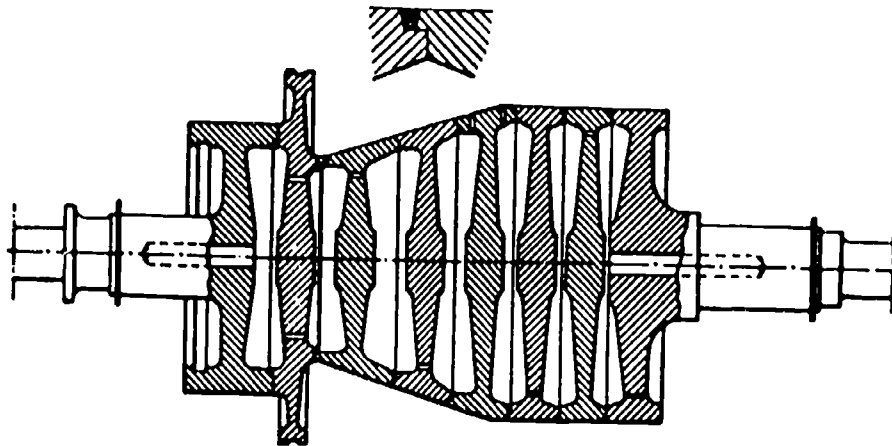
Brown-Boveri Welded Turbine Rotor
