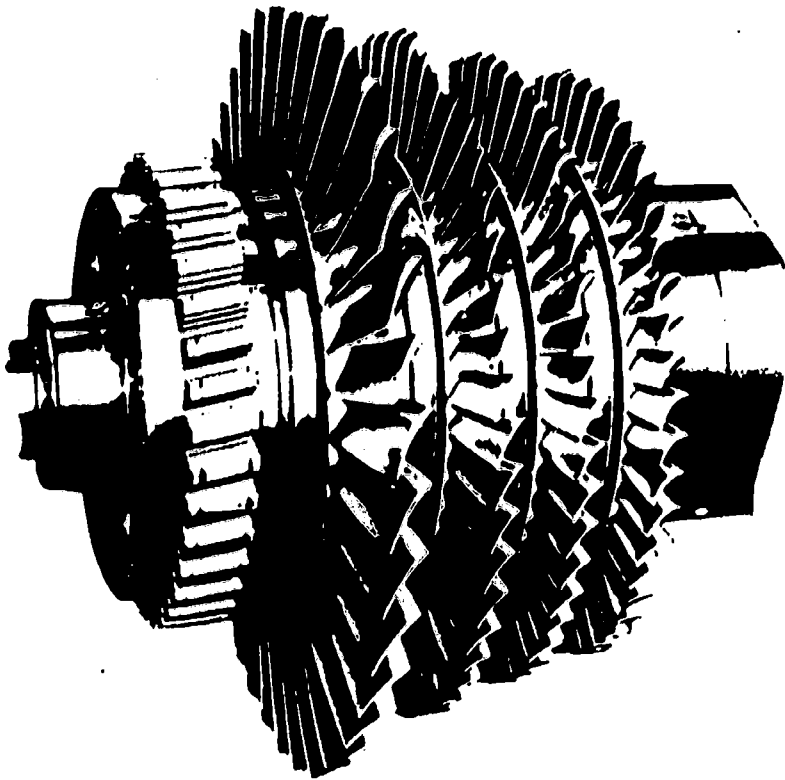
Last row of blades has not been inserted. (a)
