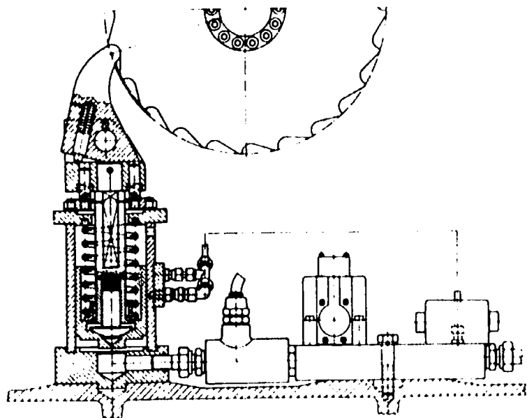
Hydraulic Turning Gear
