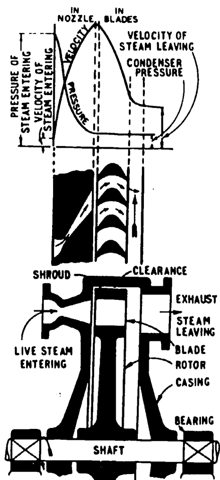
Simple Impulse Turbine
