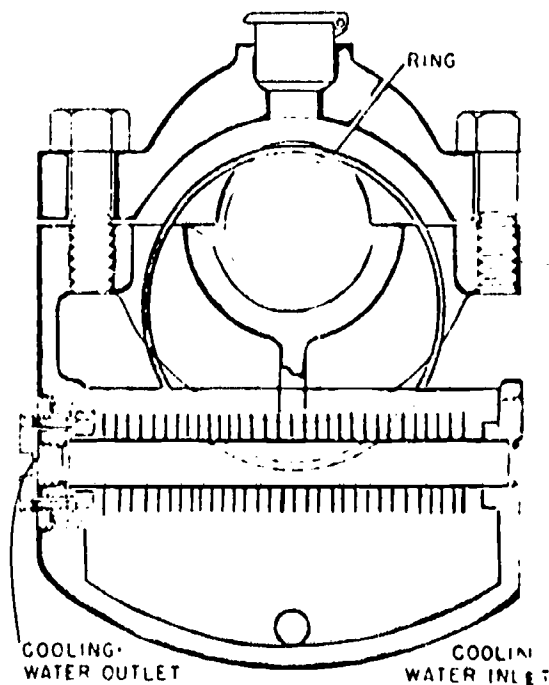
Ring-Oiled Bearing Fig. 43
