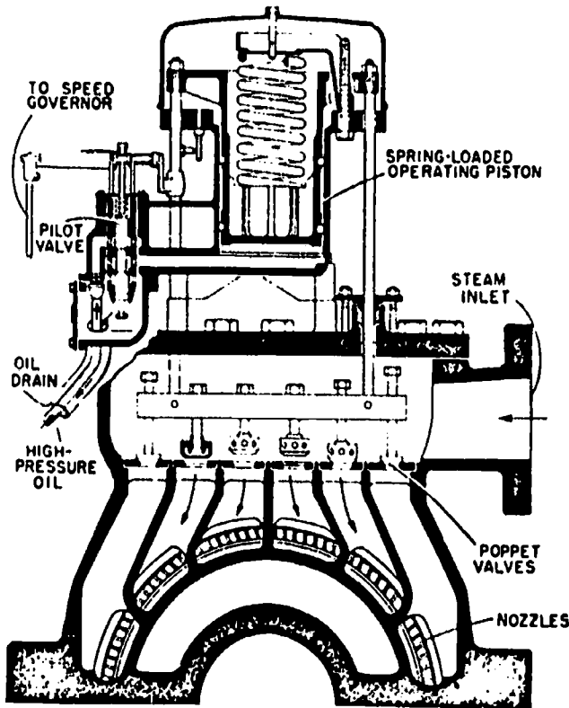
Bar-lift Steam Admission Valves Fig. 32
