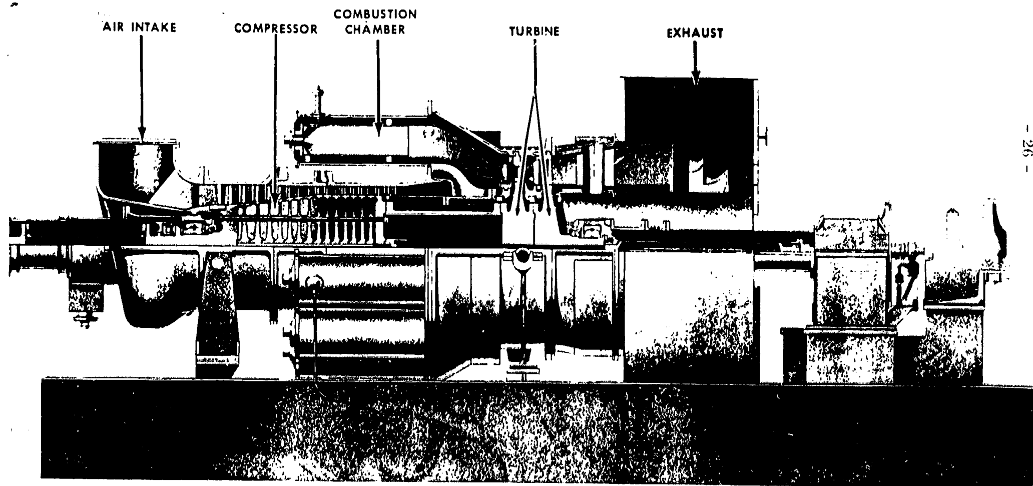
9,500 kW GENERAL ELECTRIC GAS TURBINE
