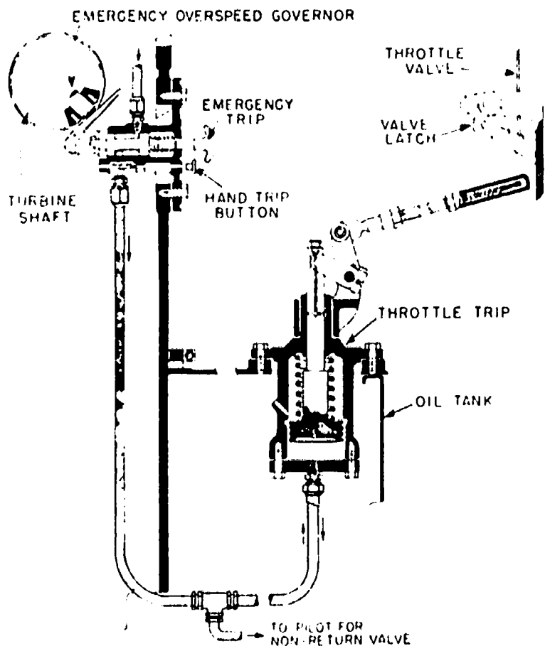
Hydraulic Emergency Overspeed Governor Fig. 29
