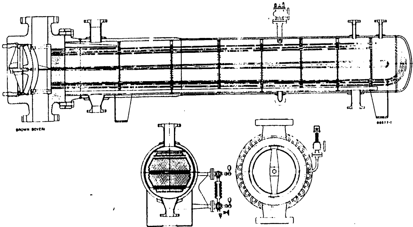
High Pressure Feedwater Heater
