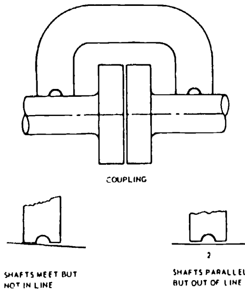
Use of Alignment Gage Fig. 10
