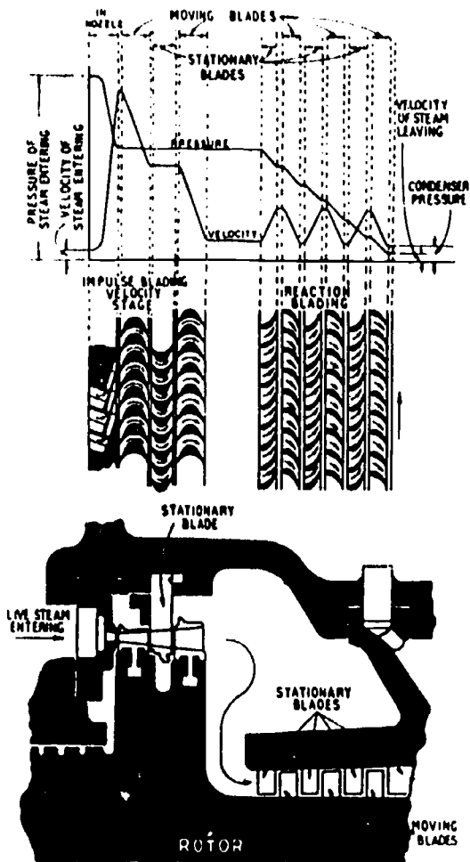
Reaction Turbine with Velocity Compounded Impulse Stage Fig. 10
