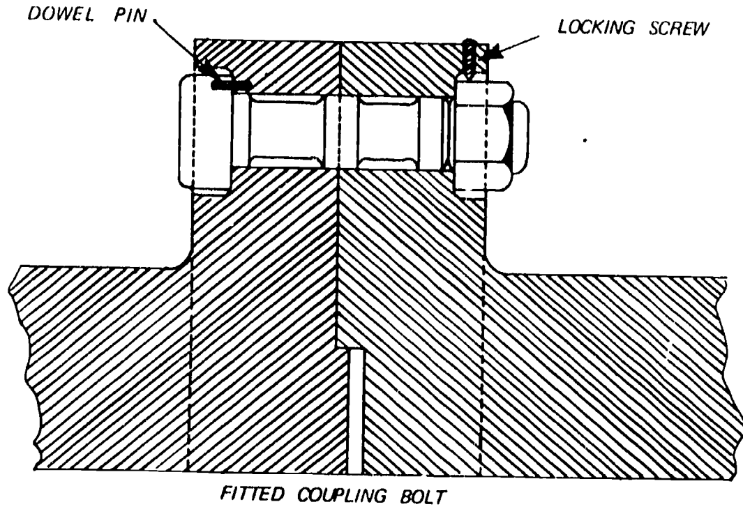
Solid Flange Coupling with Fitted Bolts
