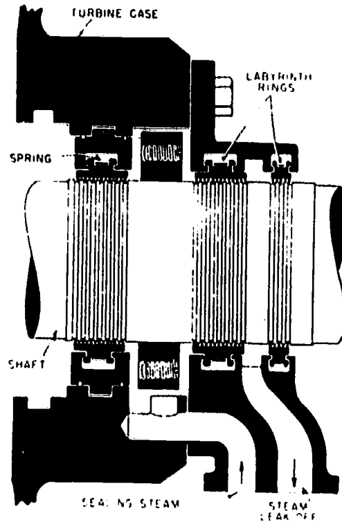
Low-Pressure Labyrinth Shaft Seal Fig. 25
