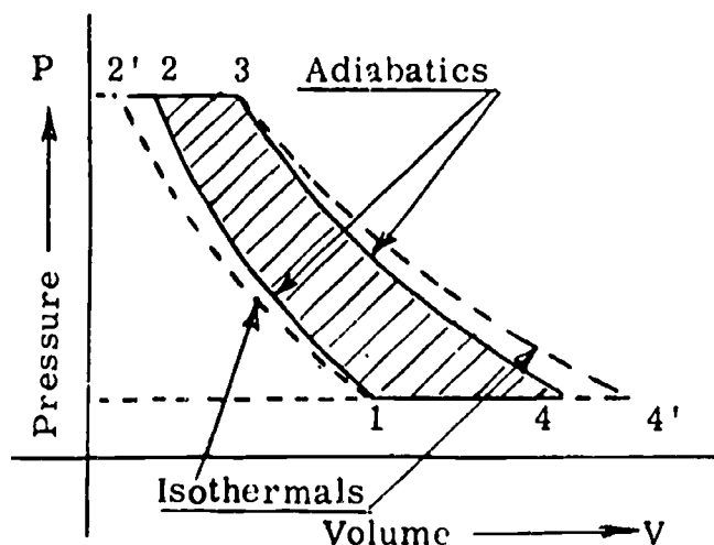
P-V Diagram for Brayton Cycle Fig. 9
