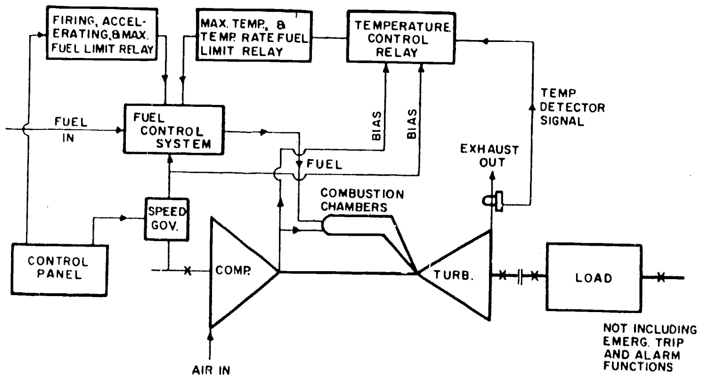
Typical Functional Control Diagram for SINGLE SHAFT GAS TURBINE Fig.32
