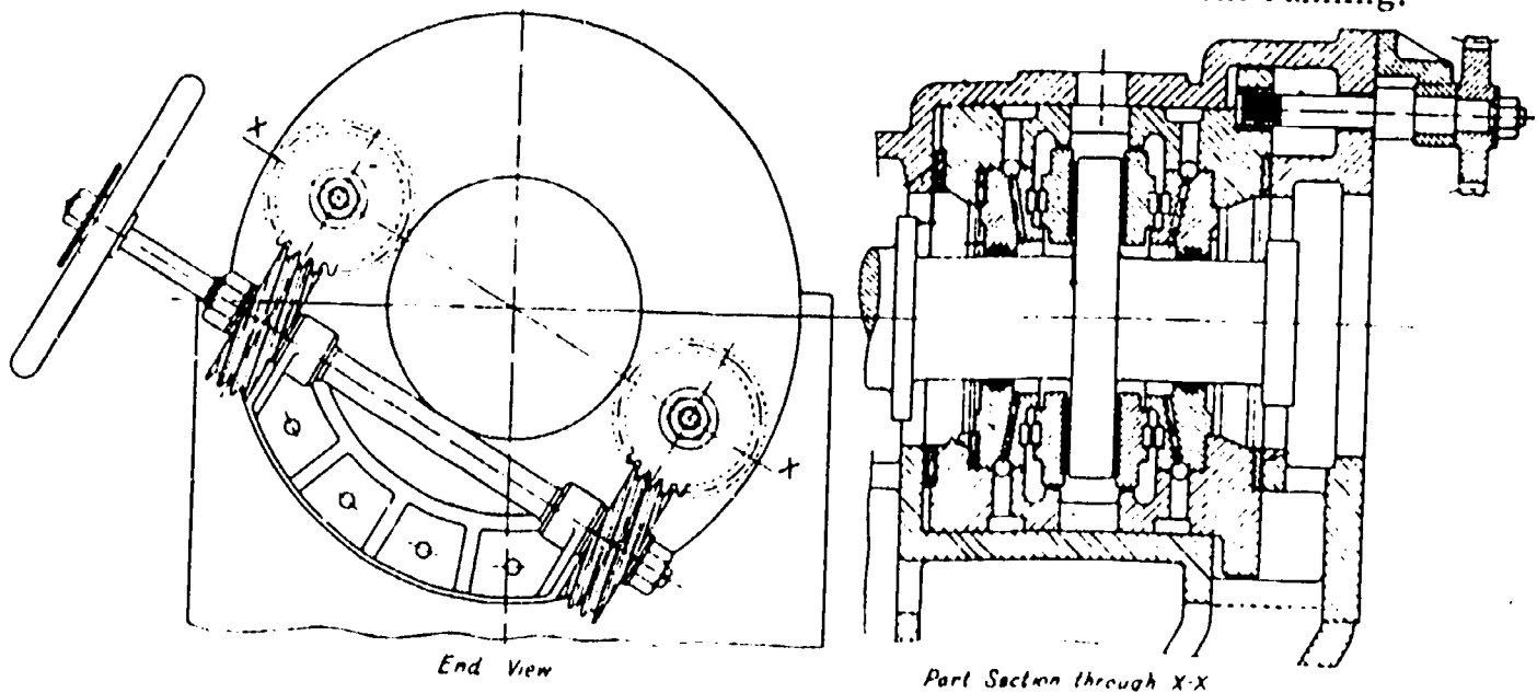
Turbine Thrust Adjusting Gear Fig. 20
