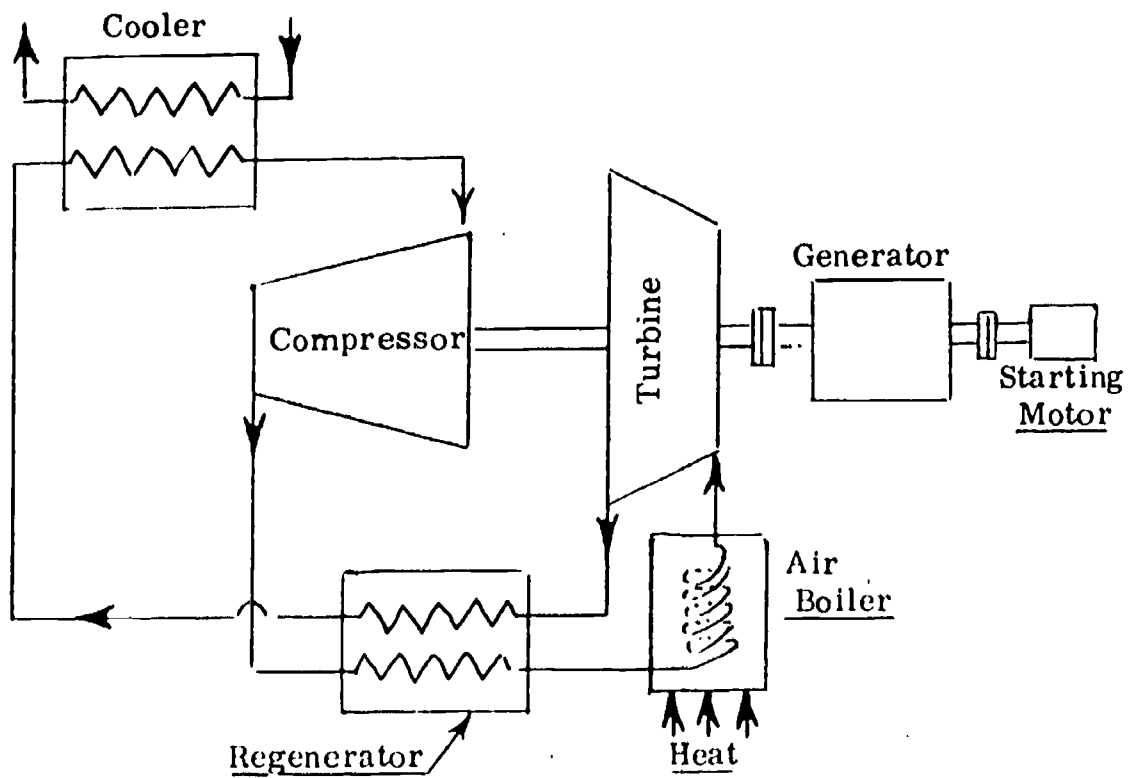
CLOSED CYCLE GAS TURBINE PLANT
