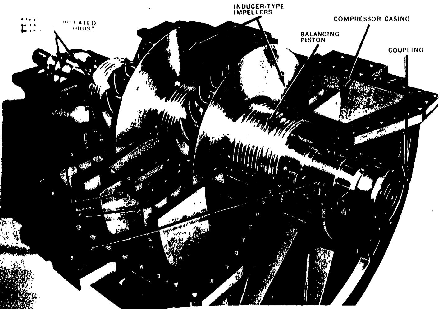
ELLIOTT CO TWO-STAGE COMPRESSOR Fig 18
