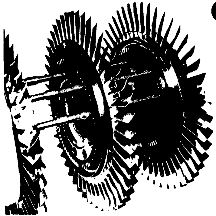
Individual discs are connected by a Curvic coupling and made rigid by a number of through bolts. (b)
