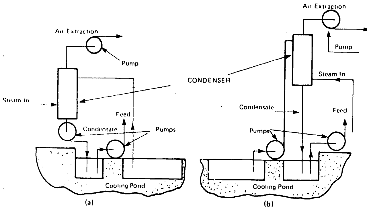
Jet Condenser Applications
