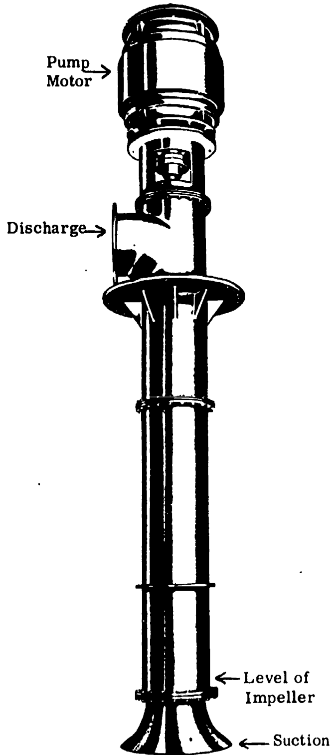
Vertical Mixed Flow CW Pump
