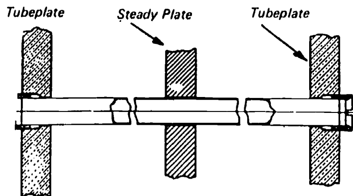
Tube secured at both ends with Ferrules
