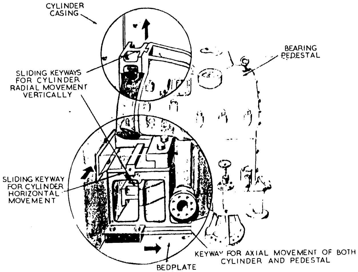
H-p Pedestal and Casing Support Fig. 13(a)
