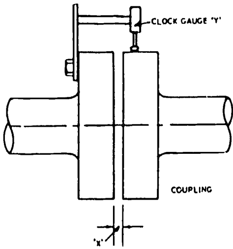
Alignment Measurements at Coupling Fig. 7
