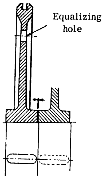
Rotor with shrunk-on discs
