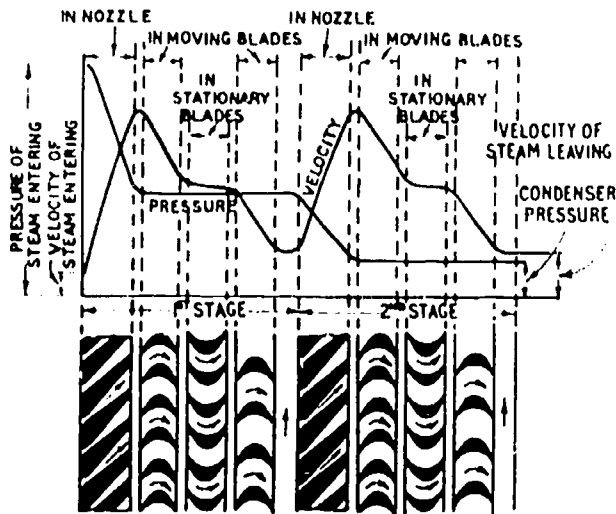
Pressure Velocity Compounding Impulse Turbine Fig. 7
