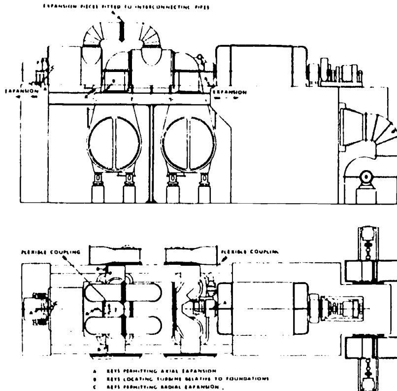
Provision for Expansion of Two-cylinder Turbine Fig. 13(b)
