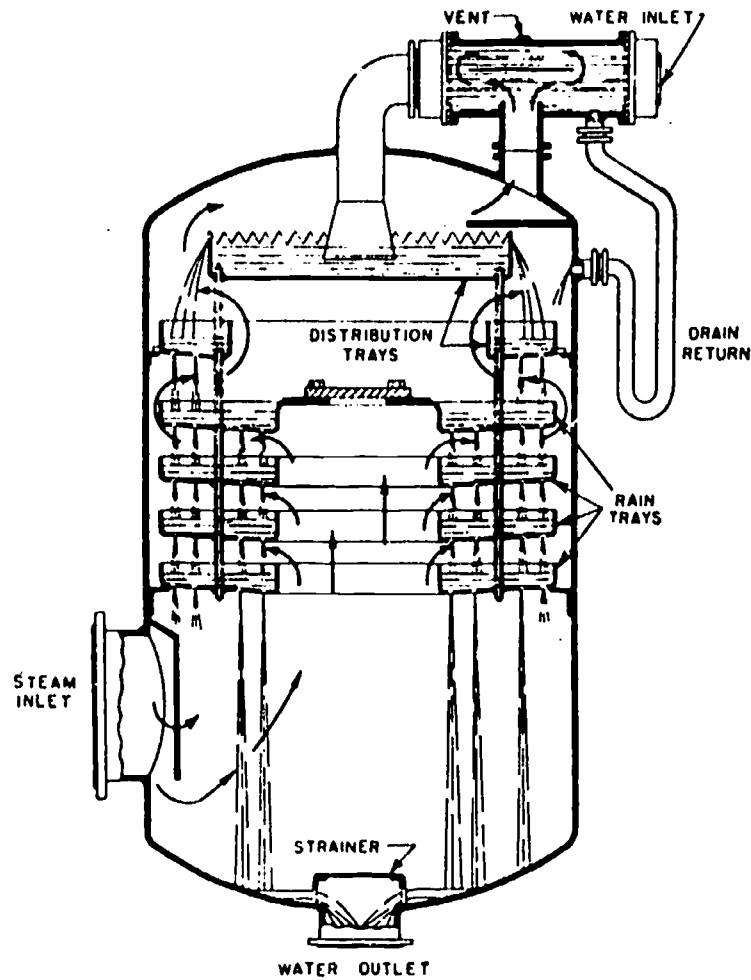
Tray-type Direct-contact Heater ( Foster Wheeler Corp. )
