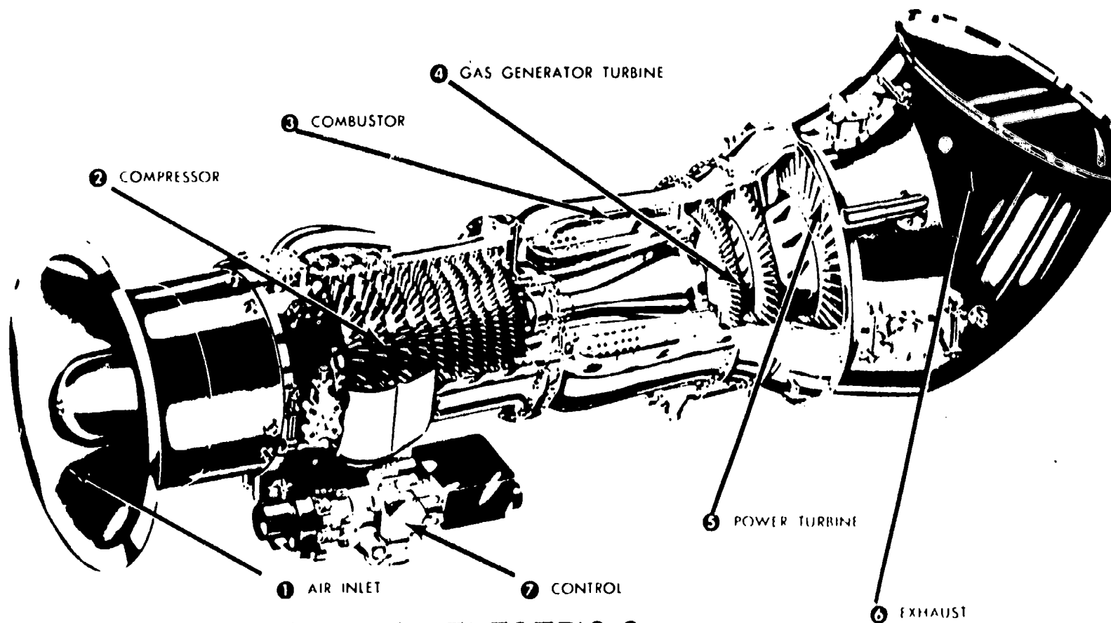
750 kW GENERAL ELECTRIC GAS TURBINE
