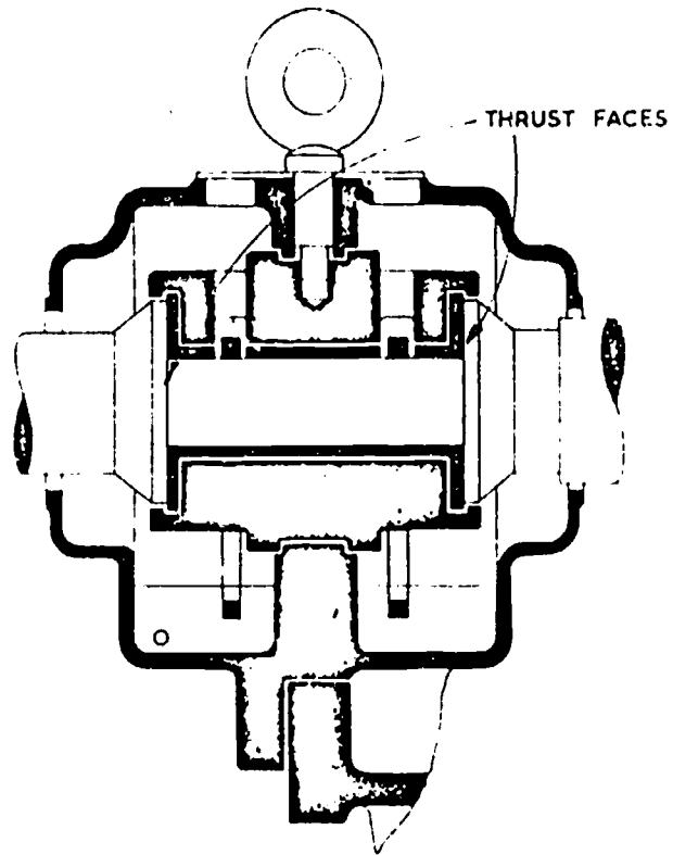
Ring Oiled Radial Bearing with Simple Thrust Pads on its ends Fig. 39
