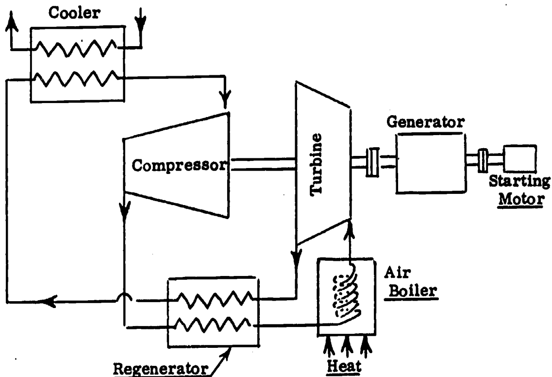
GAS TURBINE COMPONENTS
