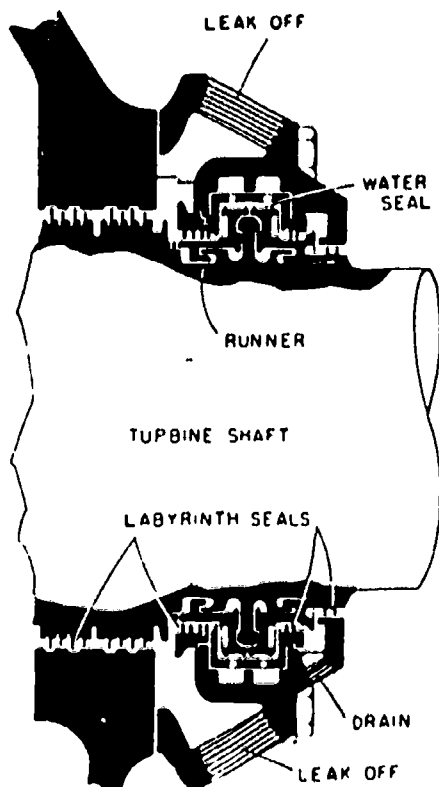
Combination Water Seal and Labyrinth Seal Fig. 27
