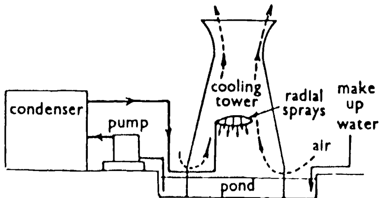
Condenser using Cooling Water from Cooling Tower
