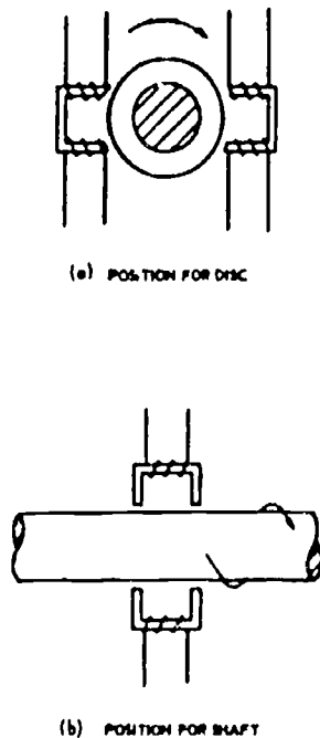
Arrangements of Eccentricity Detectors
