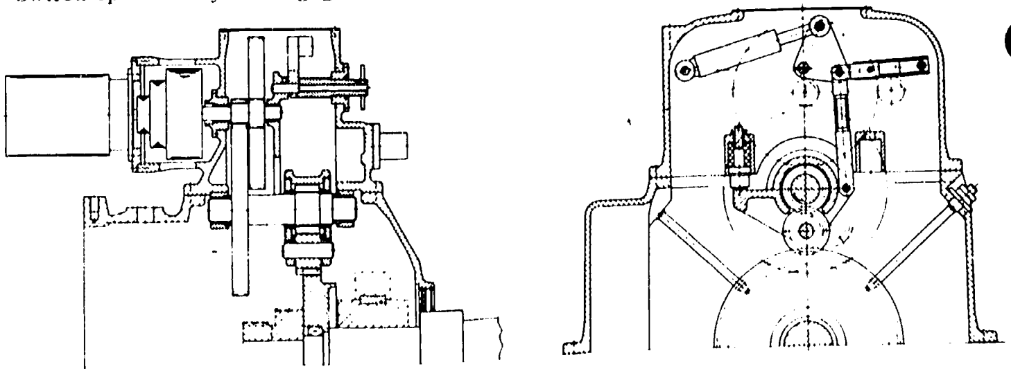
Electric Turning Gear
