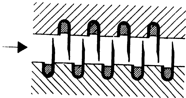
Labyrinth Seal
