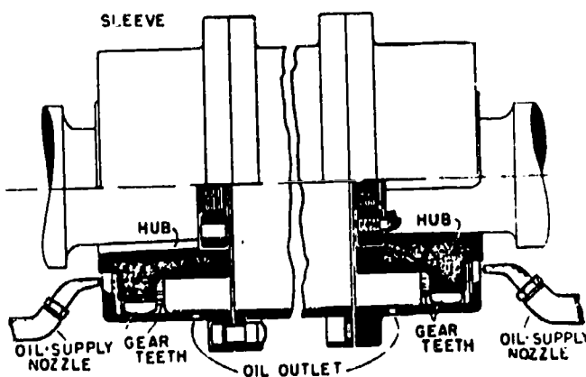
Flexible Coupling
