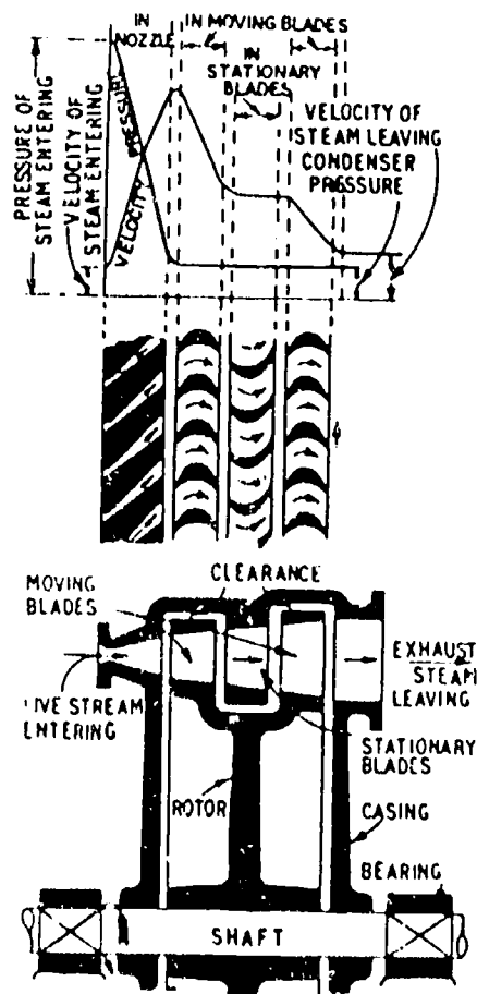
Velocity Compounded Impulse Turbine Fig. 3
