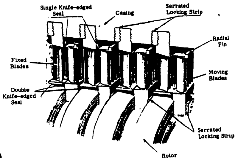
H-p Reaction Type Blading
