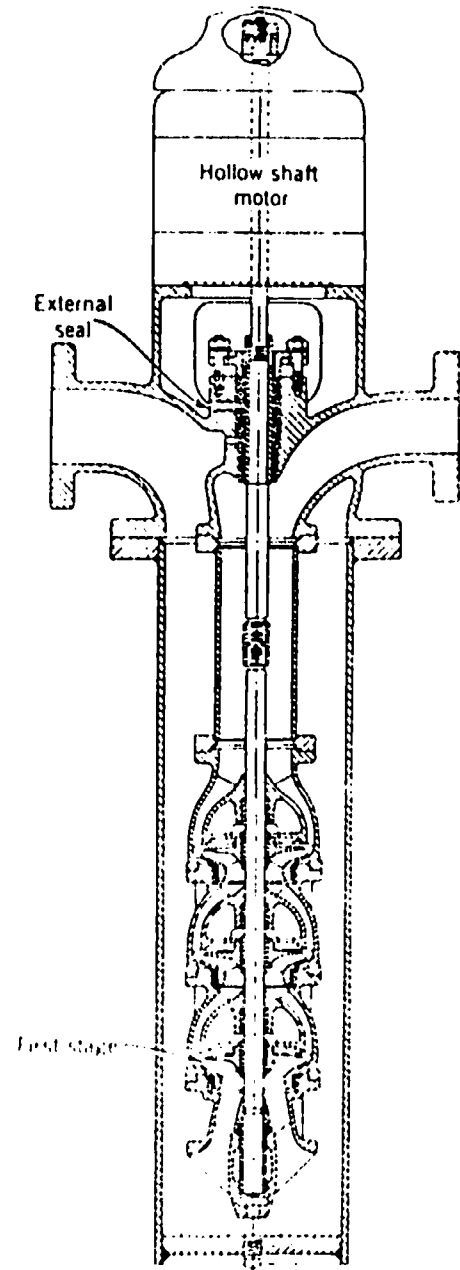
Vertical Multistage Condensate Pumps of the Turbine Type
