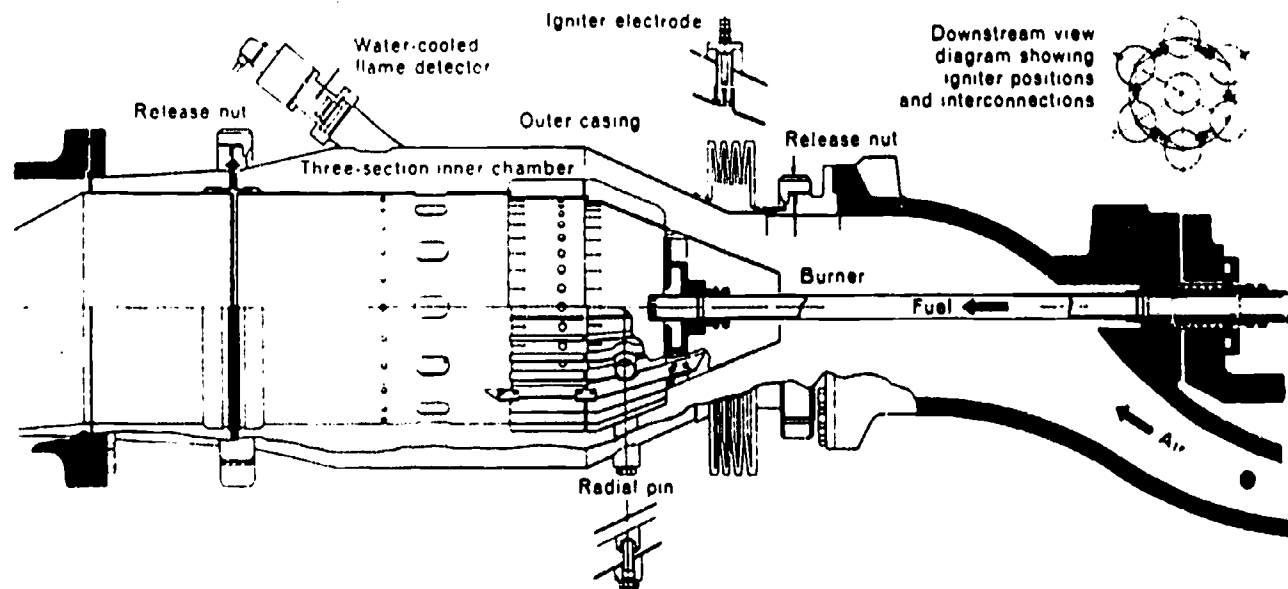
COMBUSTION CHAMBER ARRANGEMENT
