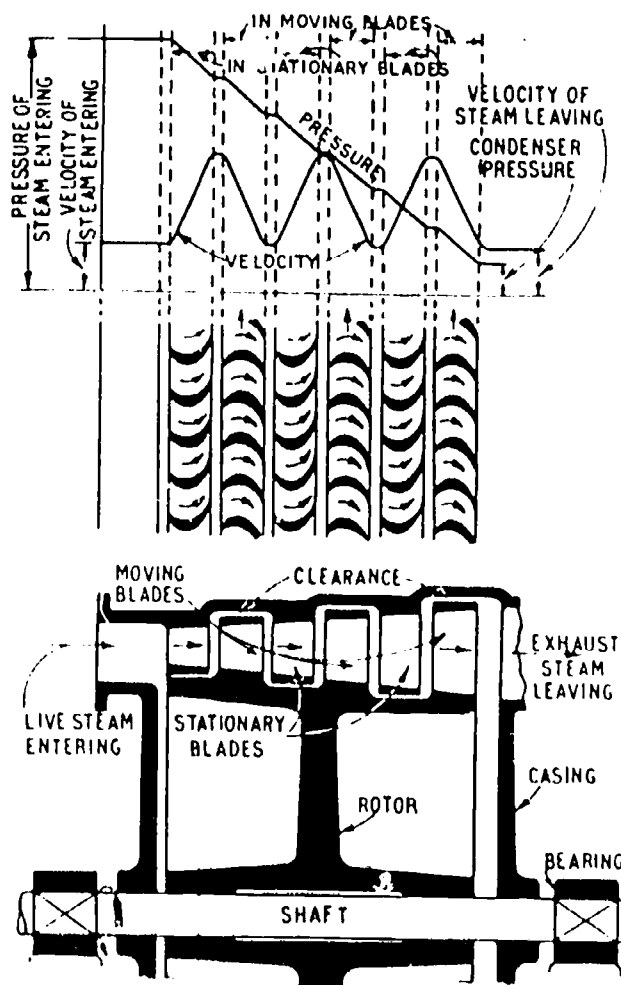
Simple Reaction Turbine
