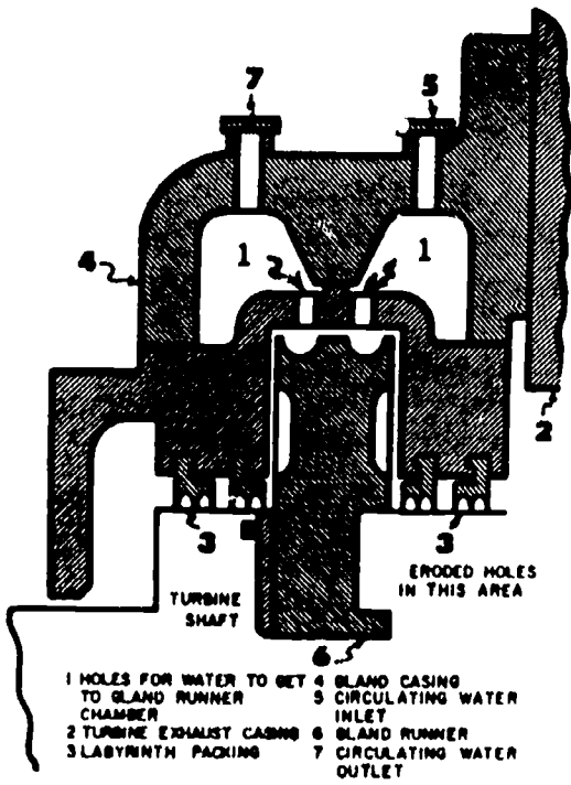
Water Sealed Gland
