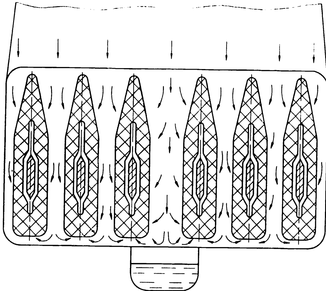
Large Condenser with Radial Flow Tube Banks
