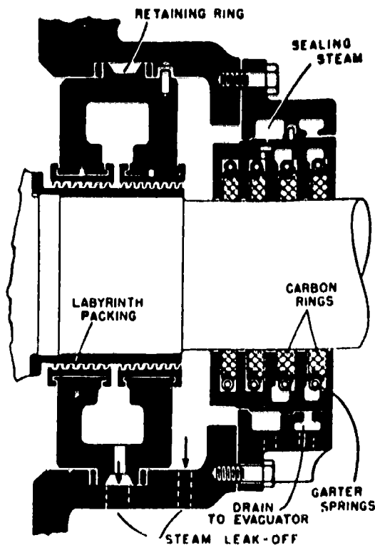
Combination Labyrinth and Carbon Ring Shaft Seal Fig. 26
