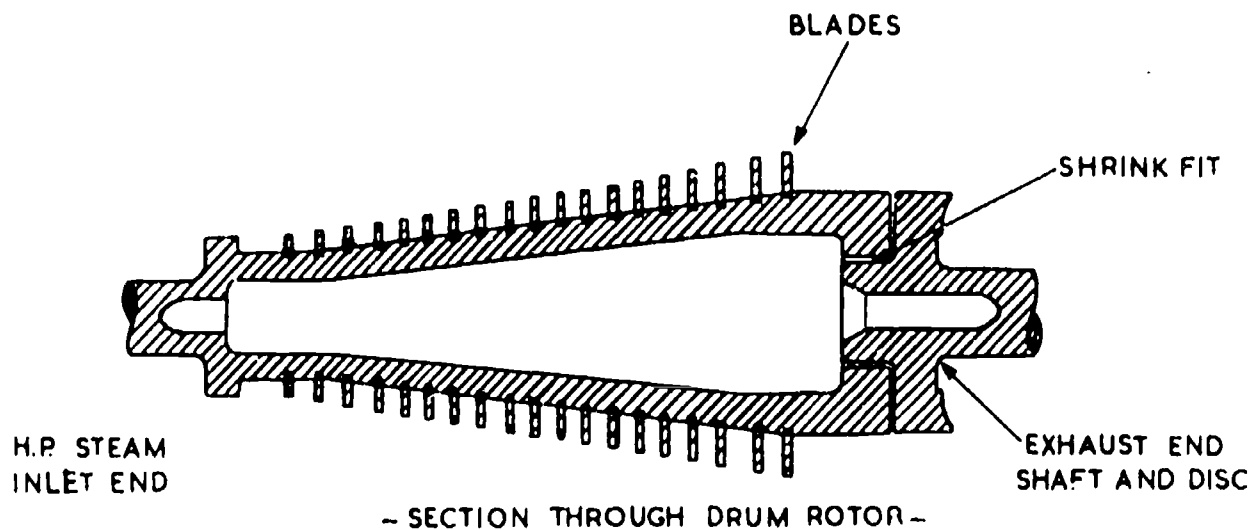
Hollow Drum Rotor
