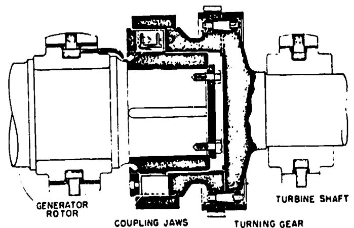
Claw Type Coupling
