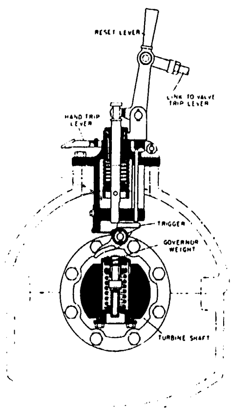
Emergency Overspeed Governor Fig. 28
