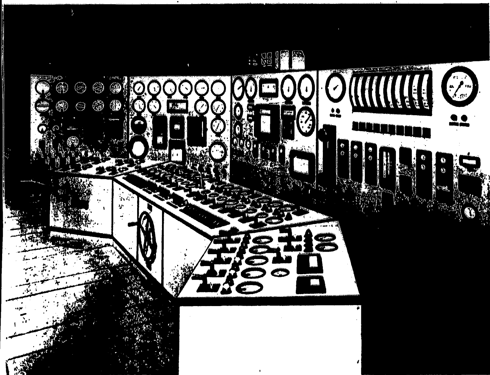
Combined Boiler and Turbine Unit Control Panel
