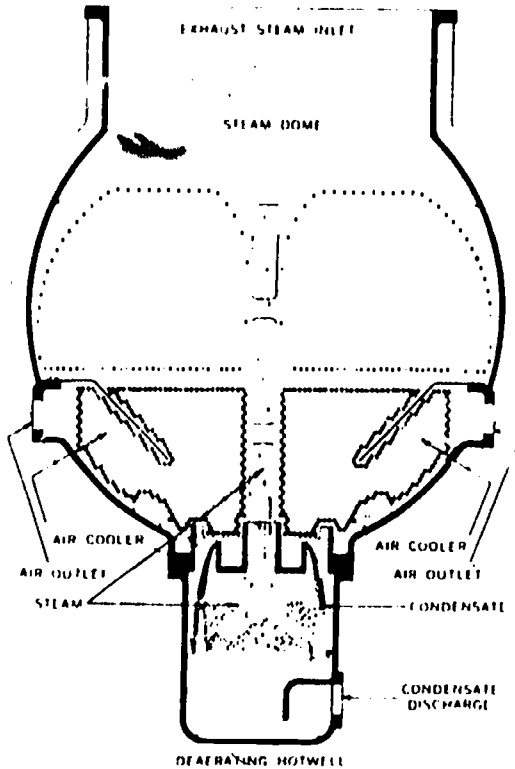
Down Flow Condenser
