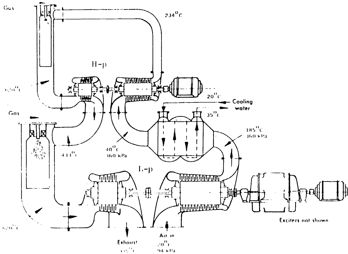
TEMPERATURES and PRESSURES Fig.34
