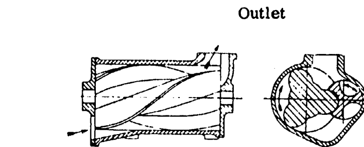
LYSHOLM COMPRESSOR
