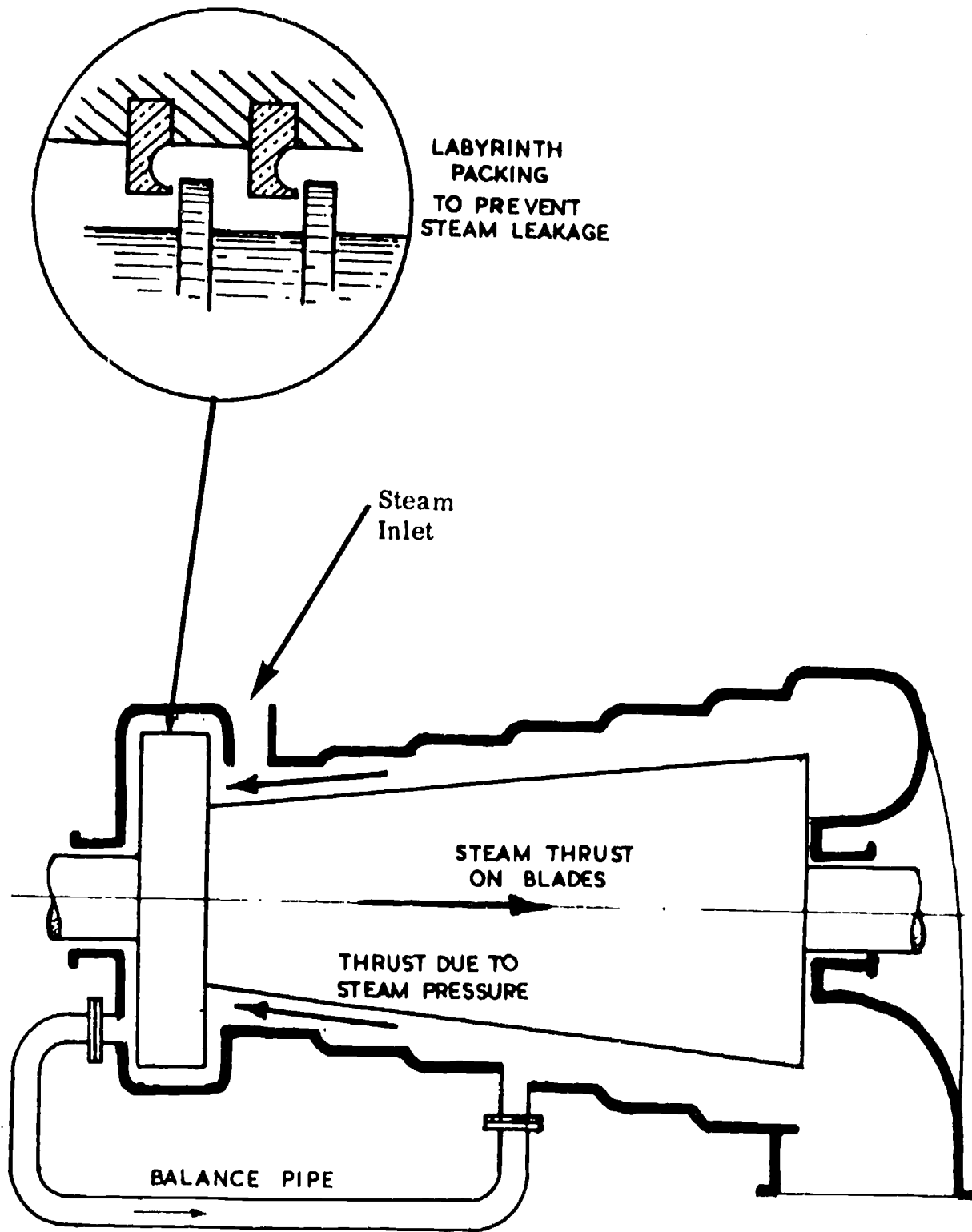
Dummy Piston and Balance Pipe
