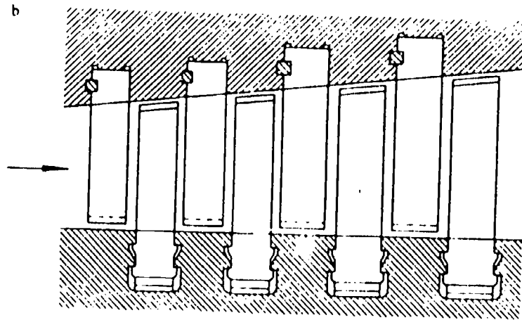
Drum-type rotor with tip-sealed blades Fig. 38
