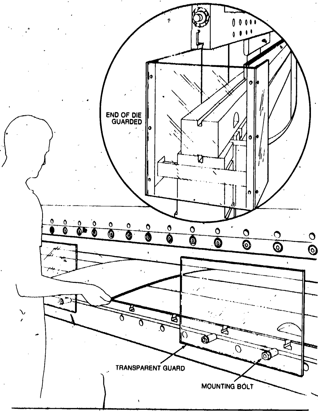
Figure 17. Fixed guard providing protection from unused portion of die on a press brake
