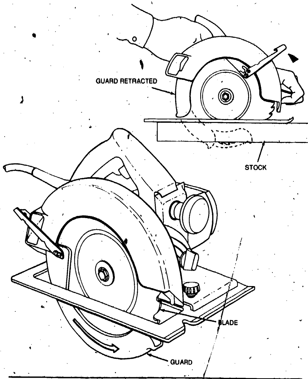
Figure 30. Self-adjusting guard on circular saw
