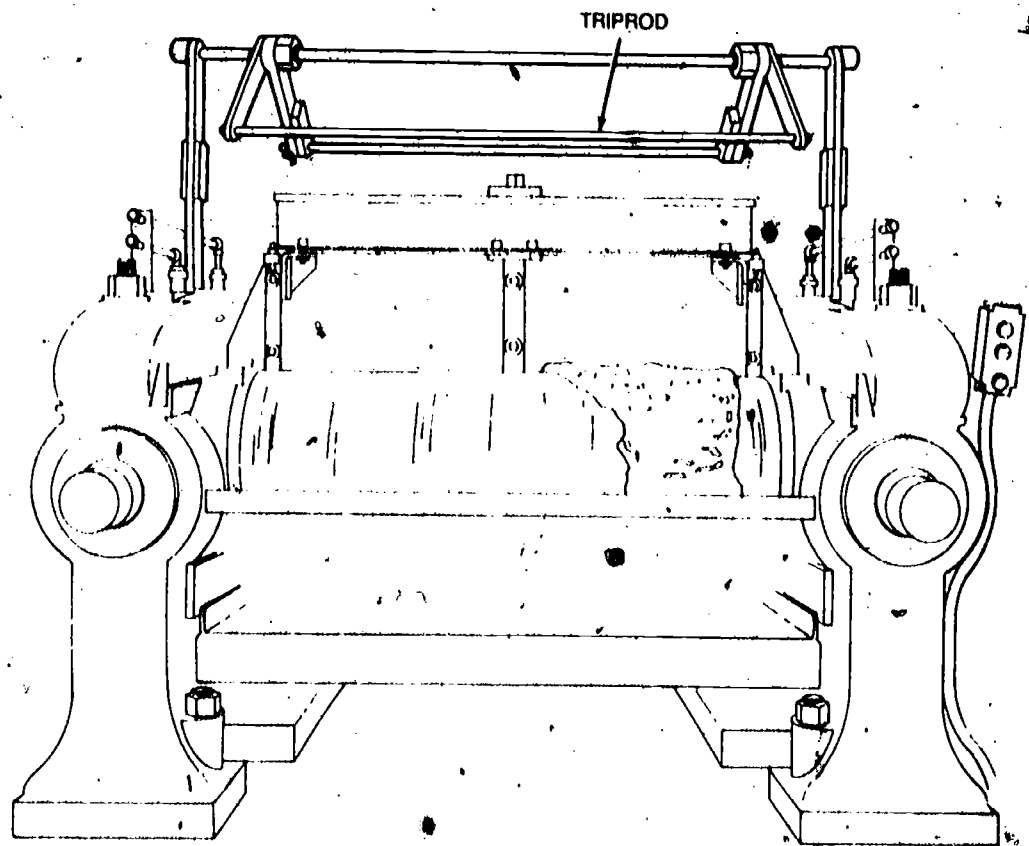
Figure 42. Safety triprod on a rubber mill
