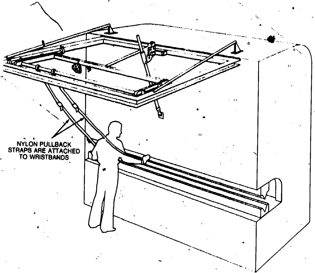
Figure 39. Pullback device on press brake
