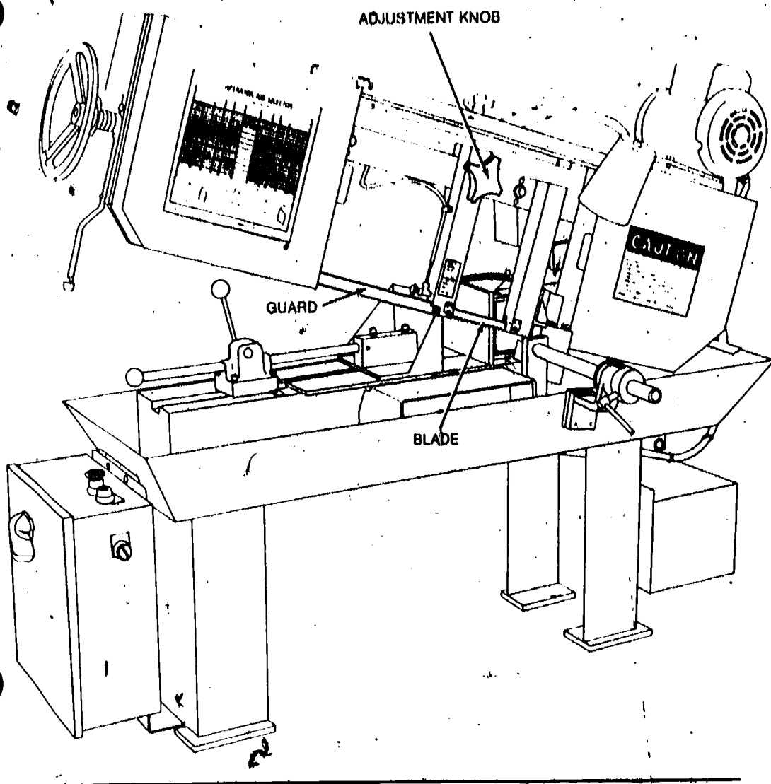
Figure 22. Adjustable guard on horizontal bandsaw
