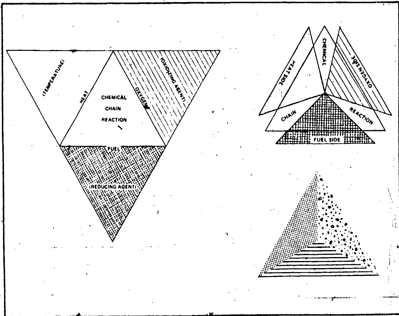
Figure 2-2 The "fire tetrahedron", a four-sided solid, was suggested to include the chemical chain reaction as another component necessary for burning. The components would then form a pyramid.
