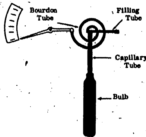
Remote Bulb Thermometer
