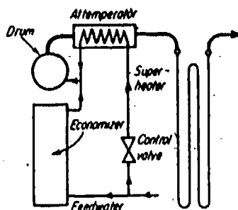
Economizers
