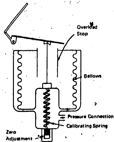
Bellows Pressure Gauge
