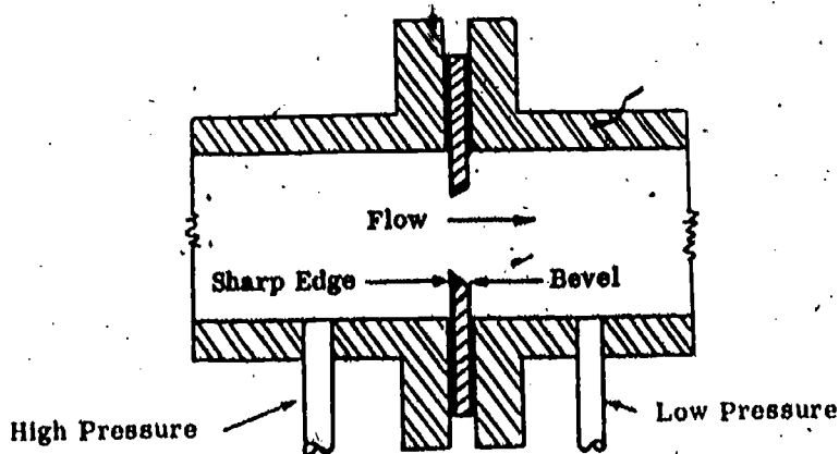
Orifice Plate with Pressure Taps
