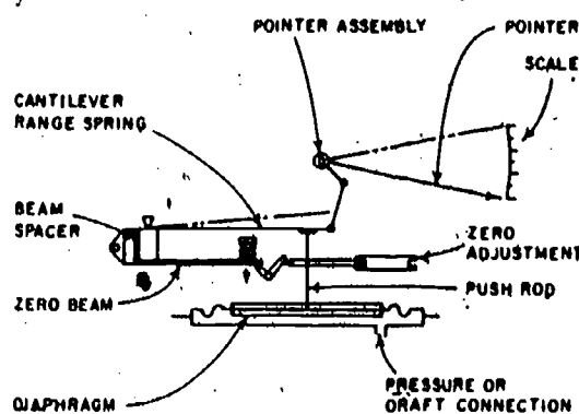
Diaphragm Pressure Gage
