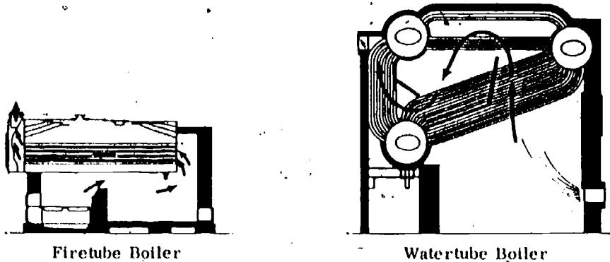
Firetube Boiler
