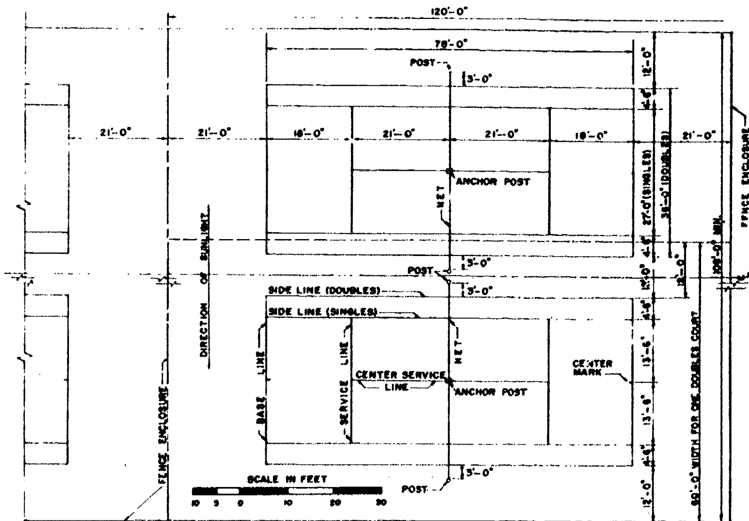
Figure 3-23 Tennis Court Layout.
