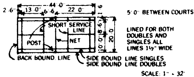
Figure 2-20 Badminton Court Dimensions.
