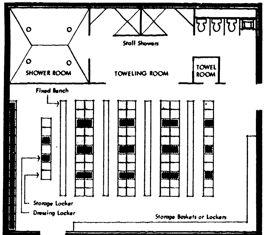
Figure 6-4 Location of locker and showers.
