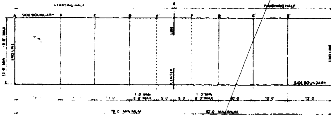
Figure 7-6 Layout of a Bocce court.
