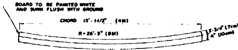
DETAIL - JAVELIN THROW SCRATCH BOARD
