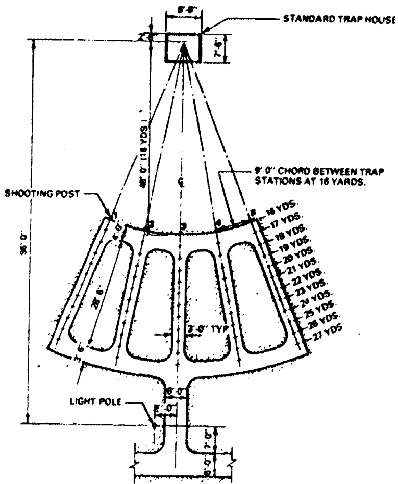
Figure 7-19 Small bore rifle and carbine range.
