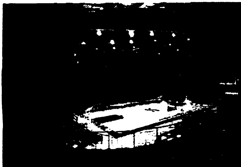
Figure 5-8 The Welsh-Ryan Arena at North- western University utilizes long spinning steel arches.
