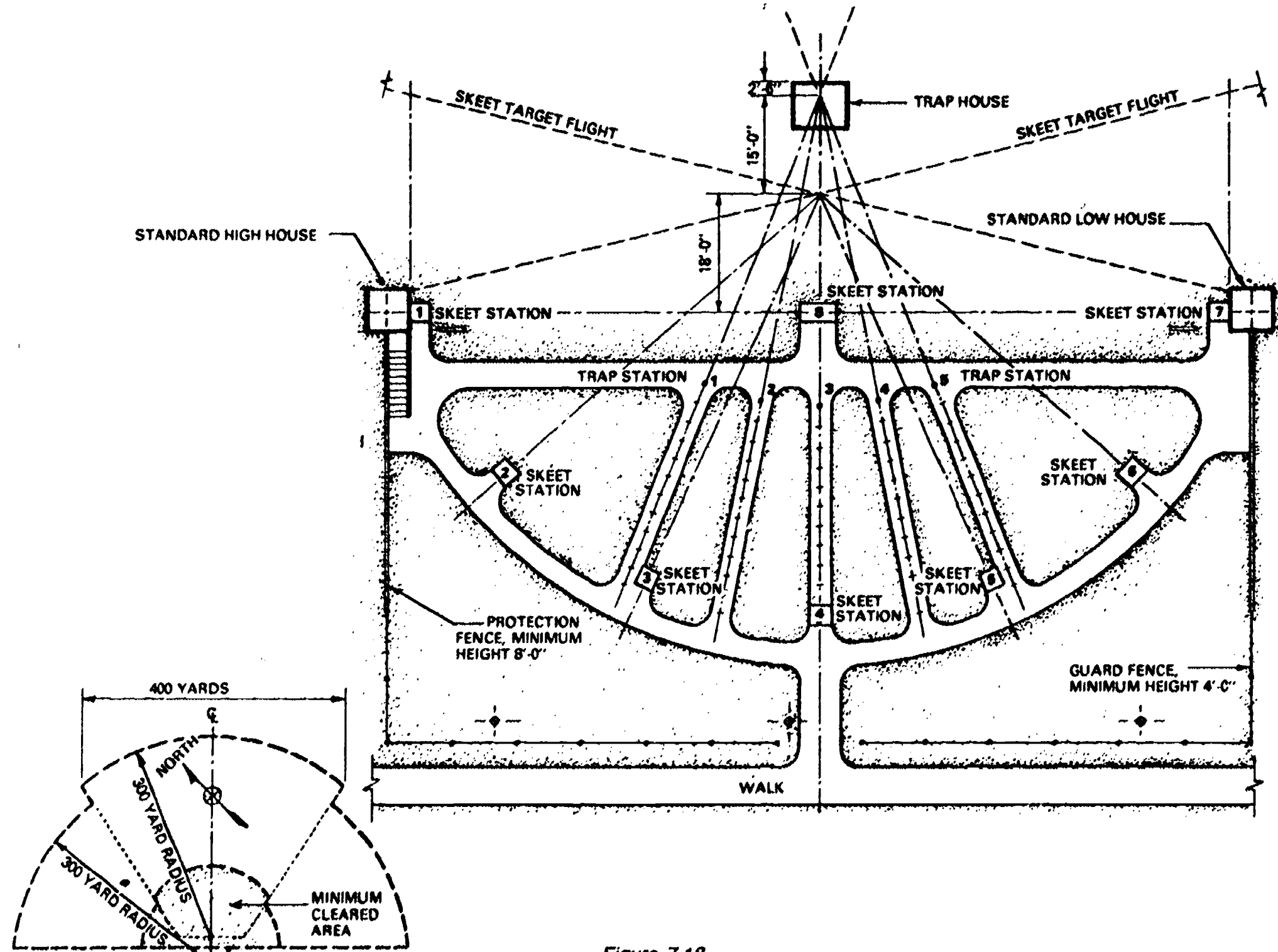
Figure 7-18 Combination Trap and Skeet field layout.
