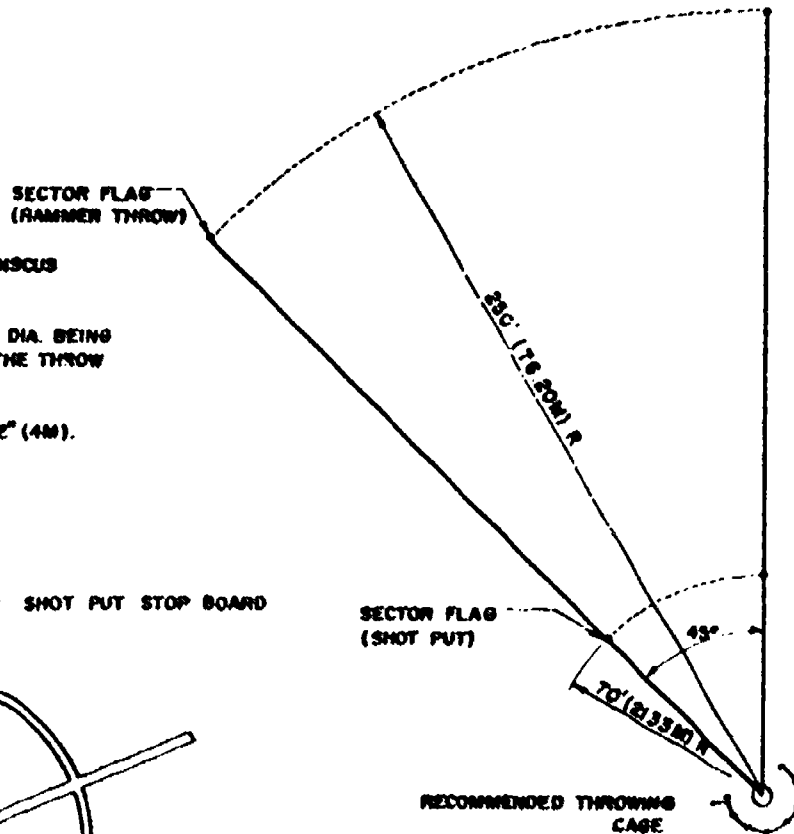
SECTOR LAYOUT - SHOT PUT & HAMMER THROW
