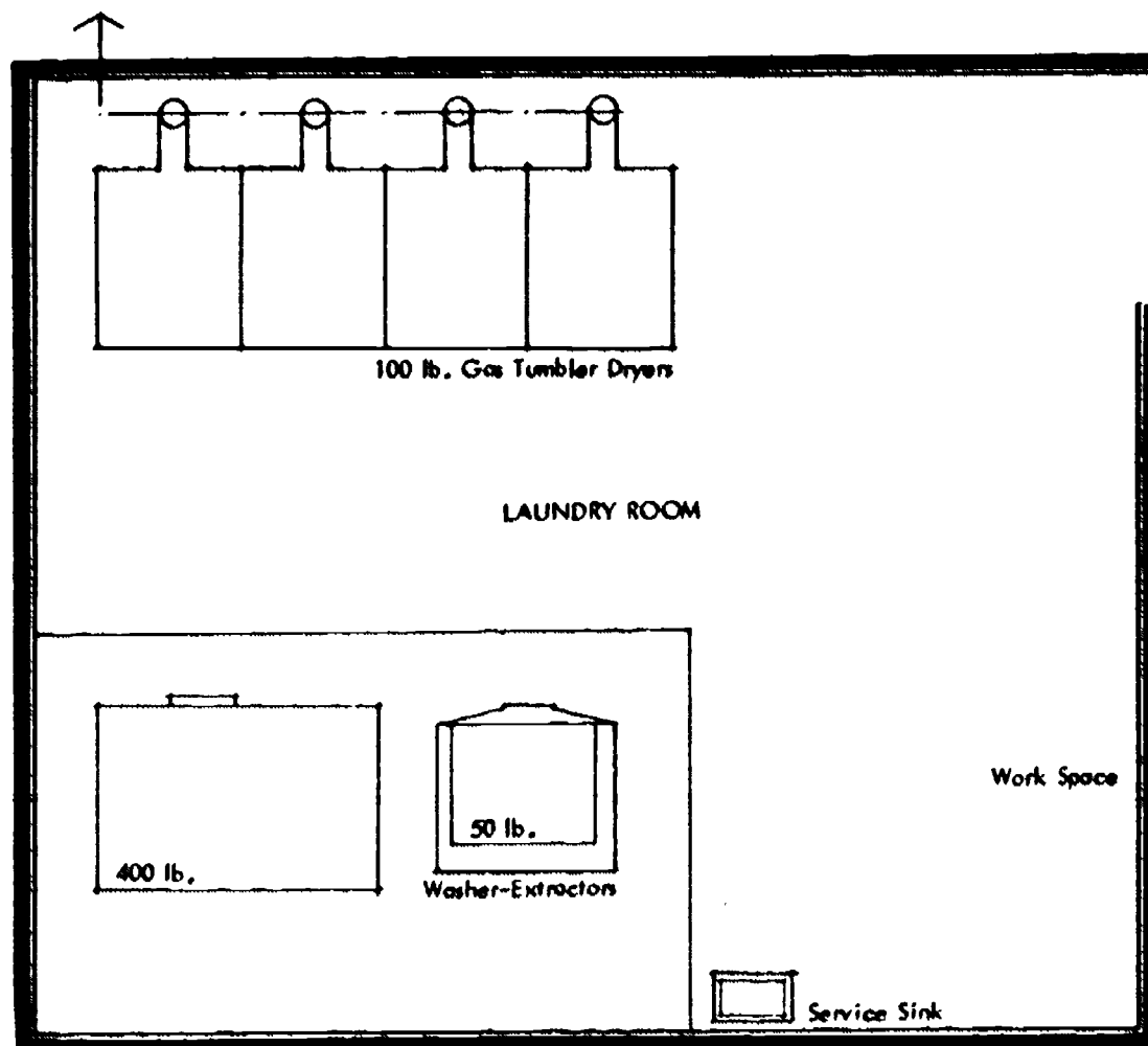
Figure 6-20 Suggested laundry room layout.
