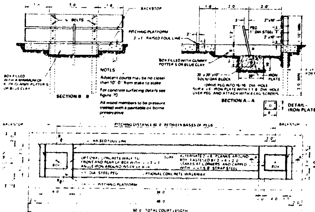
Figure 7-6A Horseshoe pitching layout.
