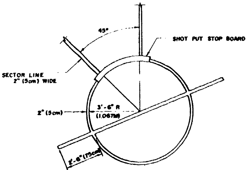
SHOT PUT & HAMMER THROW CIRCLE
