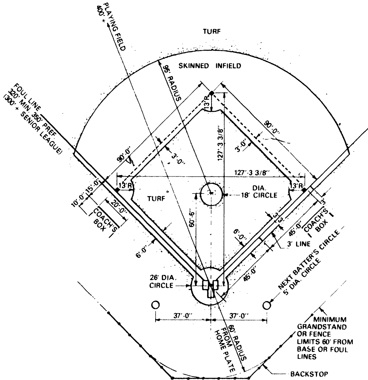
BASEBALL DIAMOND LAYOUT
