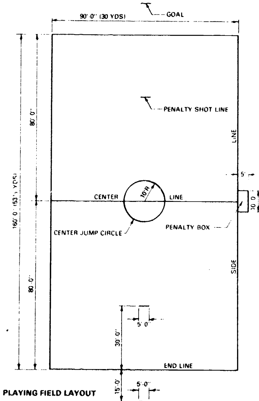
Figure 3-13 Flicker Ball Field
