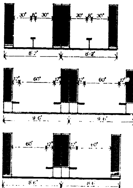
Figure 6-17 Dressing bench arrangements.
