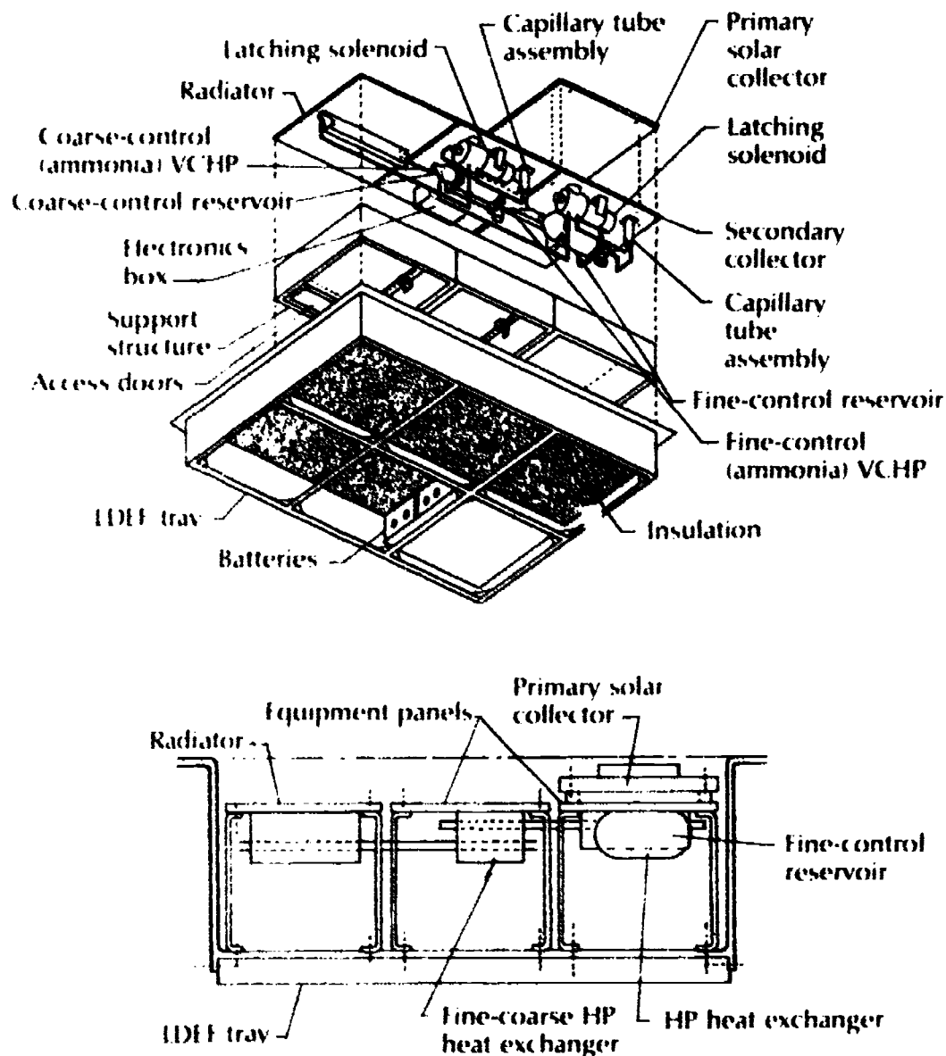
Figure 30. Cascade variable-conductance heat pipe configuration.
