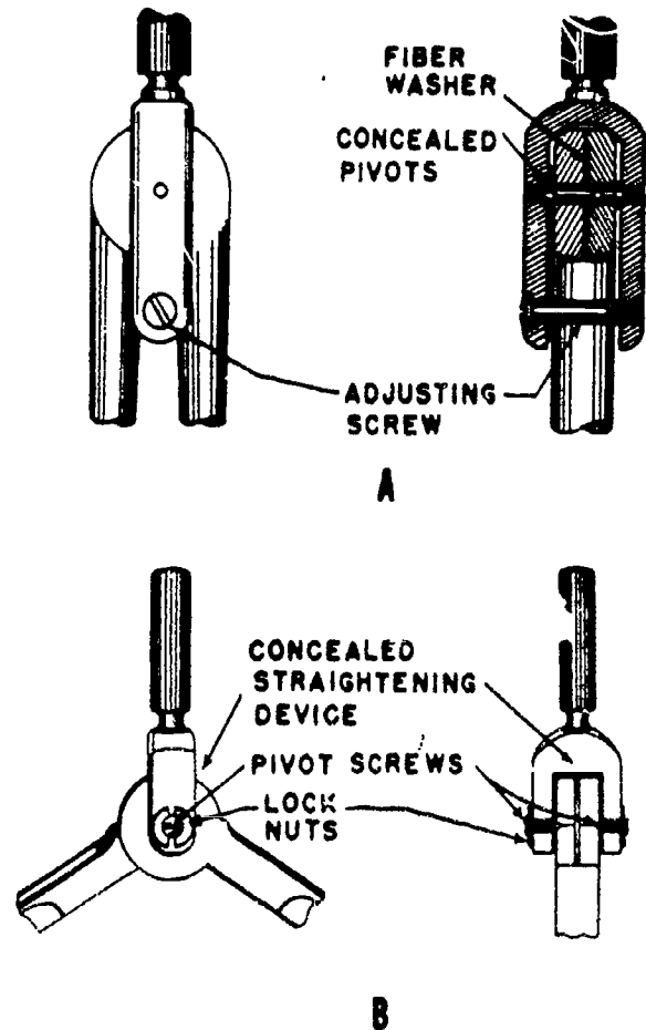
Figure 4-14.—Types of pivot joints.
