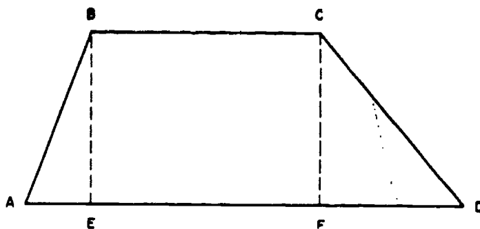
Figure 3-12.—Trapezoid.
