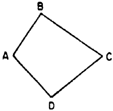
2. QUADRILATERAL
