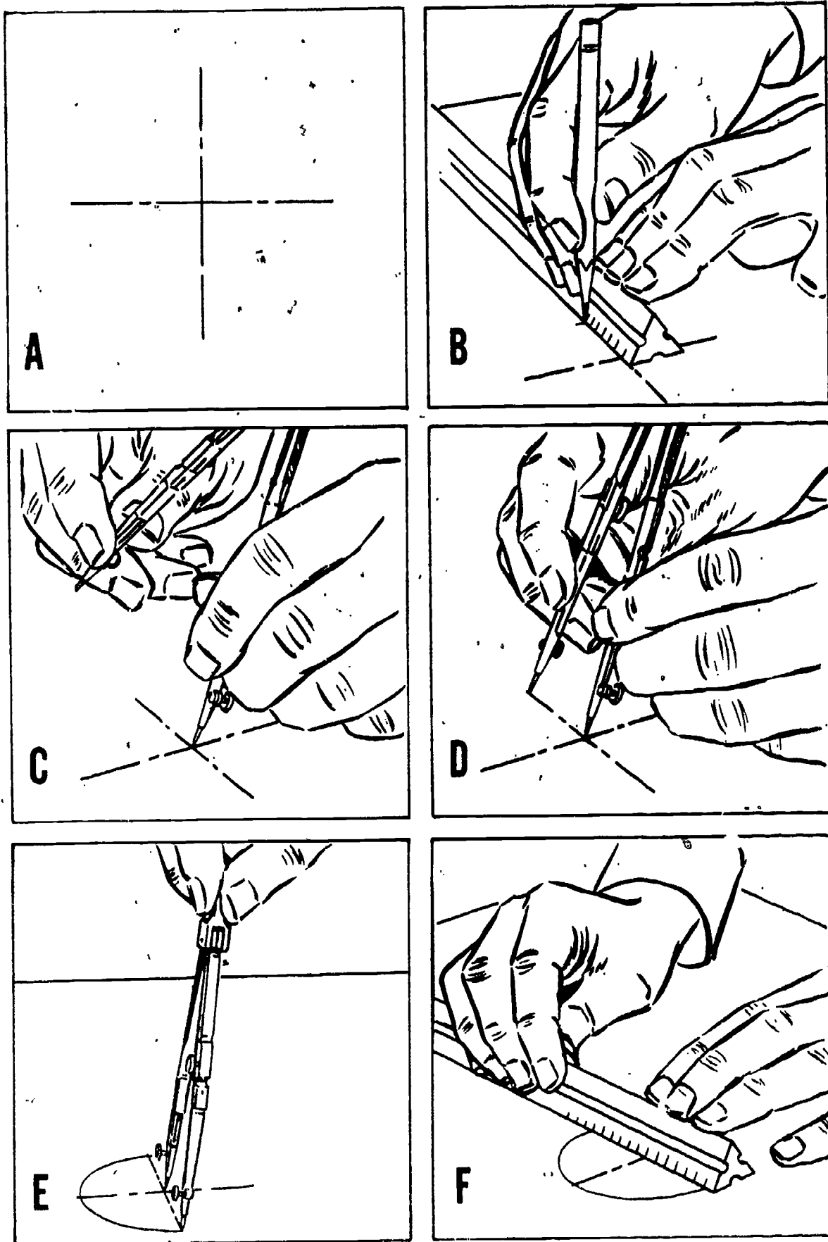
Figure 5-8.—Drawing a circle of given radius in pencil.
