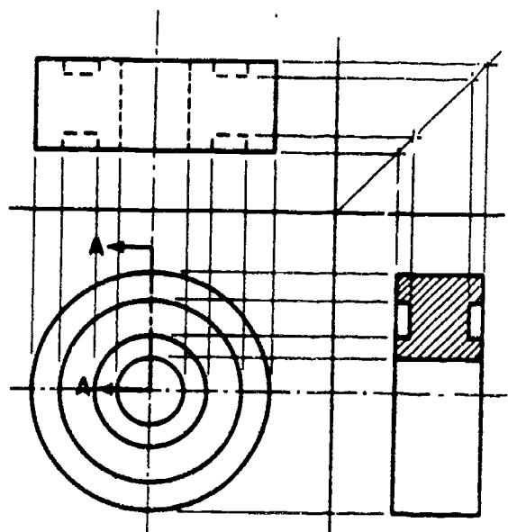
Figure 8-29.—Half section.
