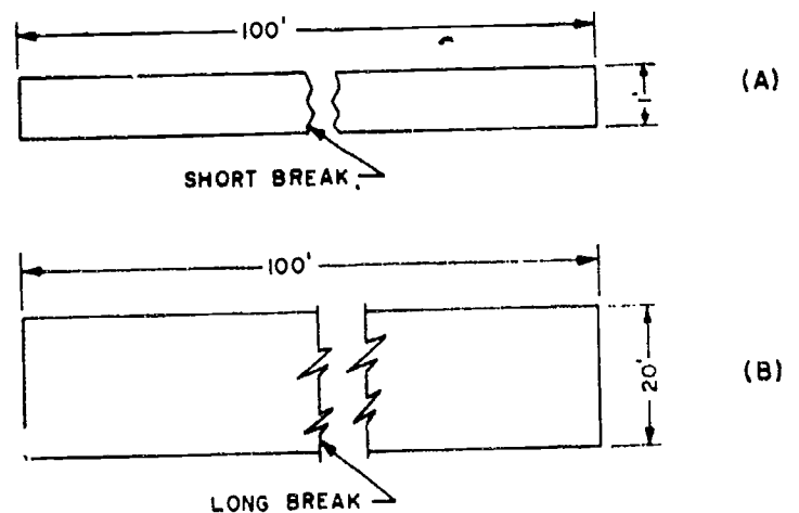
Figure 5-38.—Line conventions for (A) short break, and (B) long break.
