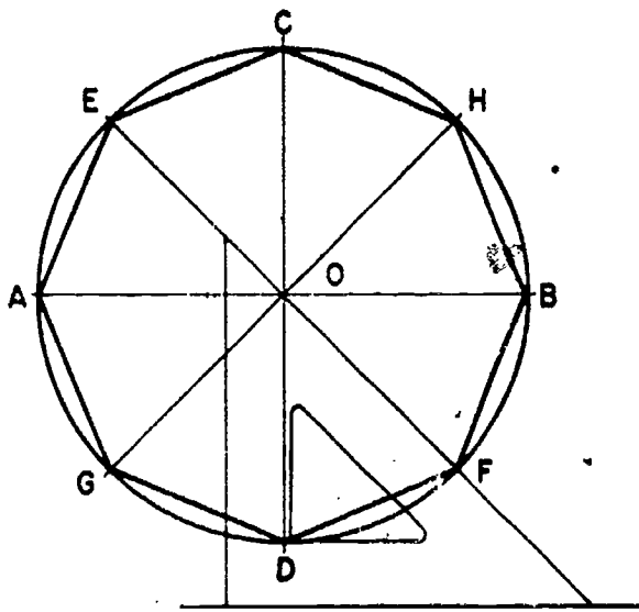
Figure 7-29.—Regular octagon in given circumscribed circle.
