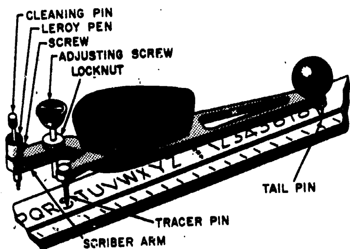
Figure 6-19.—Leroy scriber and template. 45.120
