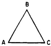
1. TRIANGLE
