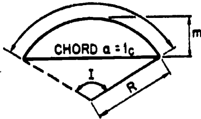
CIRCULAR SEGMENT
