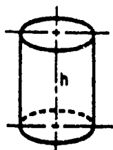
RIGHT CIRCULAR
