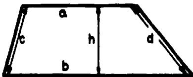
TRAPEZOID
