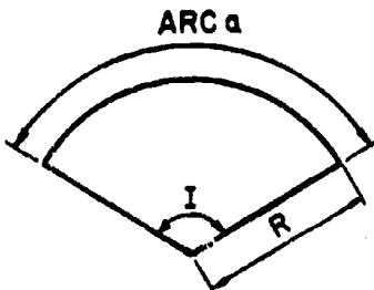
CIRCULAR SECTOR
