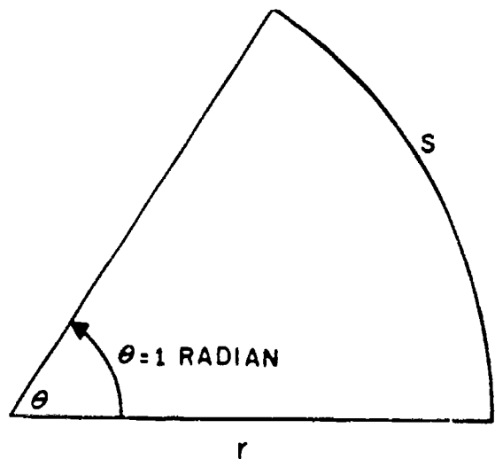
Figure 3-22.—Radian measure.
