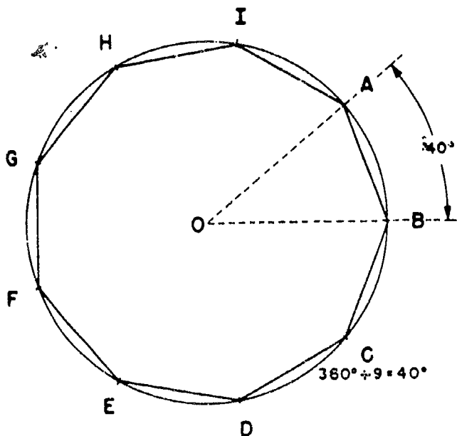
Figure 7-22.—Regular polygon in given circumscribed circle.
