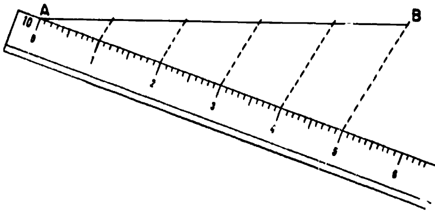
Figure 7-9.—Using a scale to lay off equal intervals on random line.
