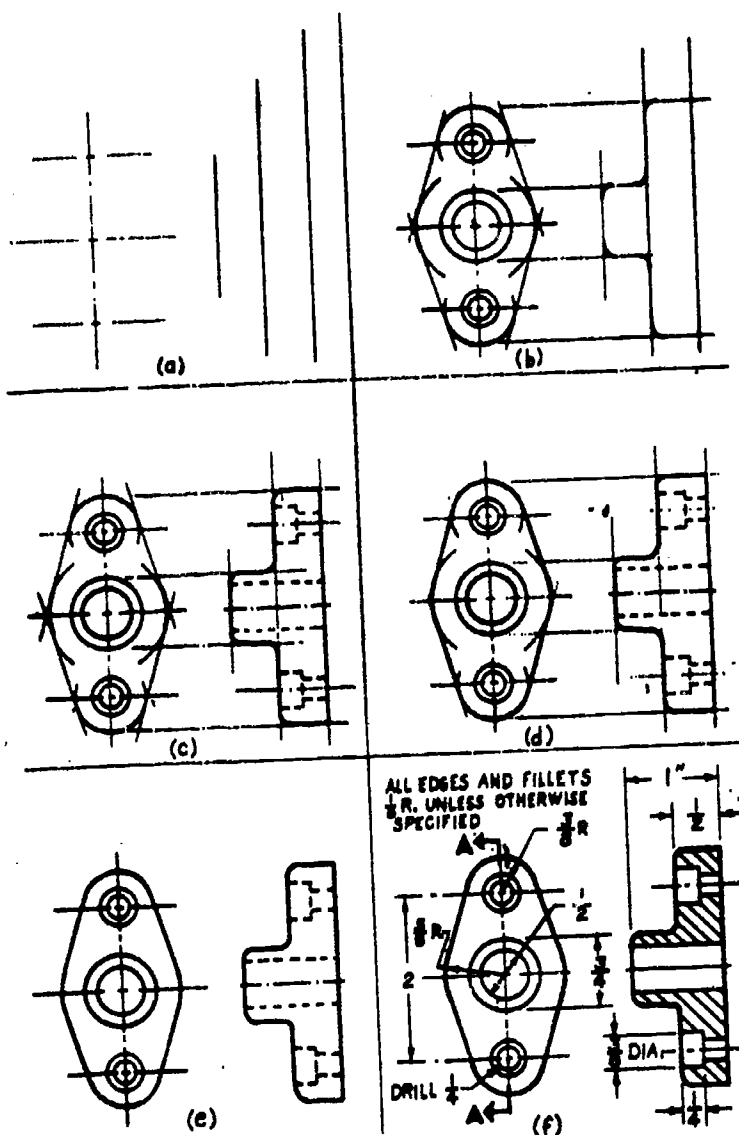
Figure 5-44.—Order of penciling a drawing.
