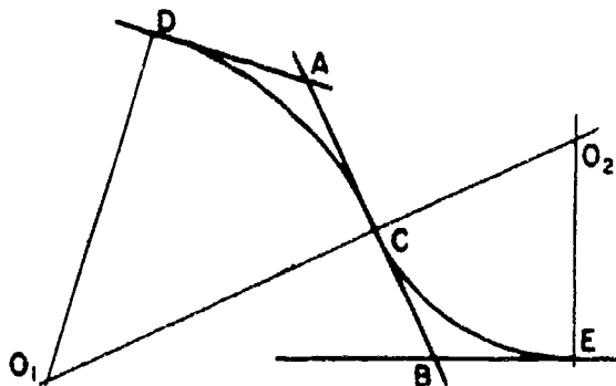
Figure 7-42.--Reverse curve tangent to three intersecting straight lines.
