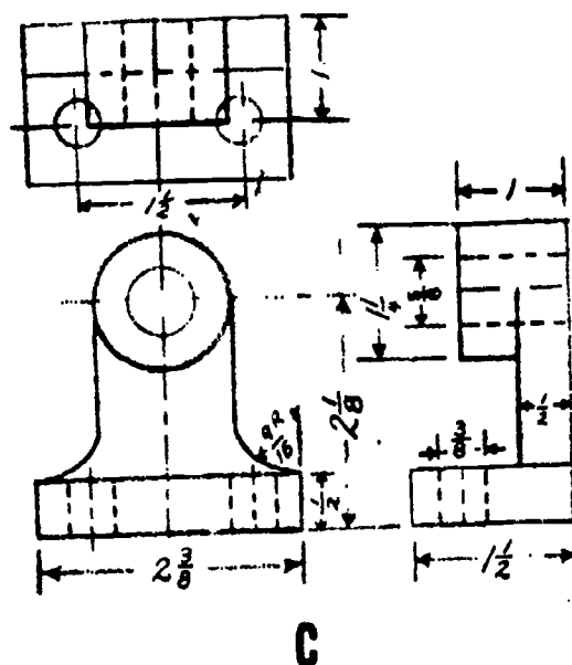
Figure 8-64.—Progress of a working sketch.
