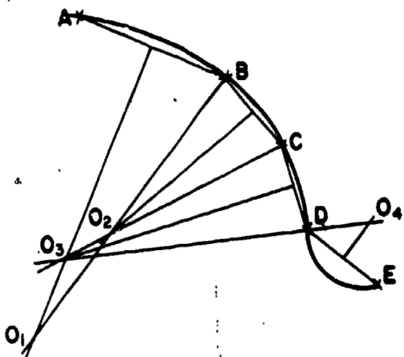
Figure 7-40.--Curve composed of a series of consecutive tangent circular arcs.
