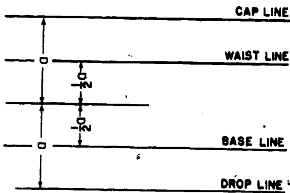
Figure 6-2.—Laying off guidelines.
