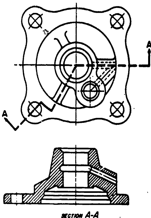
Figure 5-43.—Offset section.
