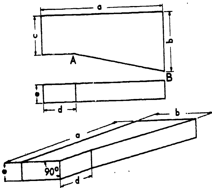
Figure 8-41.—Cavalier projection of an object with irregular lines.
