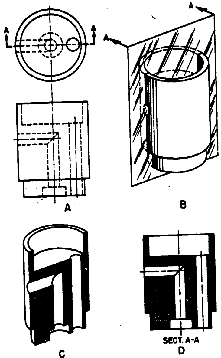
Figure 5-42.—Action of a cutting plane.
