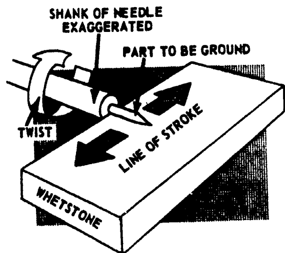
142.35 Figure 4-16.—Shaping a compass needle.
