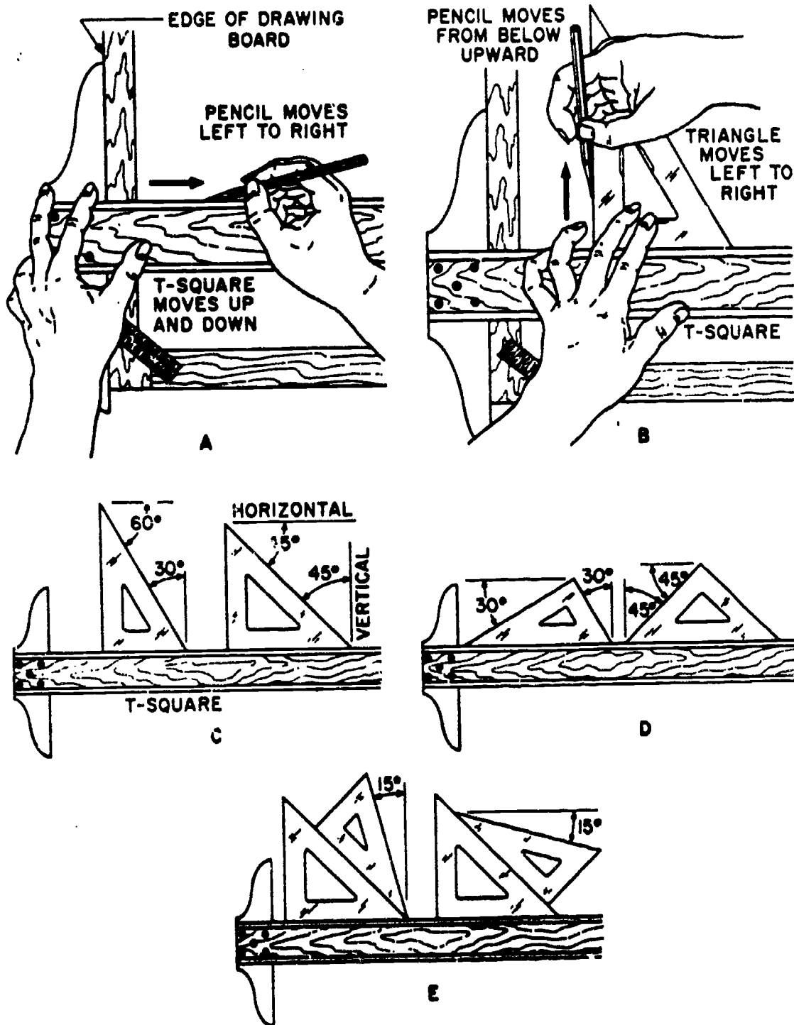
Figure 5-3.—Construction of basic lines.
