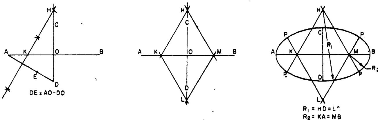
Figure 7-45.—Ellipse by four center method.
