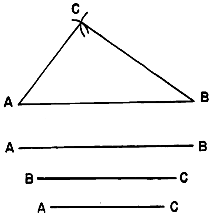
Figure 7-12.—Constructing a triangle with three sides given.
