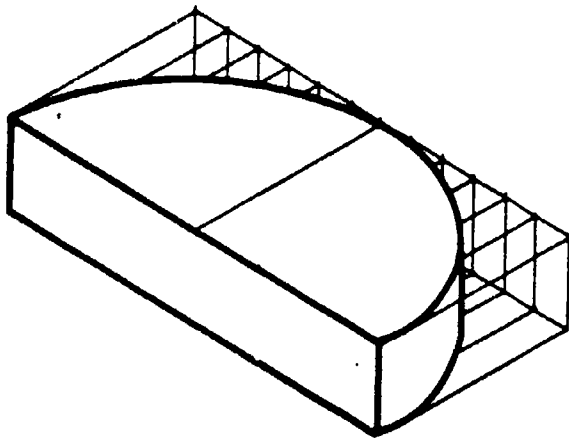
Figure 8-50.—Method of drawing a noncircular curve in isometric.
