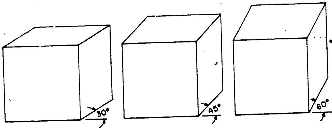
Figure 8-40.— 30^\circ , 45^\circ , and 60^\circ are the normal angles chosen for the receding axis in oblique projection because they are easily drawn with triangles.
