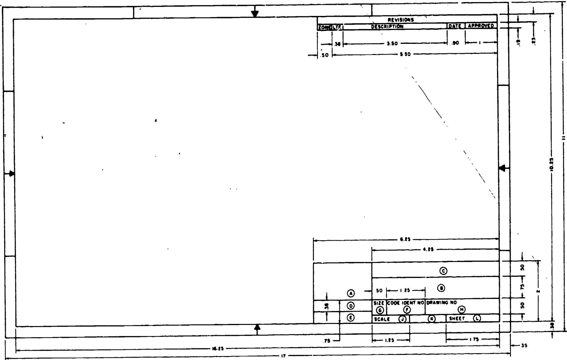
Figure 5-21.—Format for "B" size drawings.
