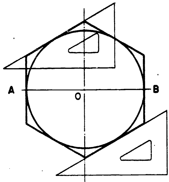
Figure 7-28.—Regular hexagon on given inscribed circle.
