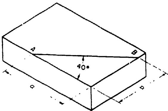
Figure 8-48.--Drawing an angle in isometric.
