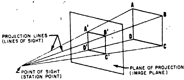
(A) PERSPECTIVE PICTORIAL PROJECTION
