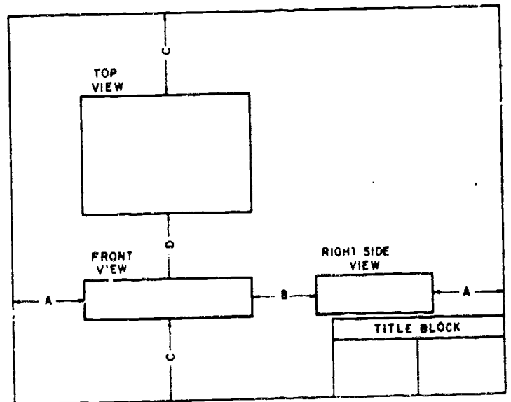
Figure 8-11.—Proper spacing of views on a three-view projection.
