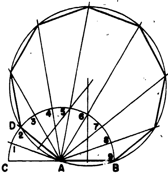
Figure 7-24.—Any regular polygon with given length of side.
