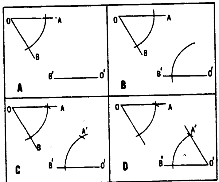
Figure 7-1.—Transferring an angle.
