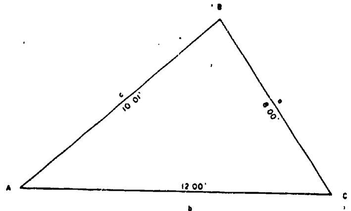
Figure 3-28.—Any triangle—three sides given.
