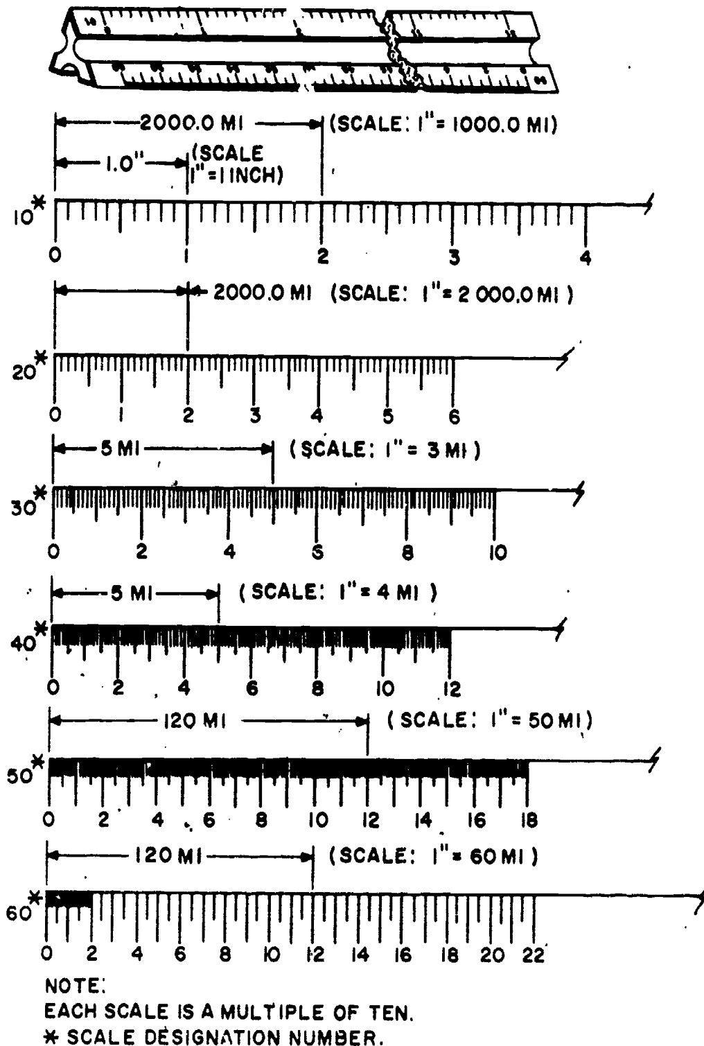
Figure 4-24.—Engineer's scale.
