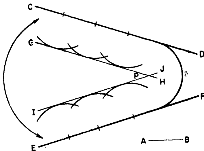
Figure 7-34.—Circular arc tangent to two lines which form any angle.
