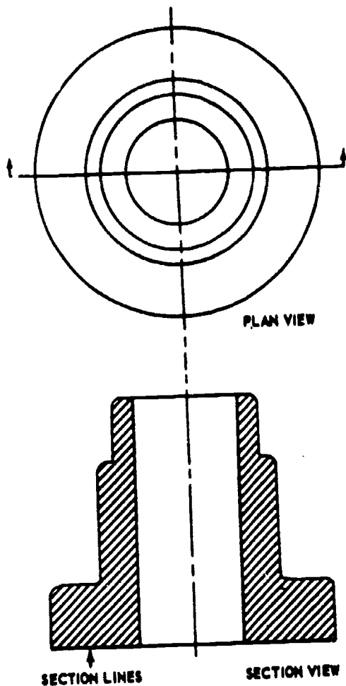
Figure 5-41.—Plan view and section.
