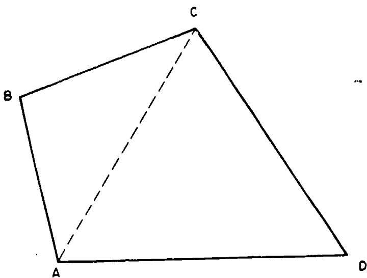
Figure 3-13.—Trapezium.
