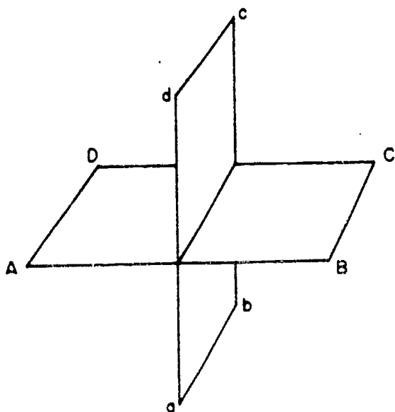
Figure 3-5.—Intersecting planes.
