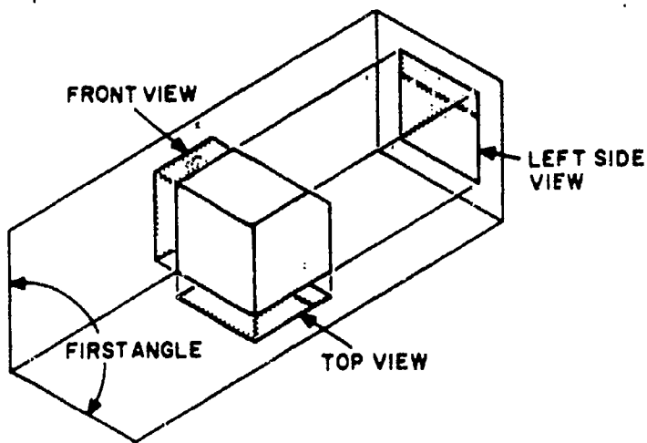
Figure 8-3.—First-angle projection of a cube.
