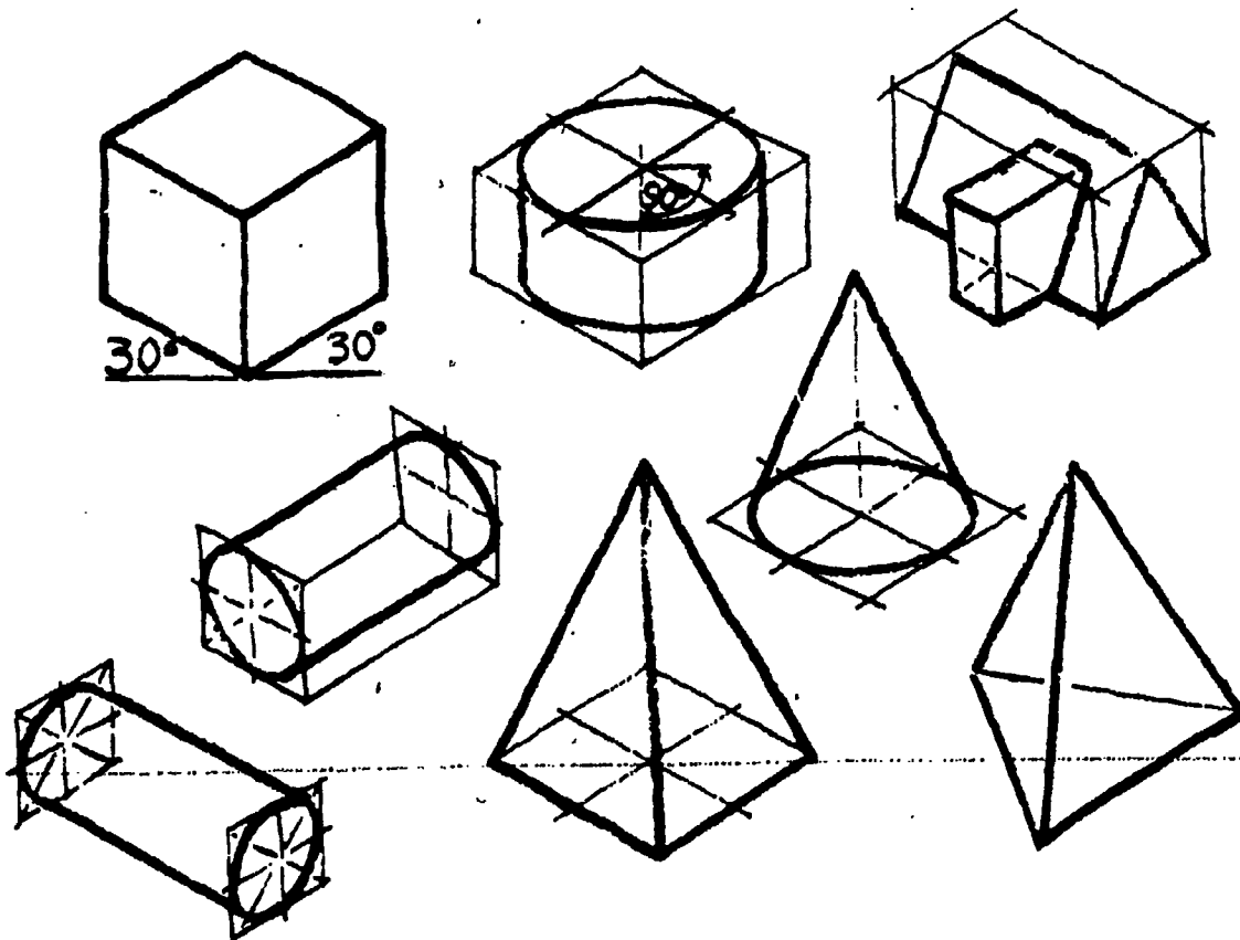
Figure 8-66.—Basic isometric forms.
