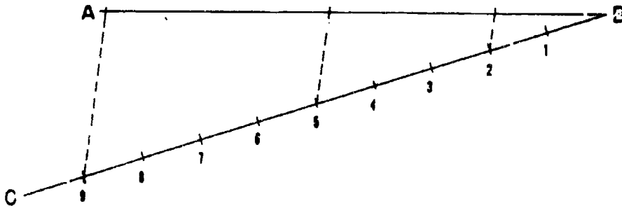
Figure 7-10.—Dividing a line into proportional parts.
