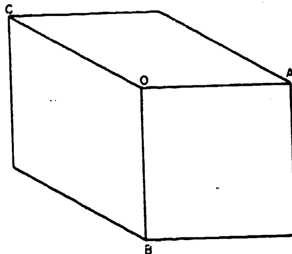
Figure 8-36.—Cavalier projection of a cube.
