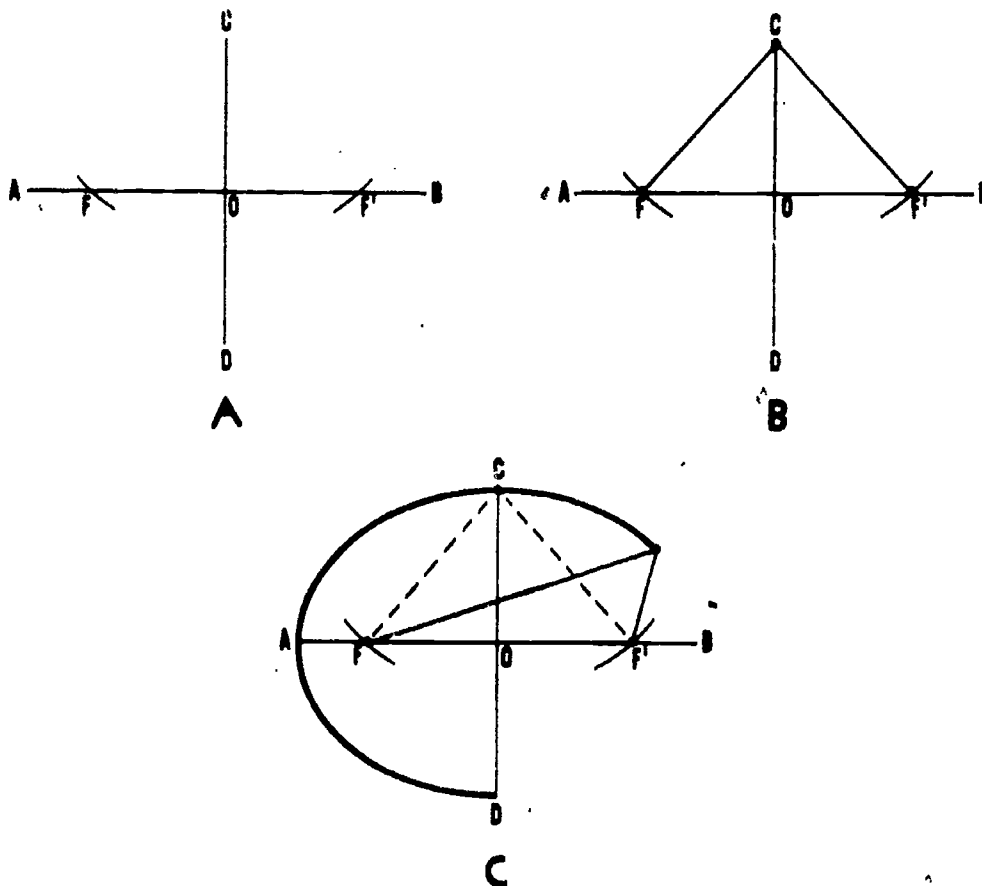
Figure 7-44.—Ellipse by pin-and-string method.
