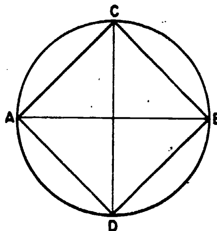
Figure 7-20.—Square in given circumscribed circle.
