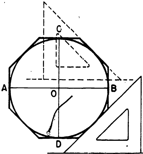
Figure 7-30.—Regular octagon around given inscribed circle.
