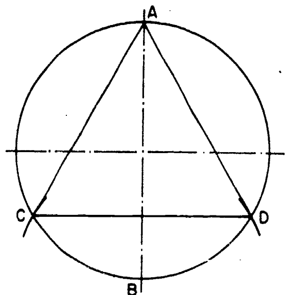
Figure 7-15.—Equilateral triangle in given circumscribed circle.
