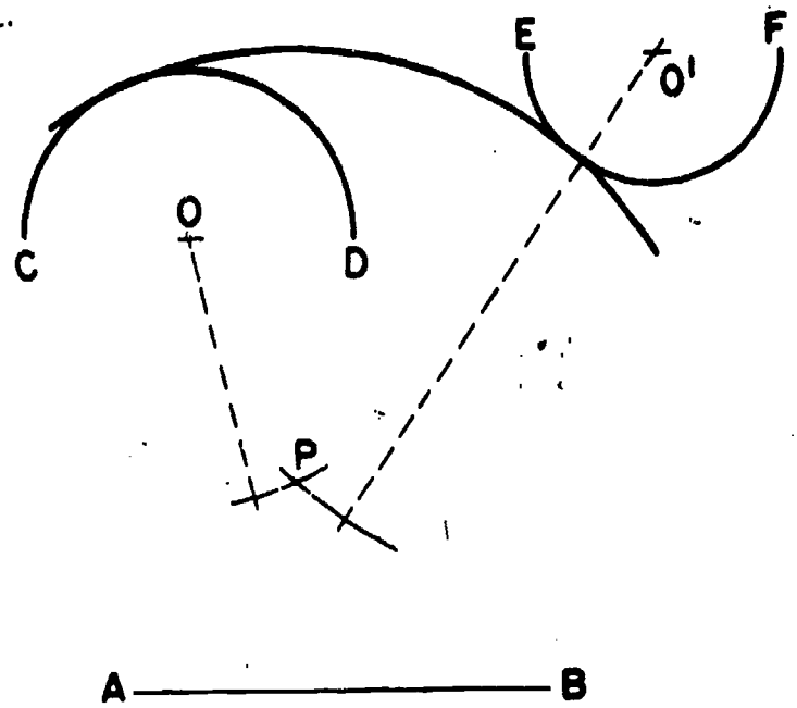
Figure 7-39.—Circular arc tangent to and enclosing one arc, and tangent to but not enclosing another.
