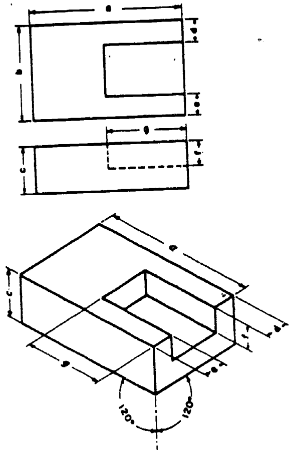
Figure 8-46.—Box construction.
