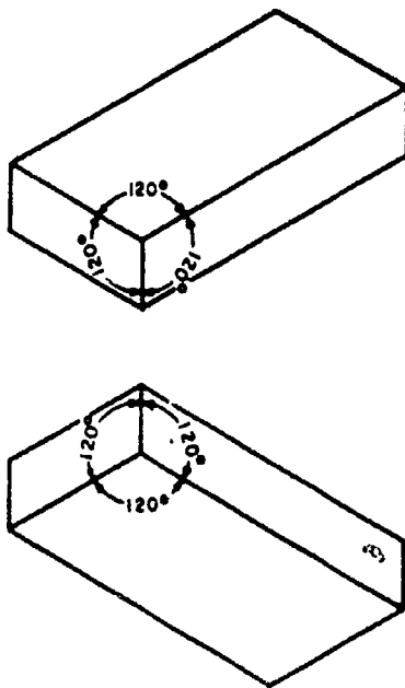
Figure 8-51.—Varying position of isometric axis varies view of the object.
