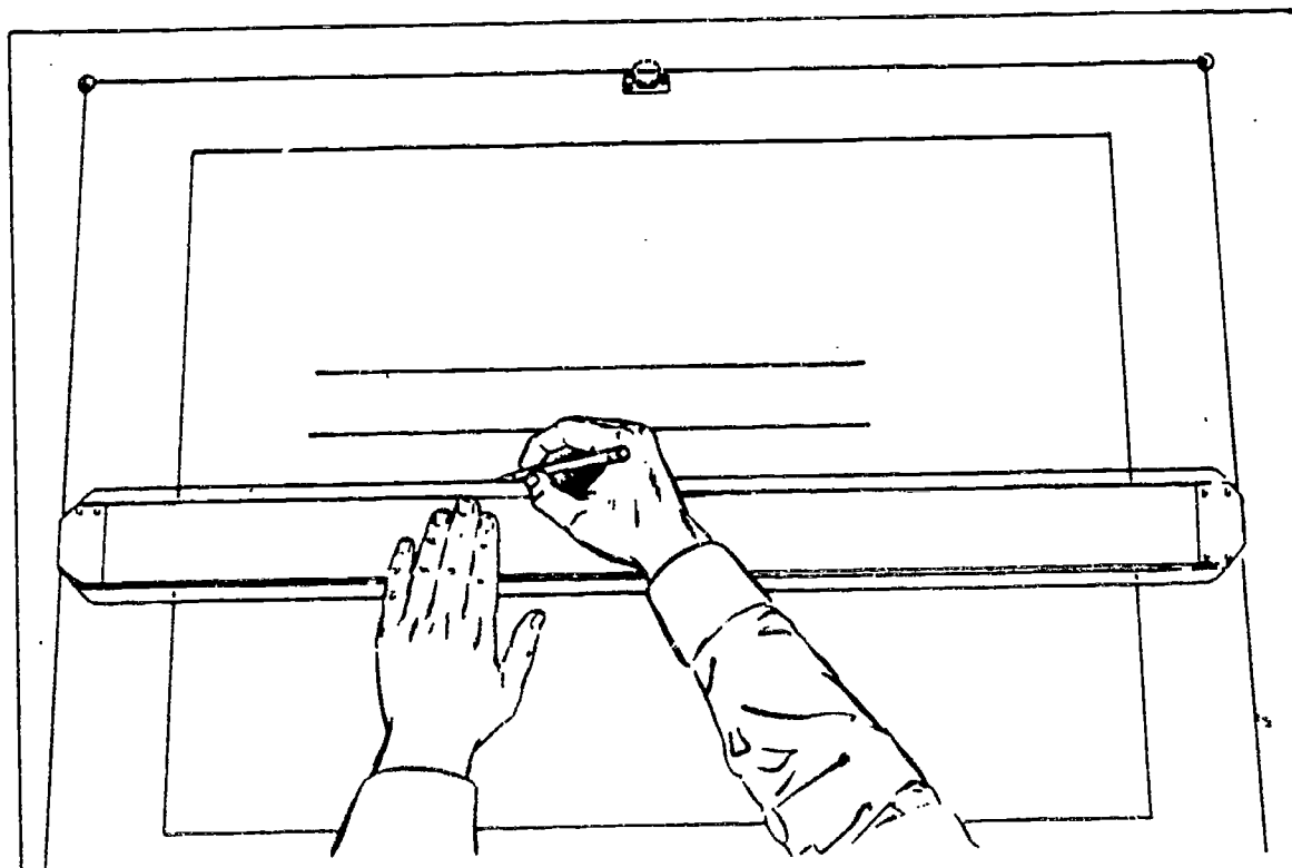
Figure 4-5.—Parallel straightedge.
