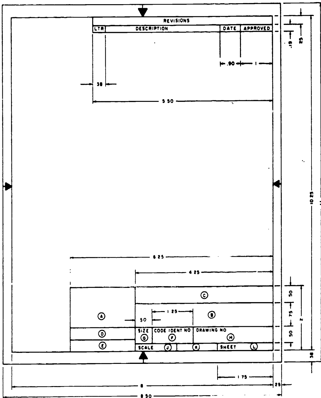
Figure 5-20.—Vertical format for "A" size drawings.
