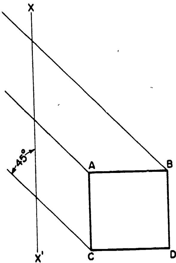
Figure 8-35.—Angle of projectors in a cavalier projection.
