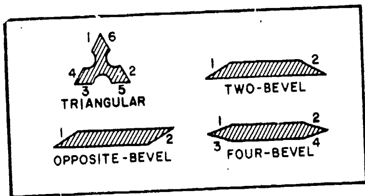
Figure 4-22.—Types of scales in cross section.
