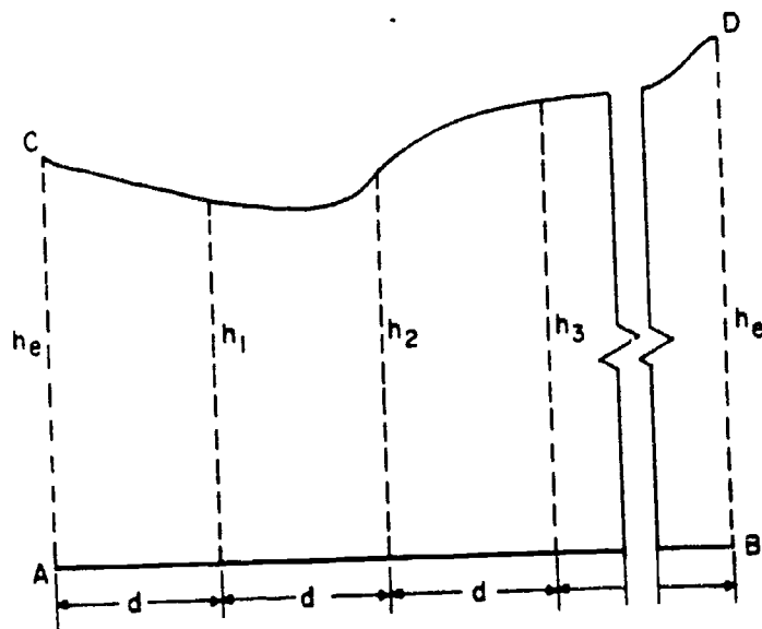
Figure 3-18.—Irregular areas by trapezoidal rule.
