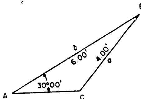
45.650 Figure 3-30.—Two ambiguous case triangles (solution of one will satisfy the other).
