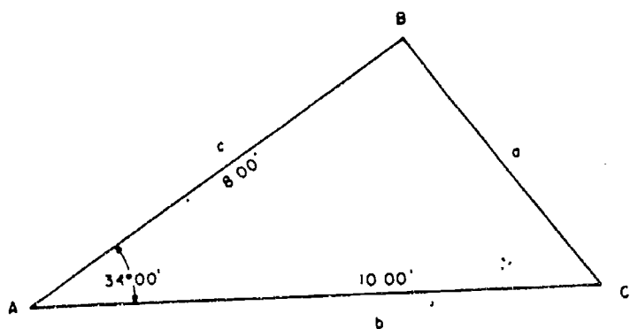
45.849 Figure 3-29.—Oblique triangle (law of tangents).
