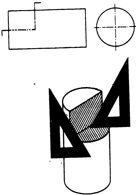
Figure 8-52.—Diagonal hatching in isometric.
