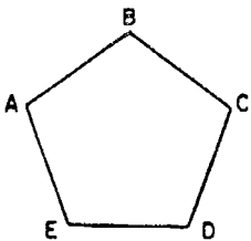
3. PENTAGON
