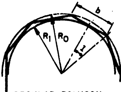
REGULAR POLYGON
