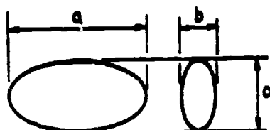
ELLIPSOID
