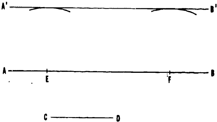
Figure 7-4.—Drawing a parallel line at a given distance from another line.
