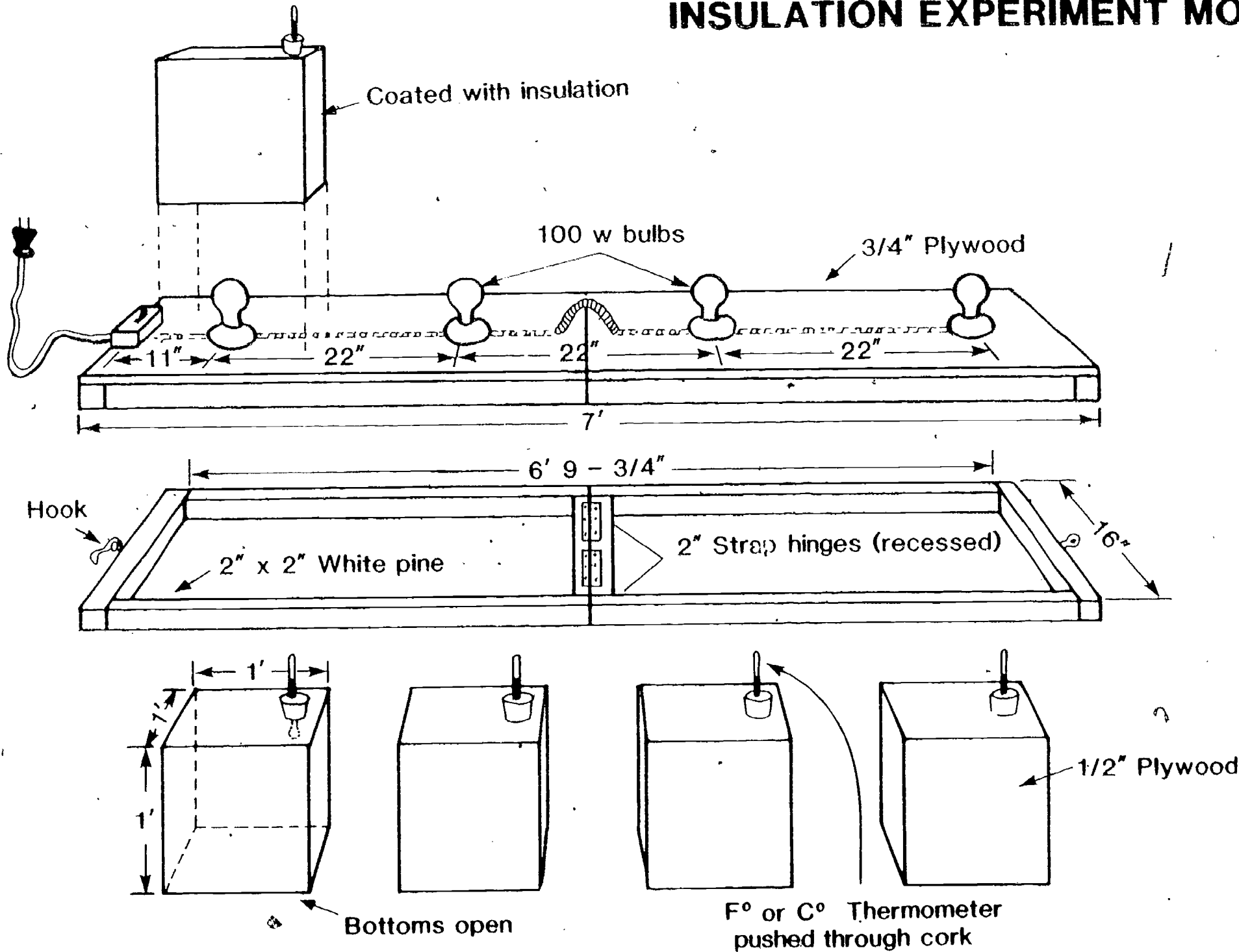
Each 1' cube is coated with different insulating materials
