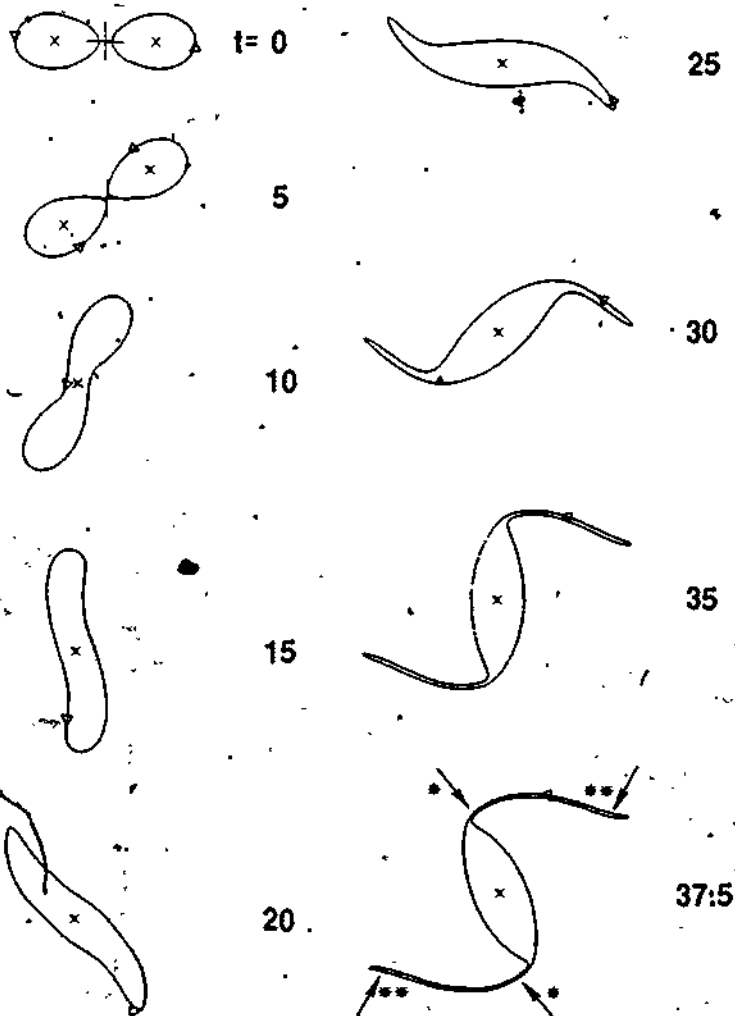
FIGURE 4.1 The evolution and merger of isolated vortex structures as predicted by contour dynamical techniques. [From E. A. Overman II and N. J. Zabusky, Phys. Fluids 25, 1297-1305 (1982).]
