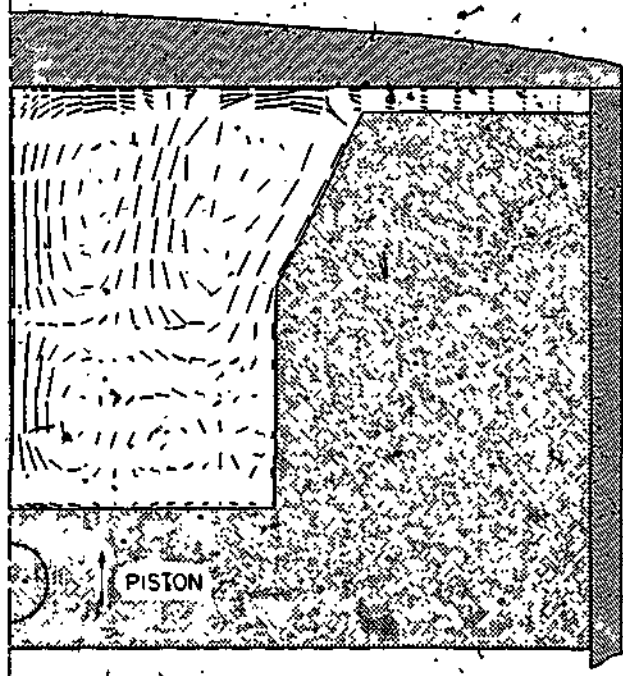
FIGURE 2.4 Velocity vectors computed in a direct-injection, stratified-charge engine at a position near top dead center. The combustion takes place in a swirling environment in a cup-like region machined into the piston. Several vortices are seen to develop in the cup. [From T. D. Butler, L. D. Cloutman, J. K. Dukowicz, and J. D. Ramshaw, Multidimensional numerical simulation of reactive flow in internal combustion engines, Prog. Energy Combust. Sci. , 7:293 (1981).]
