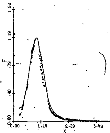
FIGURE 2.7 Monte Carlo simulation of a kinetic Ising model compared with x-ray and neutron diffraction measurements on an alloy of 60 percent gold and 40 percent platinum that has been heated and then quenched to 60 percent of its critical temperature. The abscissa is a reduced momentum transfer, and the ordinate is a reduced scattering intensity. (From M. H. Kalos, New York University.)
