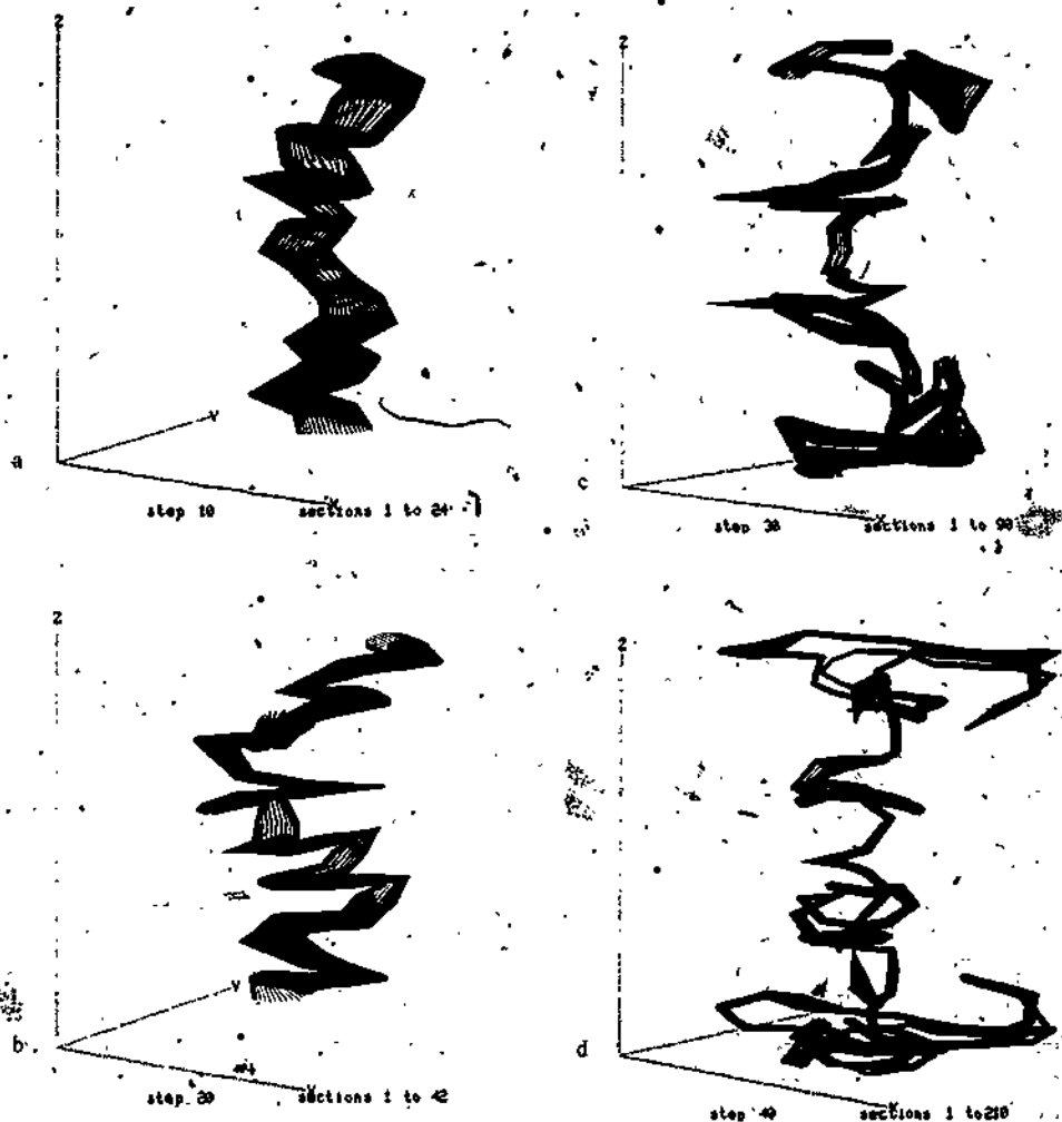
FIGURE 2.3. Successive stages in the stretching of a vortex tube in an inviscid periodic flow. Vortex stretching is the mechanism by which energy in a turbulent flow is transferred to ever smaller scales where it is eventually dissipated. a, step 10, time = 0.65; b, step 20, time = 0.88; c, step 30, time = 1.04; d, step 40, time = 1.21. [From A. J. Chorin, The evolution of a turbulent vortex, Commun. Math. Phys. 83, 526-527 (1982).]
