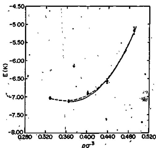
FIGURE 2.8 Energy of liquid helium as a function of density. The broken line and points with errors show results of the Monte Carlo quadrature of the many-body nonrelativistic Schrödinger equation. The solid line is a fit to the experimental data. (From M. H. Kalos, New York University.)
