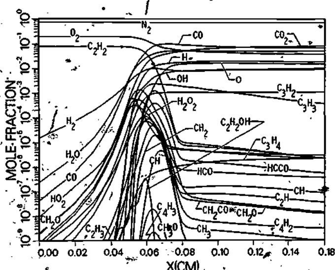
FIGURE 2.5 Species mole fraction profiles showing the internal structure of an atmospheric-pressure stoichiometric acetylene-air flame. [From J. A. Miller and R. J. Kee, Sandia National Laboratories.]
