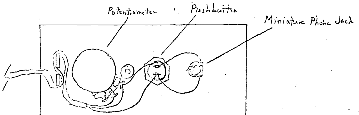
Game Paddle, Inside Front View
