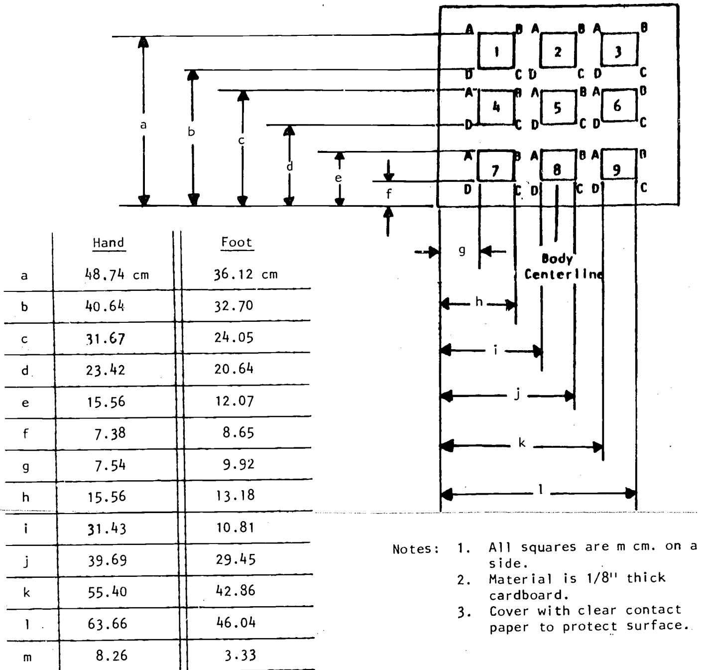
Figure 2. Layout of testing sheet used for range measurement of hand and foot. The foot sheet may also be used for small children with limited reach.
