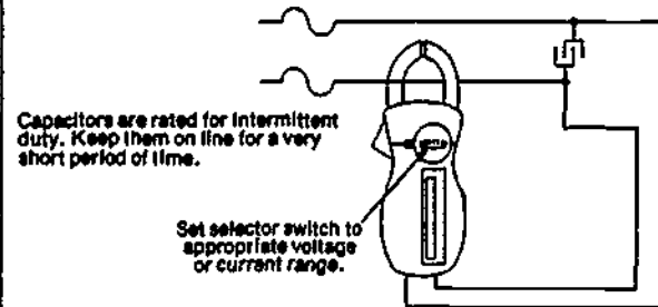
Figure 6 - Checking AC Electrolytic Capacitors If there is no current indication, capacitor is open. Shorted capacitor will blow fuse when line voltage is applied.
