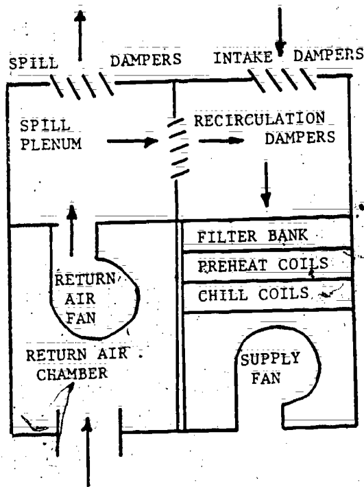
Figure 2.14 Typical HVAC system configuration of high-rise buildings 1/
