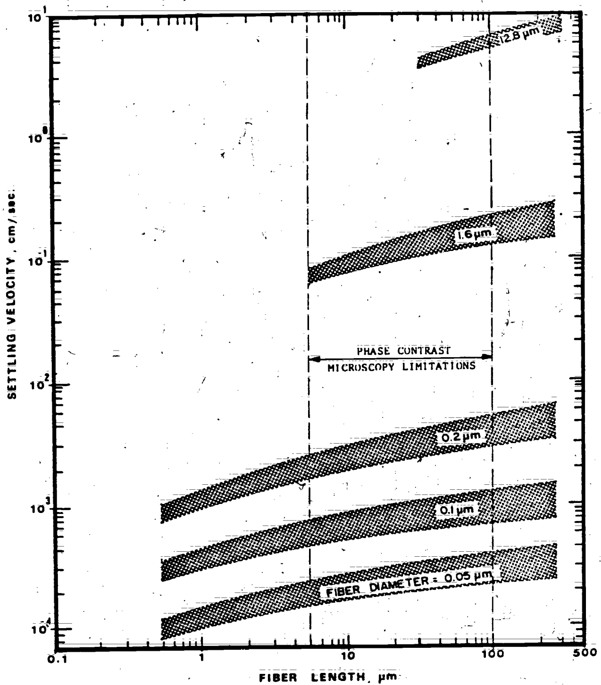
Figure 1.2 Theoretical settling velocities of asbestos fibers 1/ 1/ Figure taken from reference [5].
