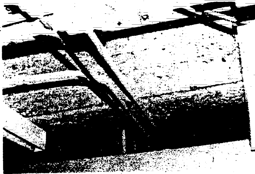
Figure 2.11 Damage to fireproofing on structural steel due to electrical system modifications
