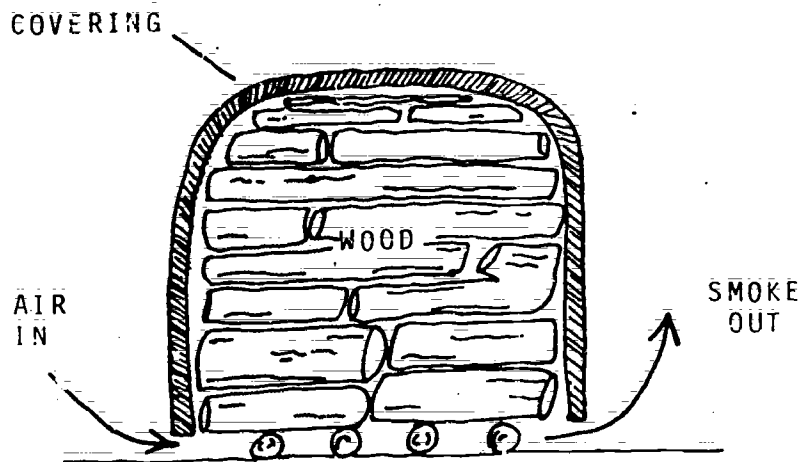
BASIC DESIGN FEATURES FOR A CHARCOAL KILN
