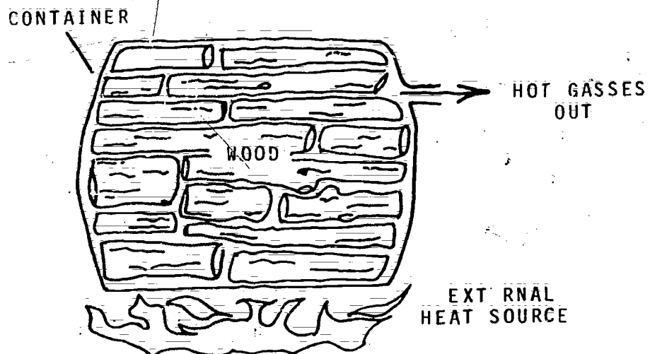
BASIC DESIGN FEATURES FOR A CHARCOAL RETORT
