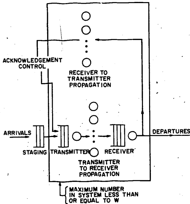
Figure 1. Queuing Network Block Diagram
