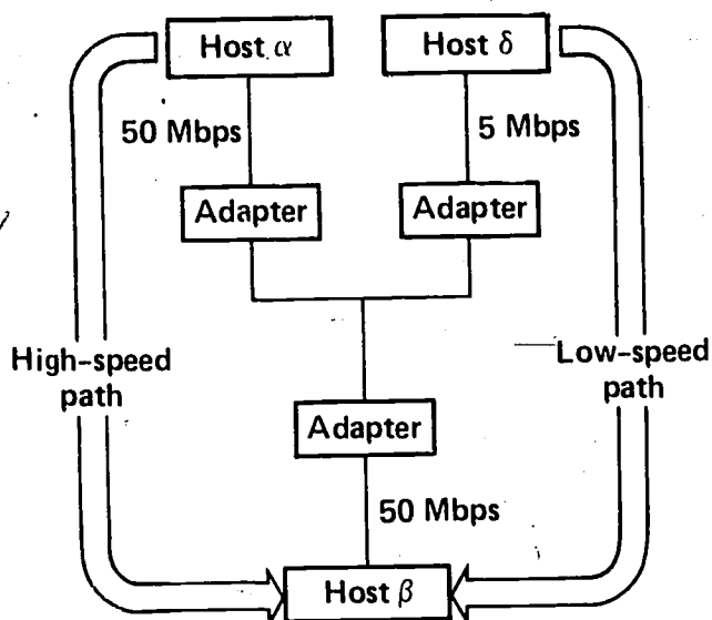
Figure 19. Uni-directional message switch.
