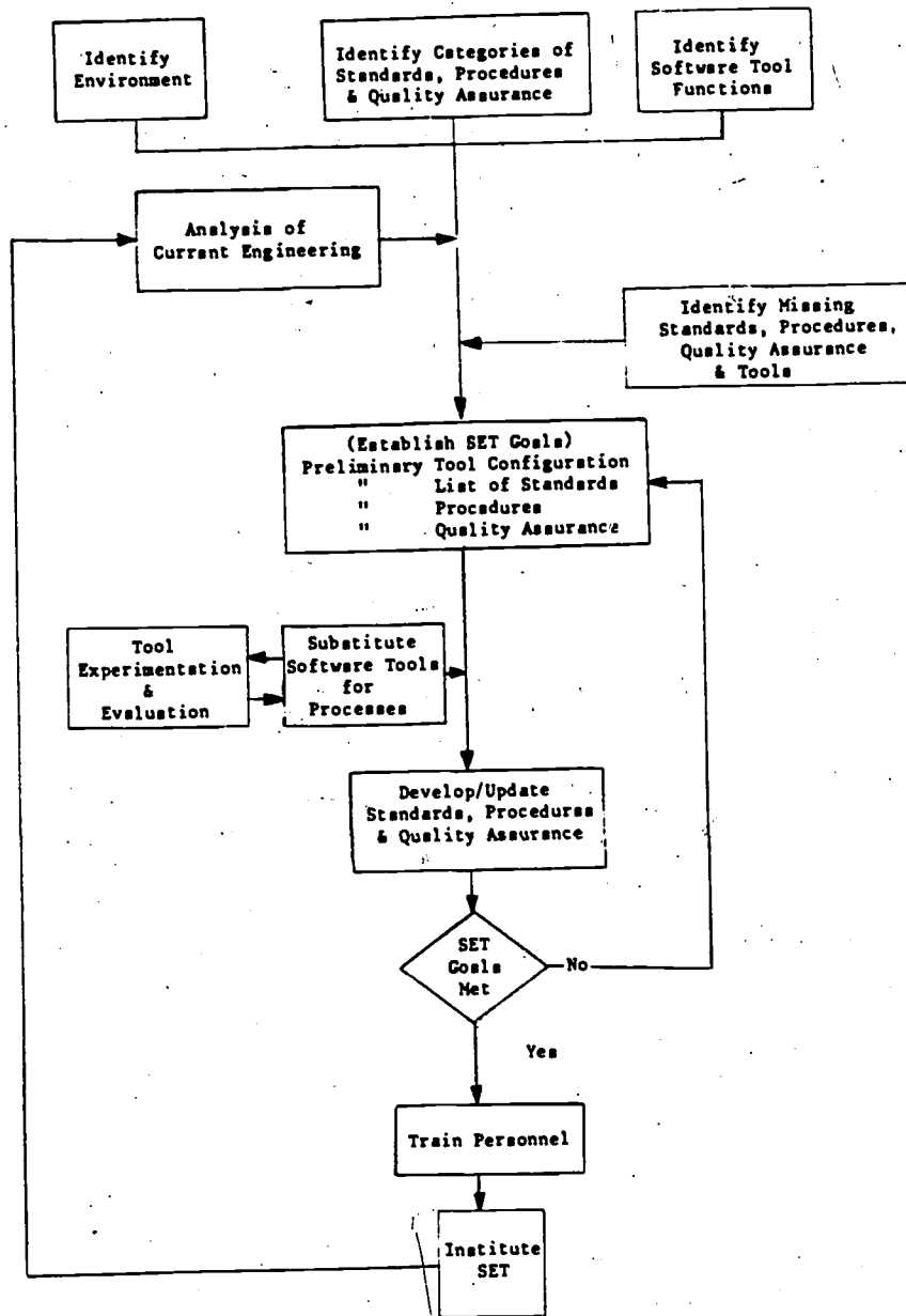
Figure 3: Model for Developing a SET
