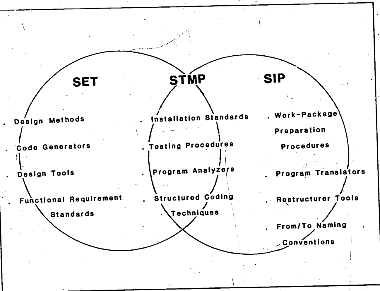
Figure 6. Example of Typical SET and SIP Interrelationship under a STMP
