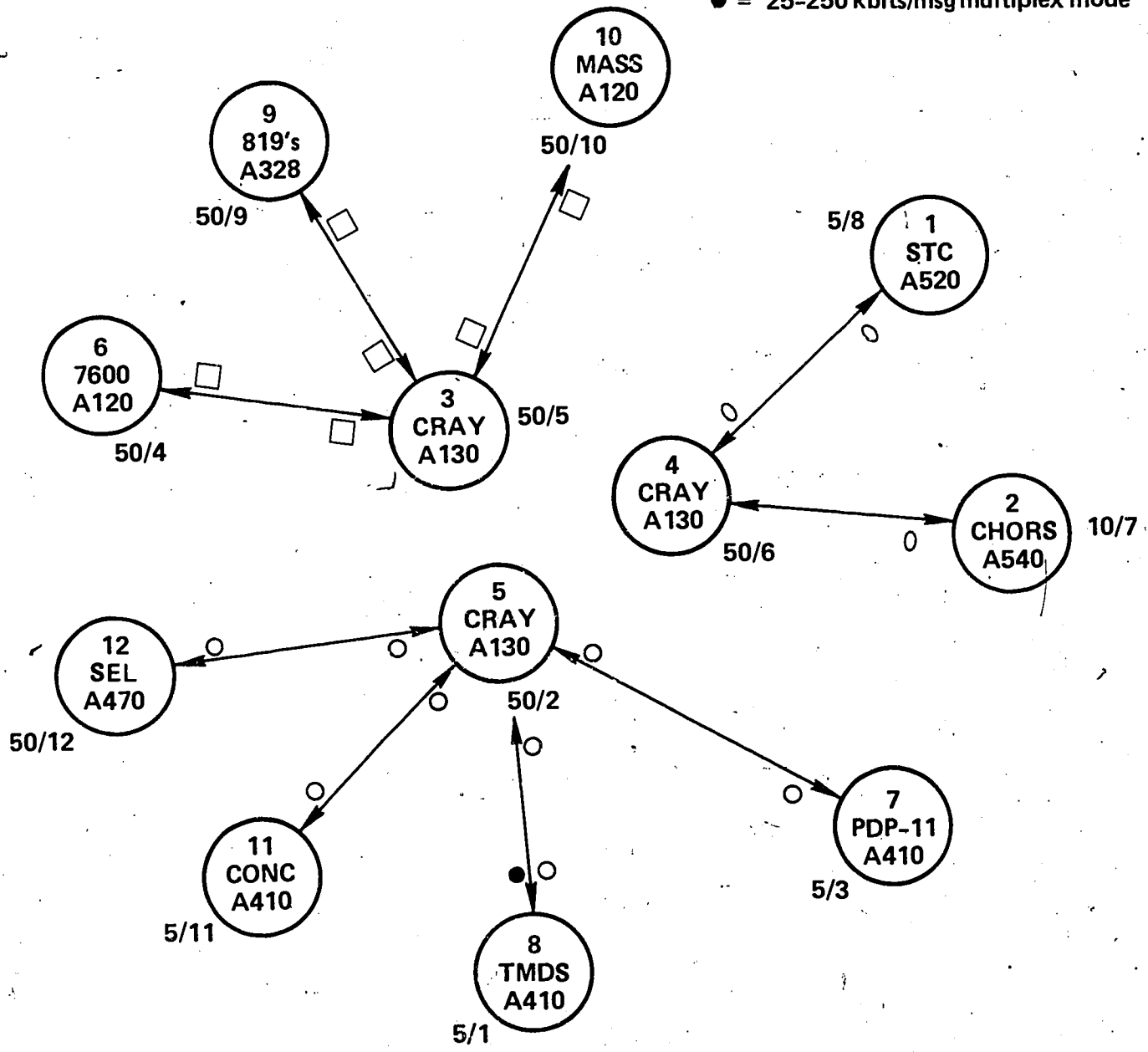
Figure 4. An older, single CRAY version of CRAYNET showing traffic patterns and message sizes.
