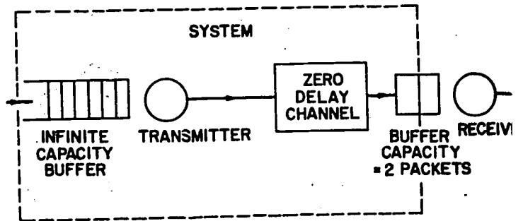
Figure 4. Queuing Network Block Diagram for W=2
