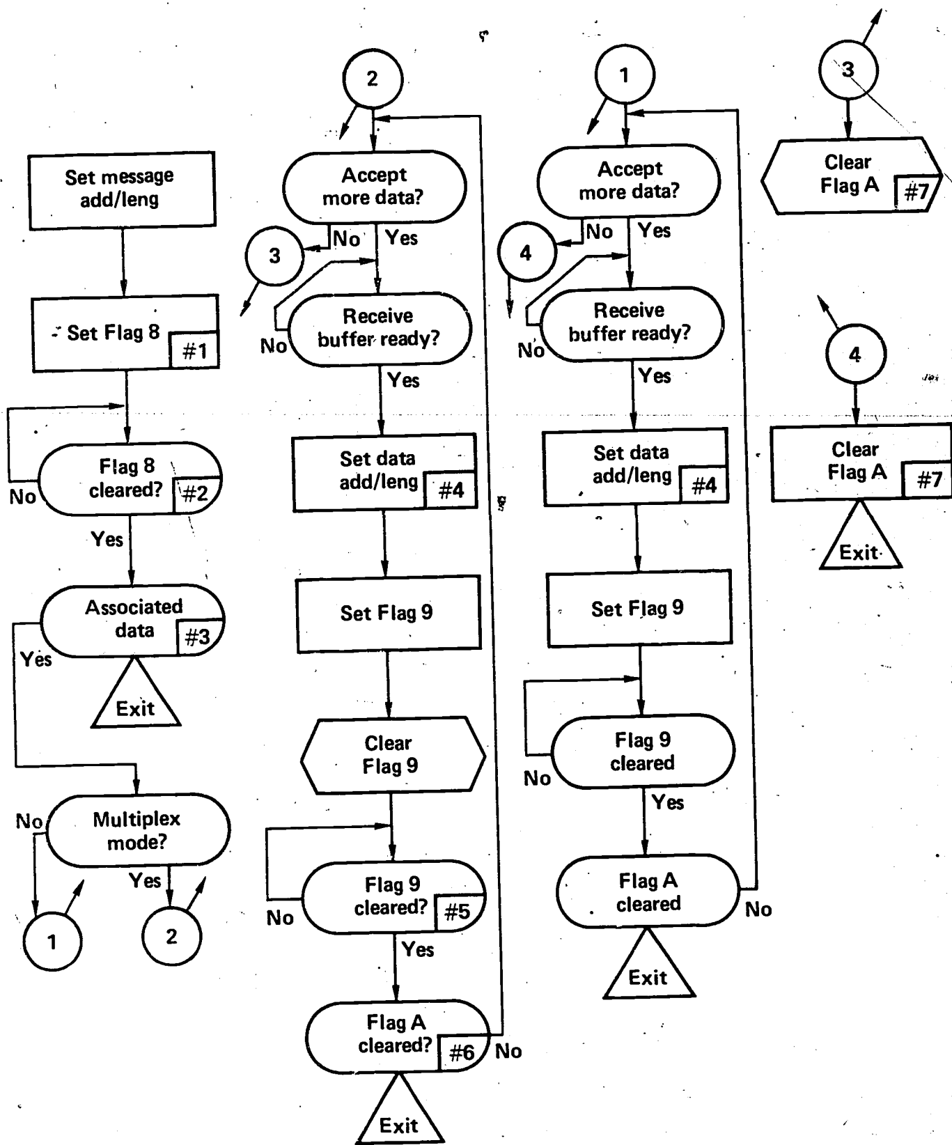
Figure 18b. The receiver protocol.
