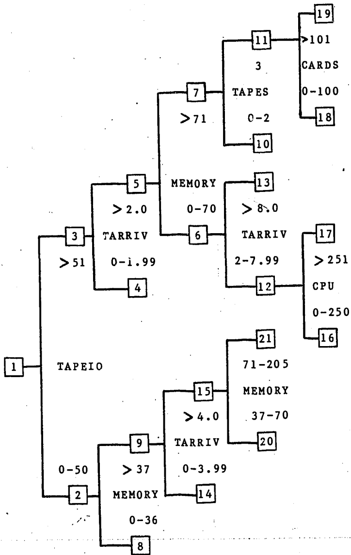
Figure 3. Augmented AID Skeleton Tree for Data Set 1
