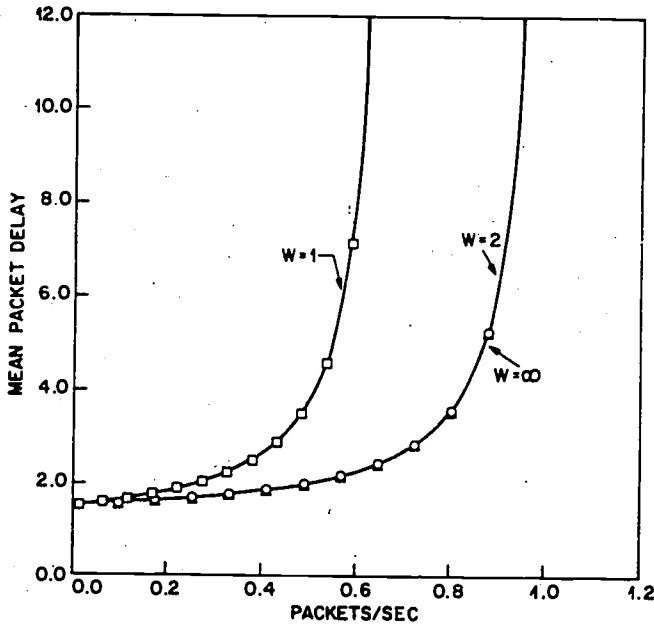
Figure 5. Mean Packet Delay vs Arrival Rate
