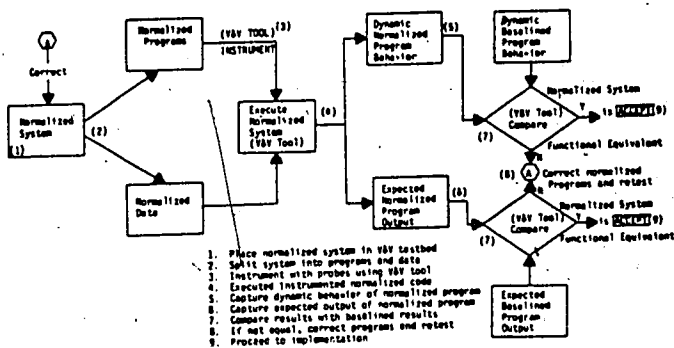
Exhibit 11. System Test Step in Conversion Phase
