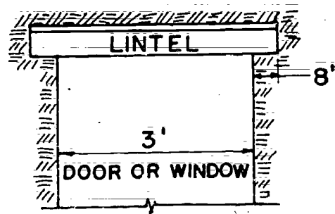
Figure 95. Wood lintel.
