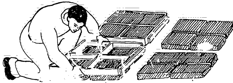
Figure 41. Lifting the forms from freshly made blocks.
