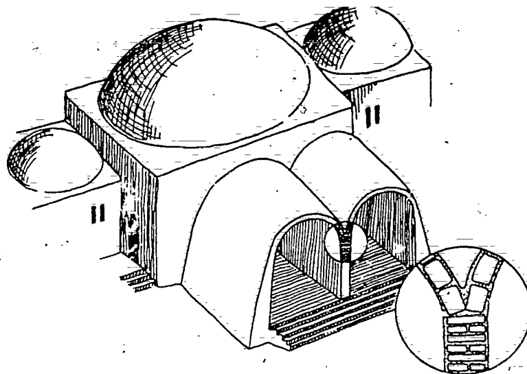
Figure 88. This style of earth dome and vault construction was used in a reconstruction program at New Gourná, Egypt.
