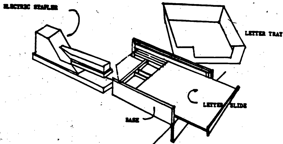
Figure 15.1. Electric stapler jig. (Designed by Alice Udvari)
