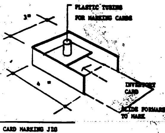
CARD MARKING JIG
