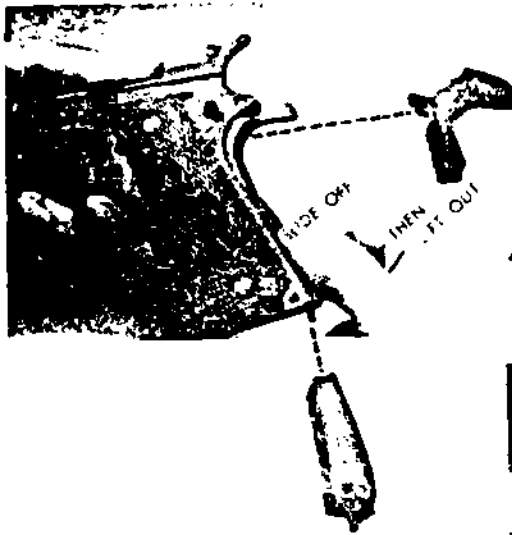
5 HAMMER, HAMMER STRUT, AND PINS
