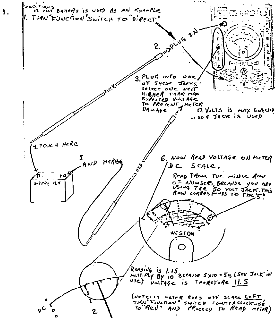
Figure 4-13. Measuring voltage, 12 volt battery.
